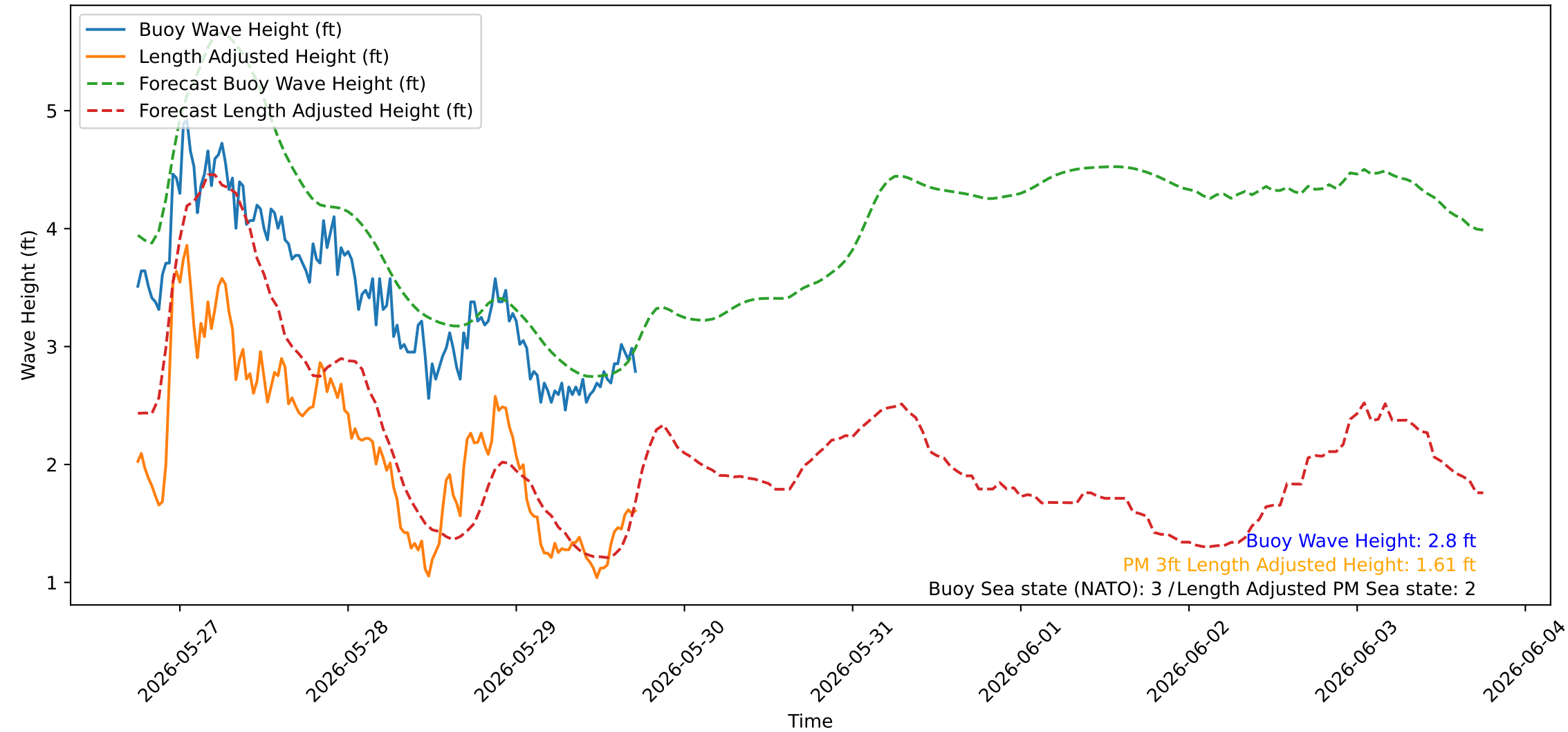
Wave Heights over Time for Green Beach at 2026-05-29 18:01:04
