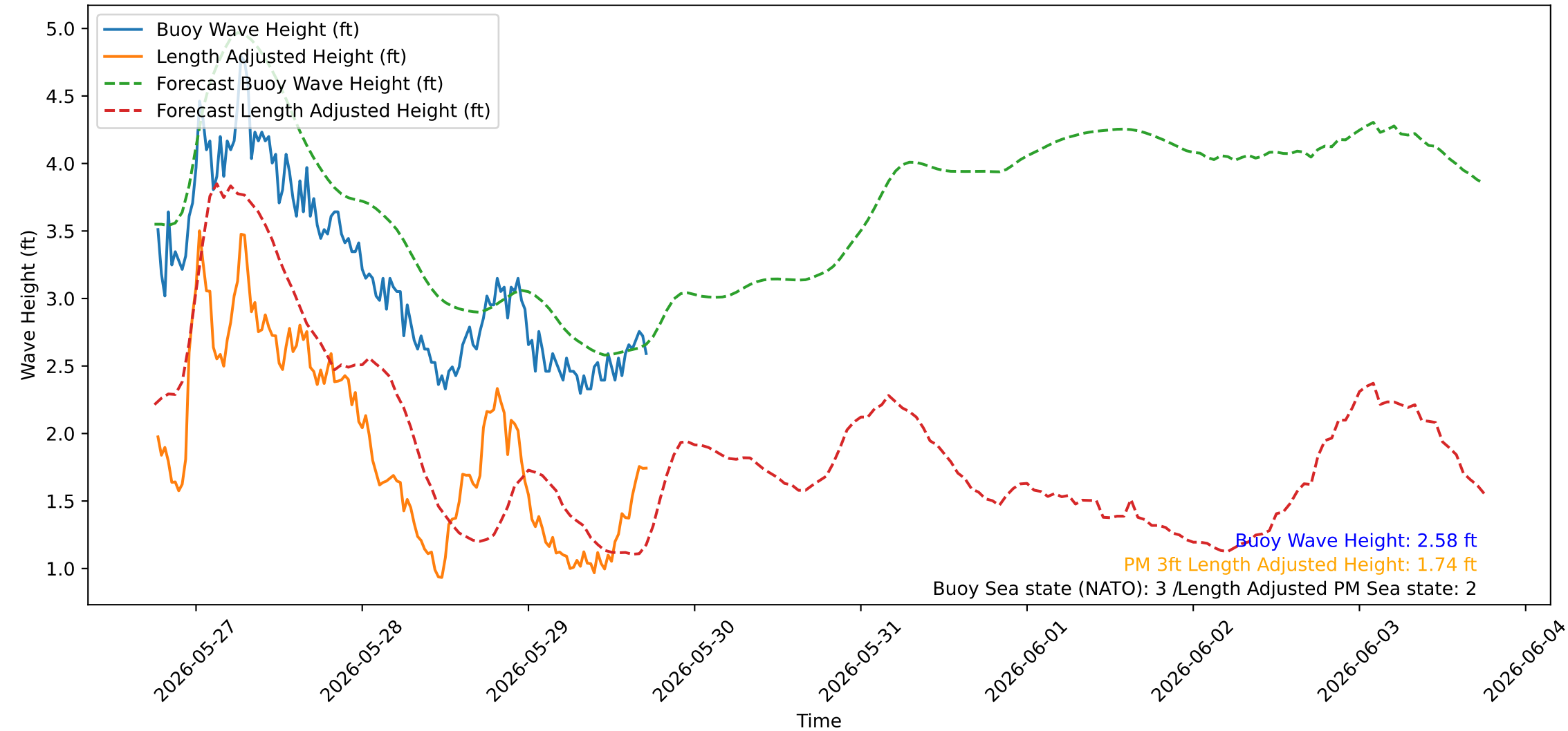
Wave Heights over Time for Red Beach at 2026-05-29 18:00:41
