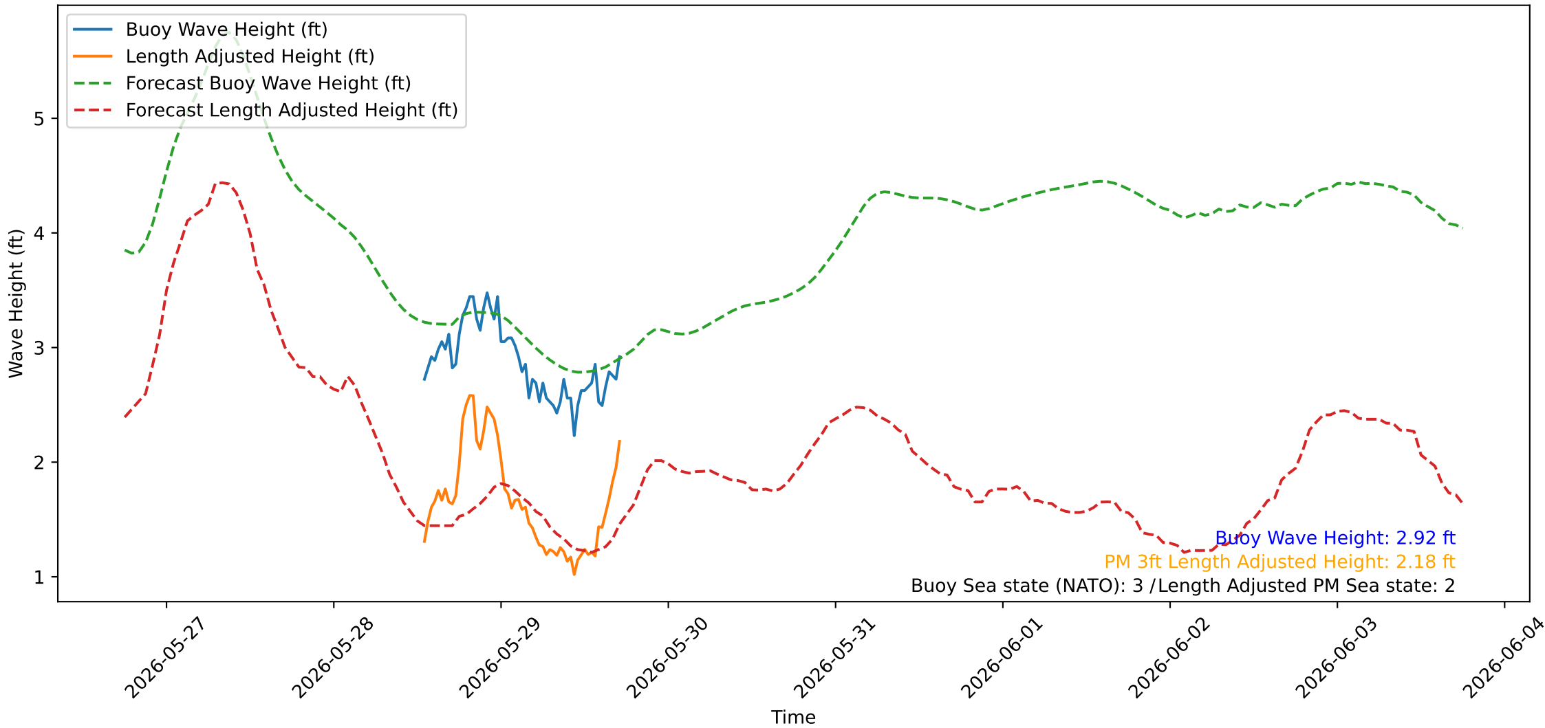
Wave Heights over Time for Oceanside Harbor at 2026-05-29 18:00:22
