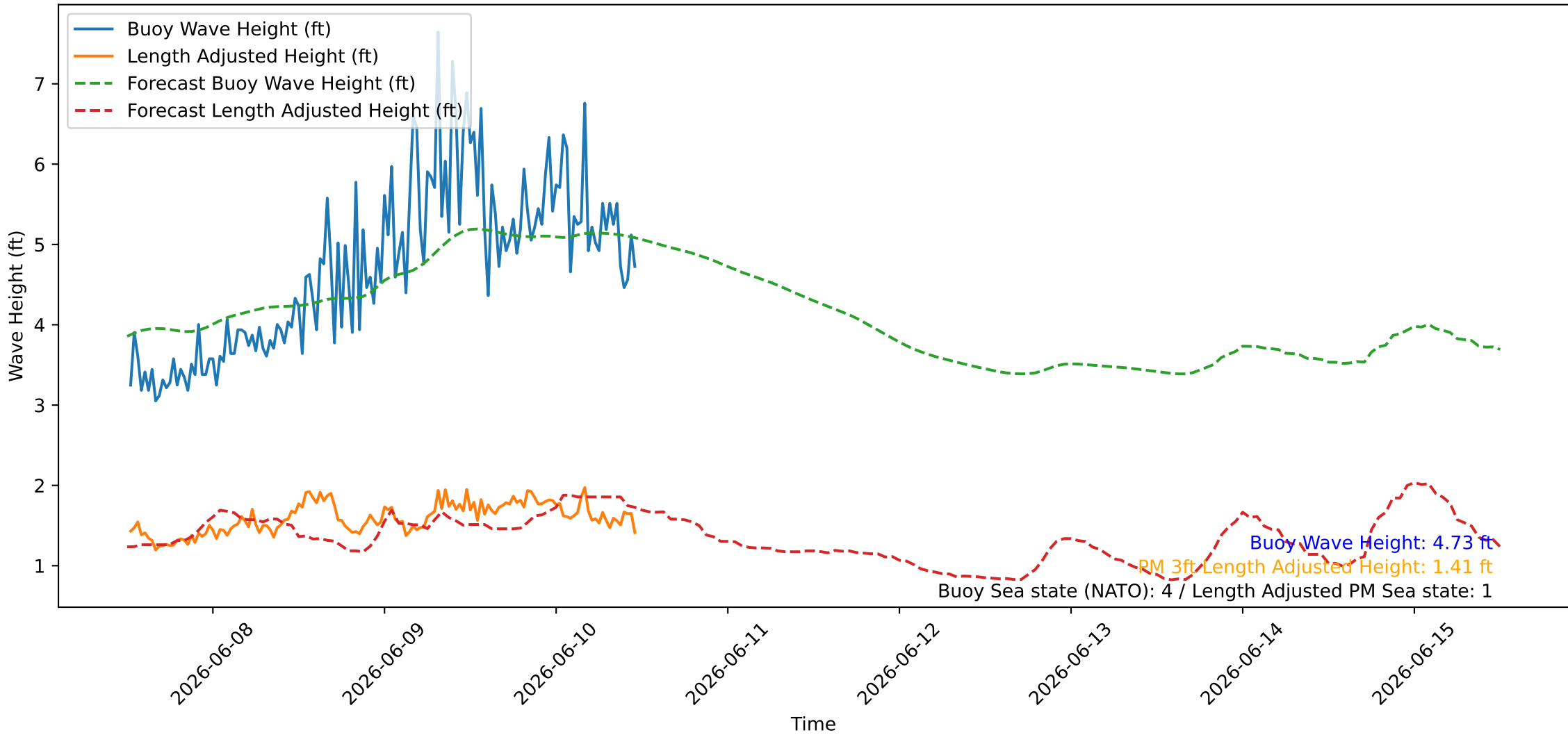
Wave Heights over Time for Red Beach at 2026-06-10 12:20:48
