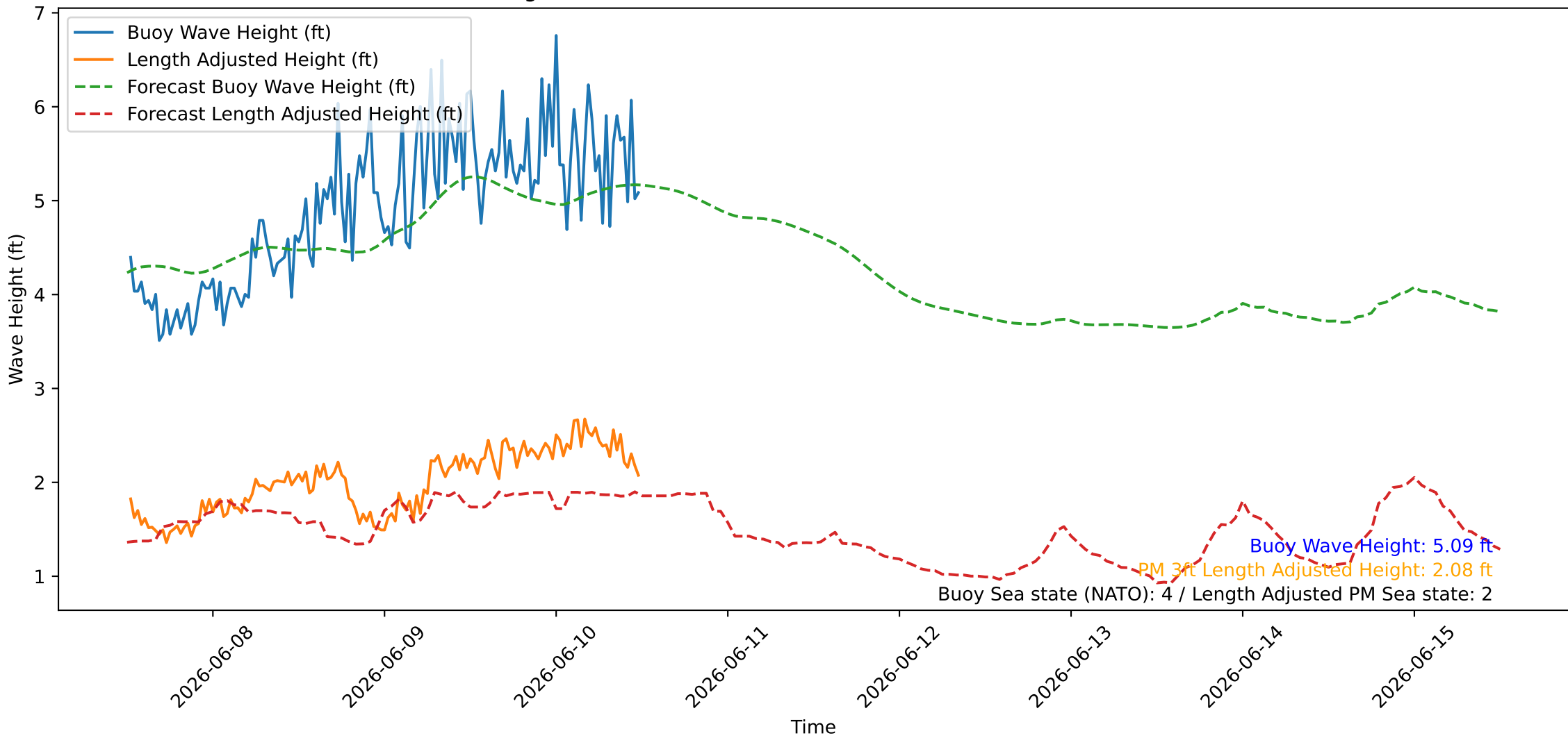
Wave Heights over Time for Oceanside Harbor at 2026-06-10 12:20:26
