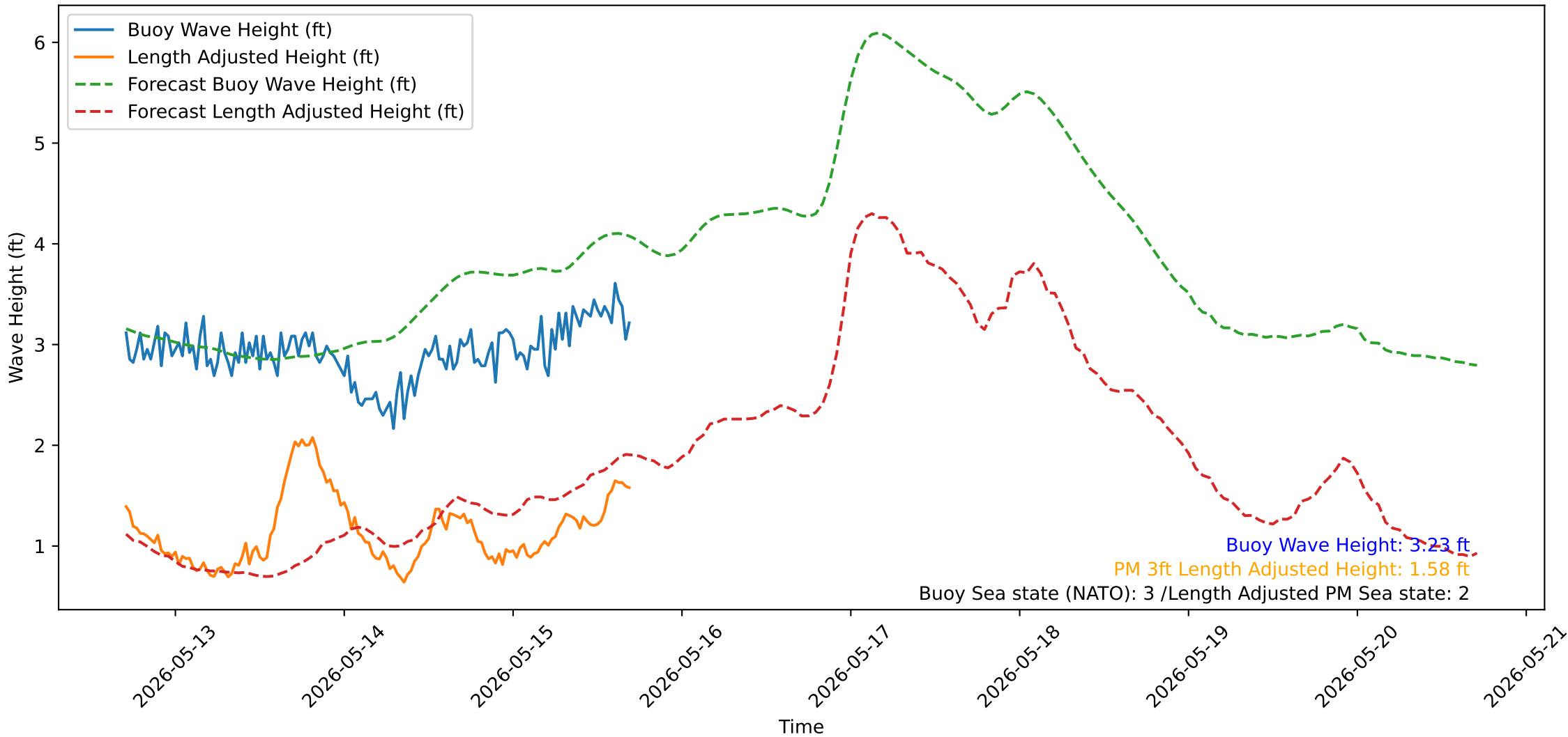
Wave Heights over Time for Oceanside Harbor at 2026-05-15 17:10:32
