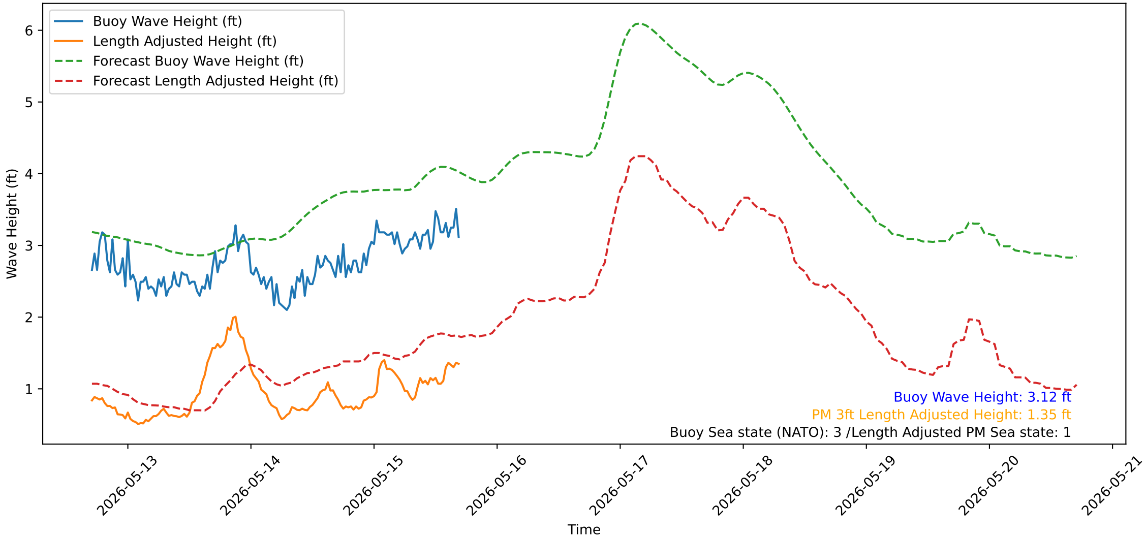
Wave Heights over Time for Green Beach at 2026-05-15 17:11:14
