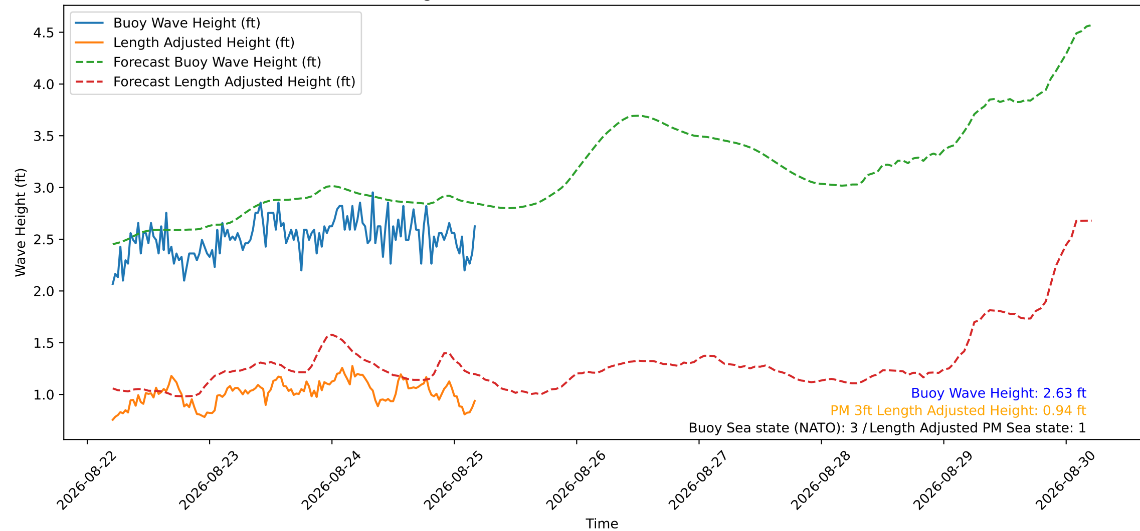
Wave Heights over Time for Red Beach at 2026-08-25 04:40:49
