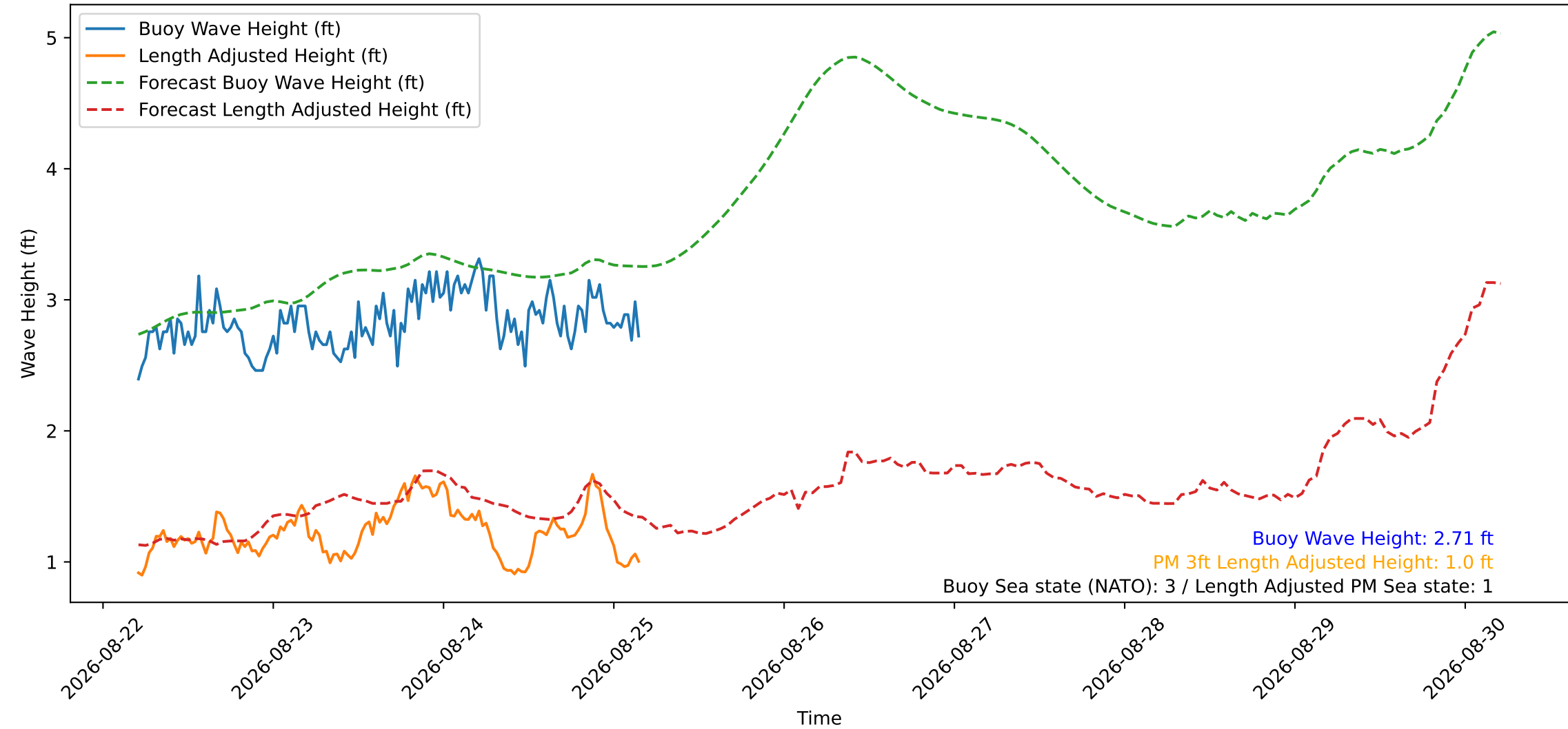
Wave Heights over Time for Green Beach at 2026-08-25 04:41:12
