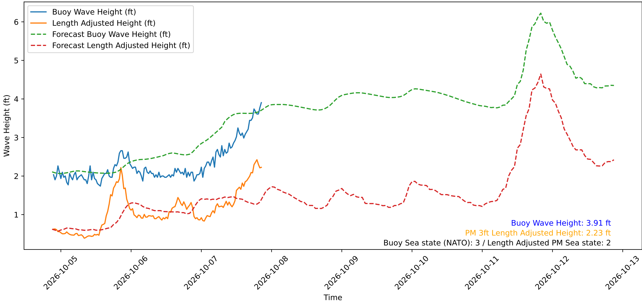
Wave Heights over Time for Red Beach at 2026-10-07 21:20:52
