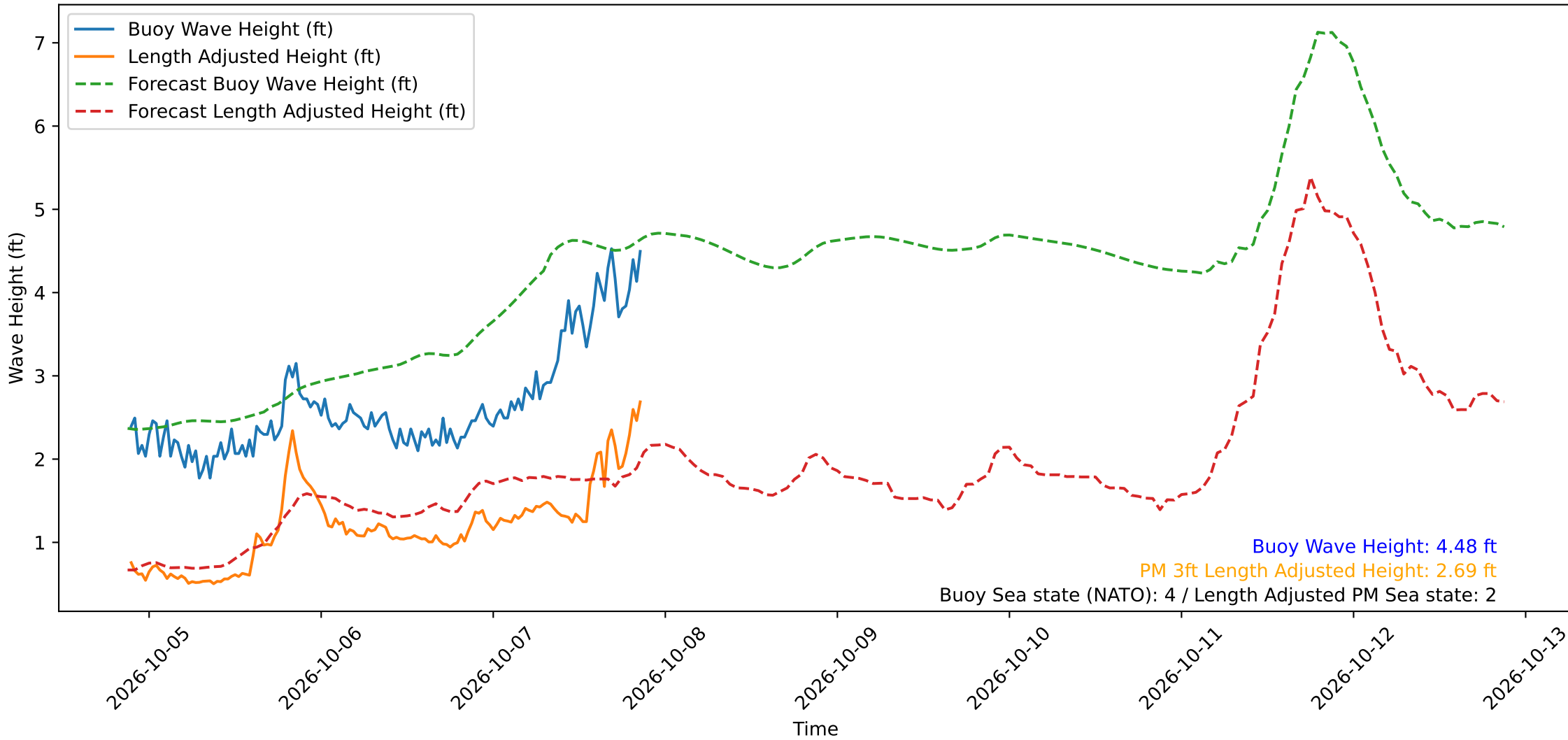
Wave Heights over Time for Green Beach at 2026-10-07 21:21:16
