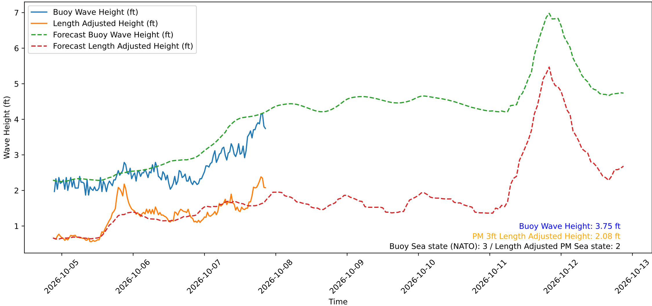
Wave Heights over Time for Oceanside Harbor at 2026-10-07 21:20:30
