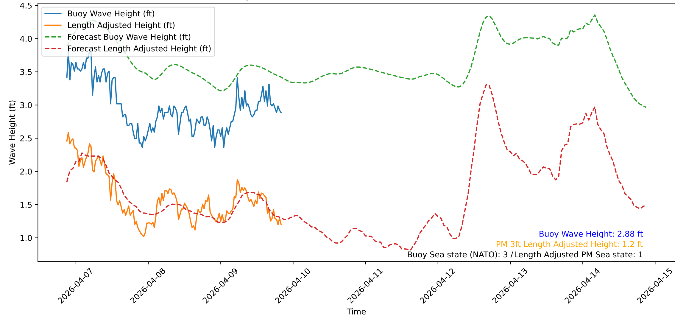
Wave Heights over Time for Green Beach at 2026-04-09 21:01:11
