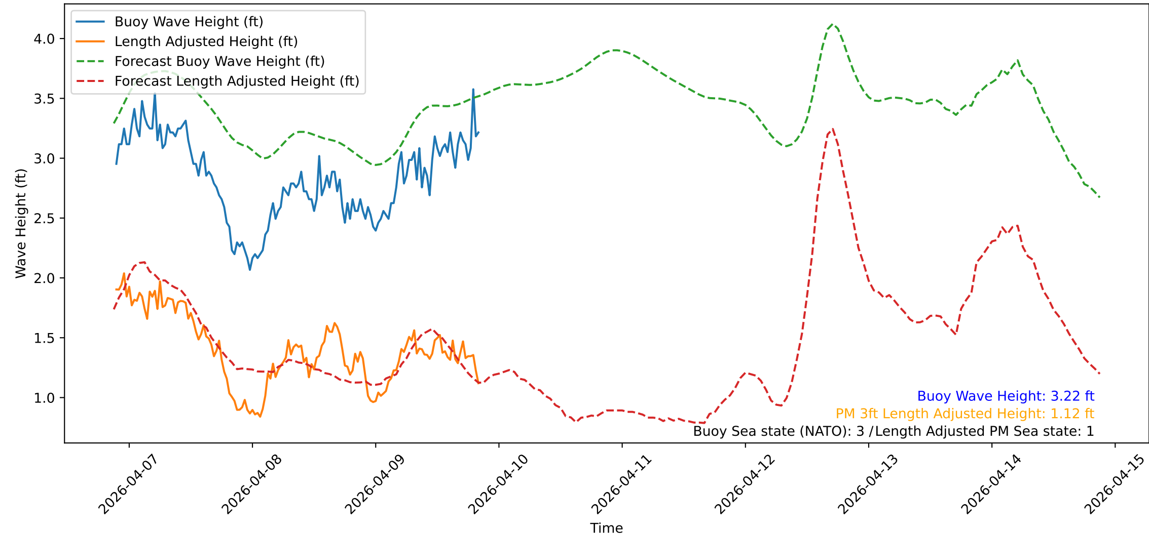
Wave Heights over Time for Red Beach at 2026-04-09 21:00:47
