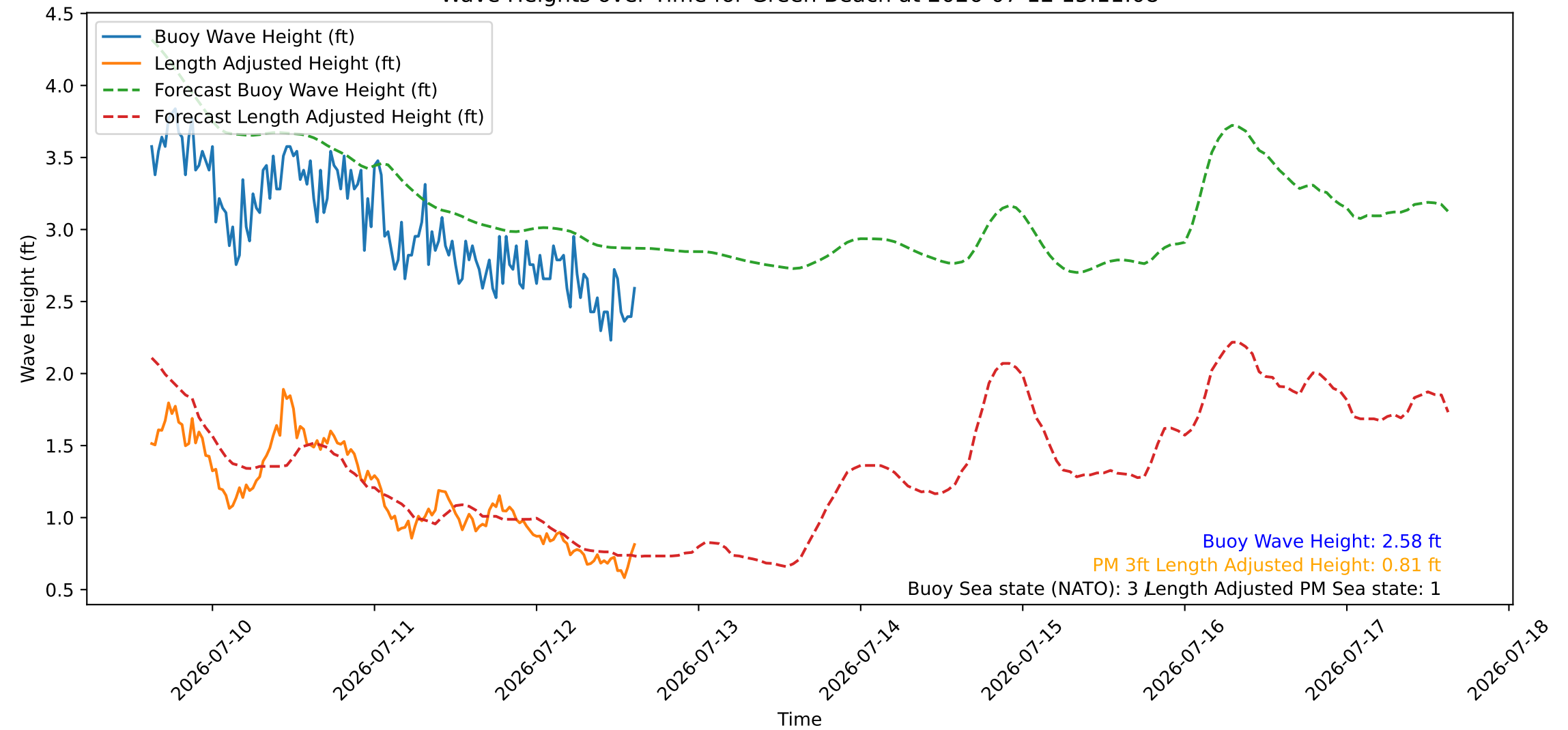
Wave Heights over Time for Green Beach at 2026-07-12 15:11:08
