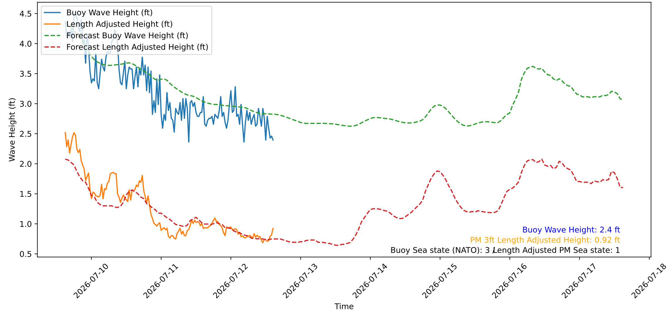
Wave Heights over Time for Oceanside Harbor at 2026-07-12 15:10:26
