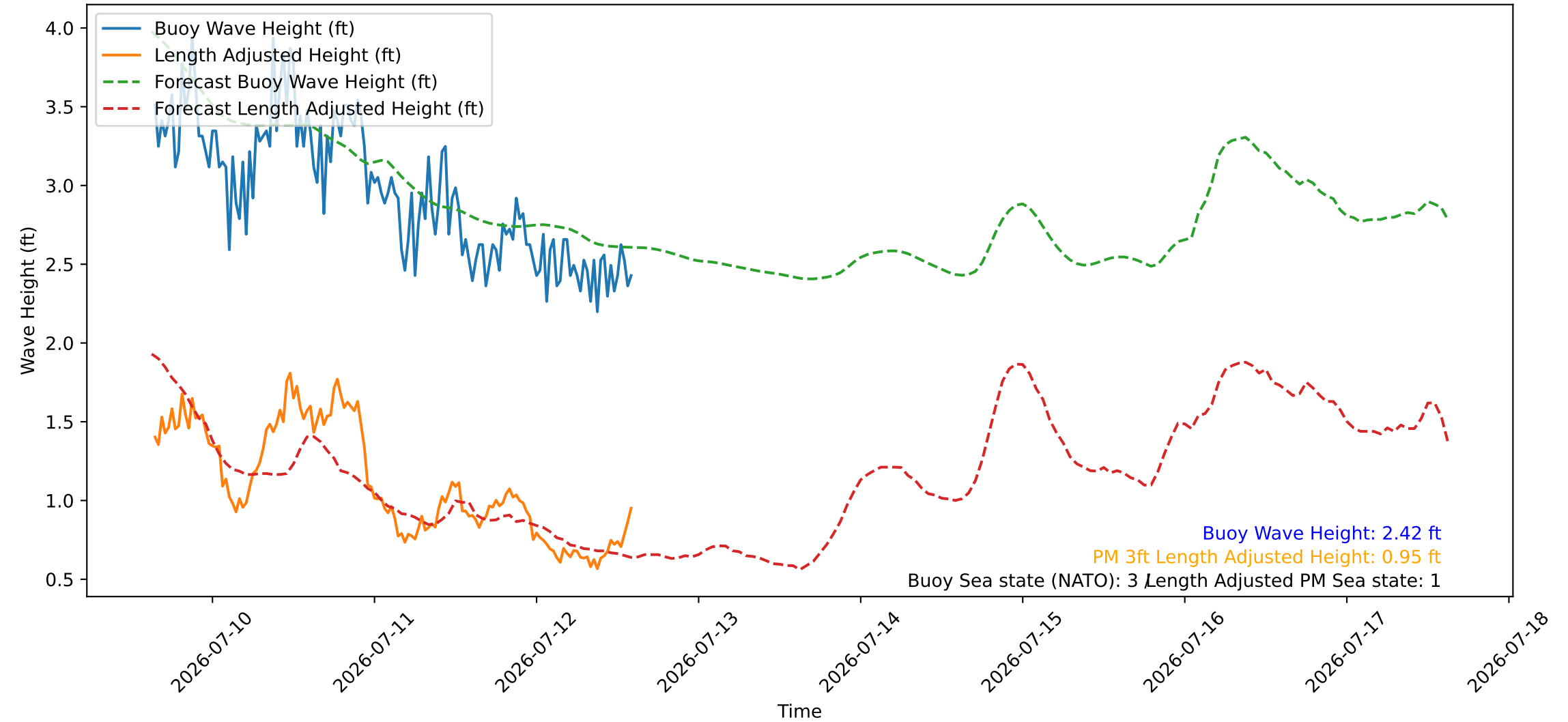
Wave Heights over Time for Red Beach at 2026-07-12 15:10:46
