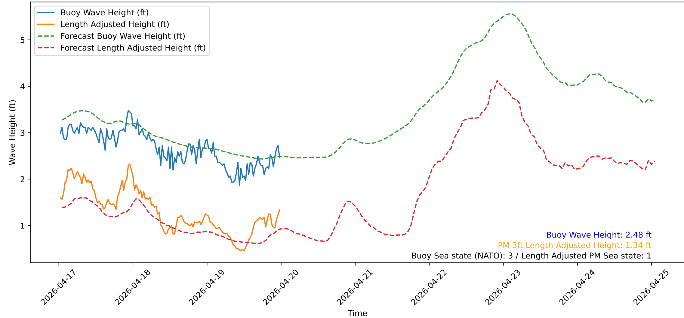
Wave Heights over Time for Green Beach at 2026-04-20 00:31:13
