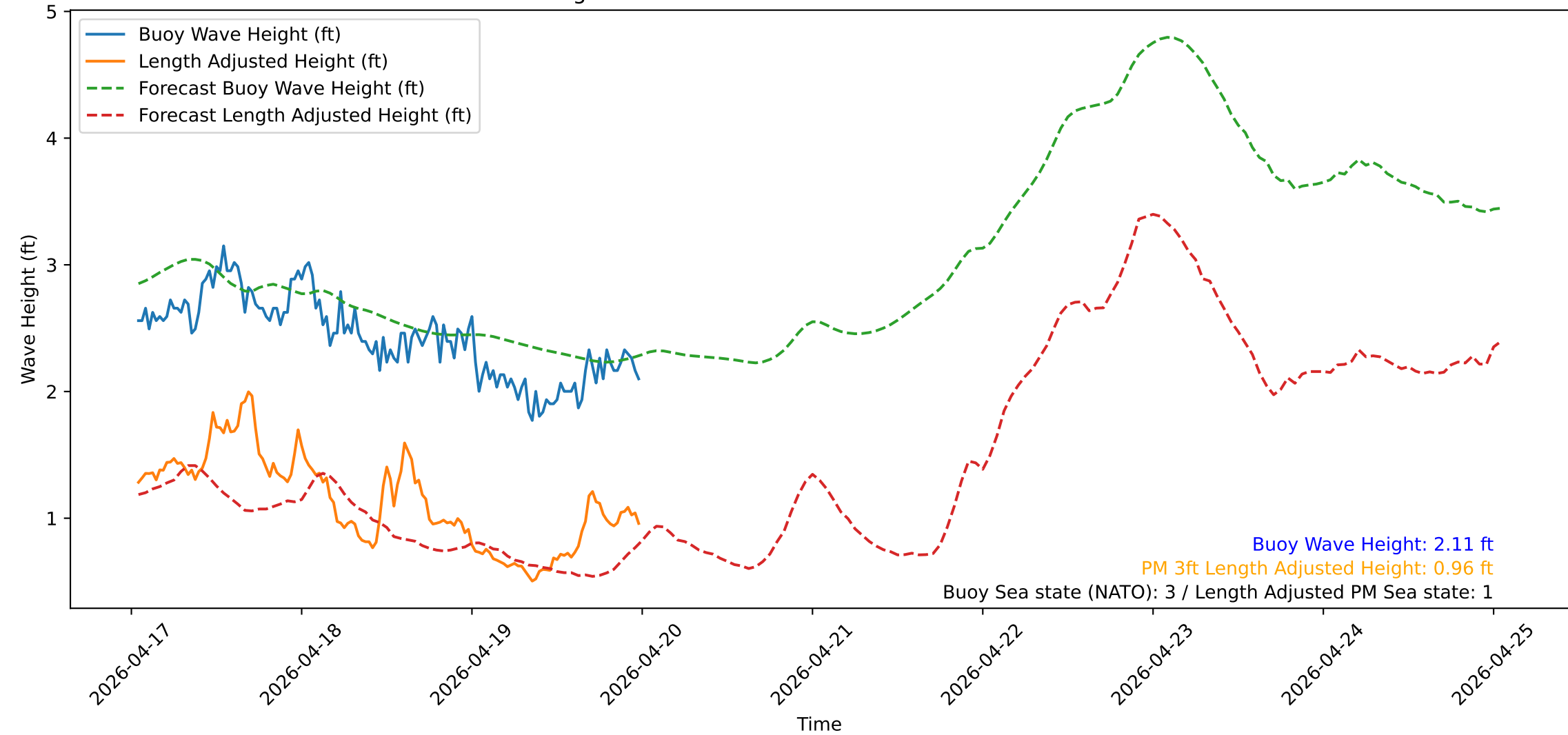
Wave Heights over Time for Red Beach at 2026-04-20 00:30:50
