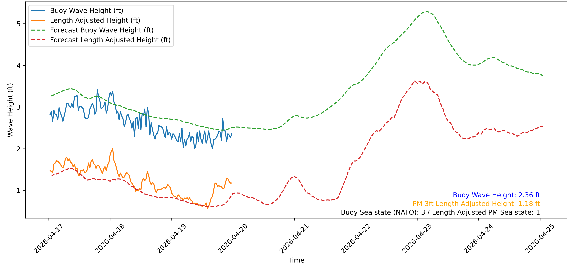
Wave Heights over Time for Oceanside Harbor at 2026-04-20 00:30:31
