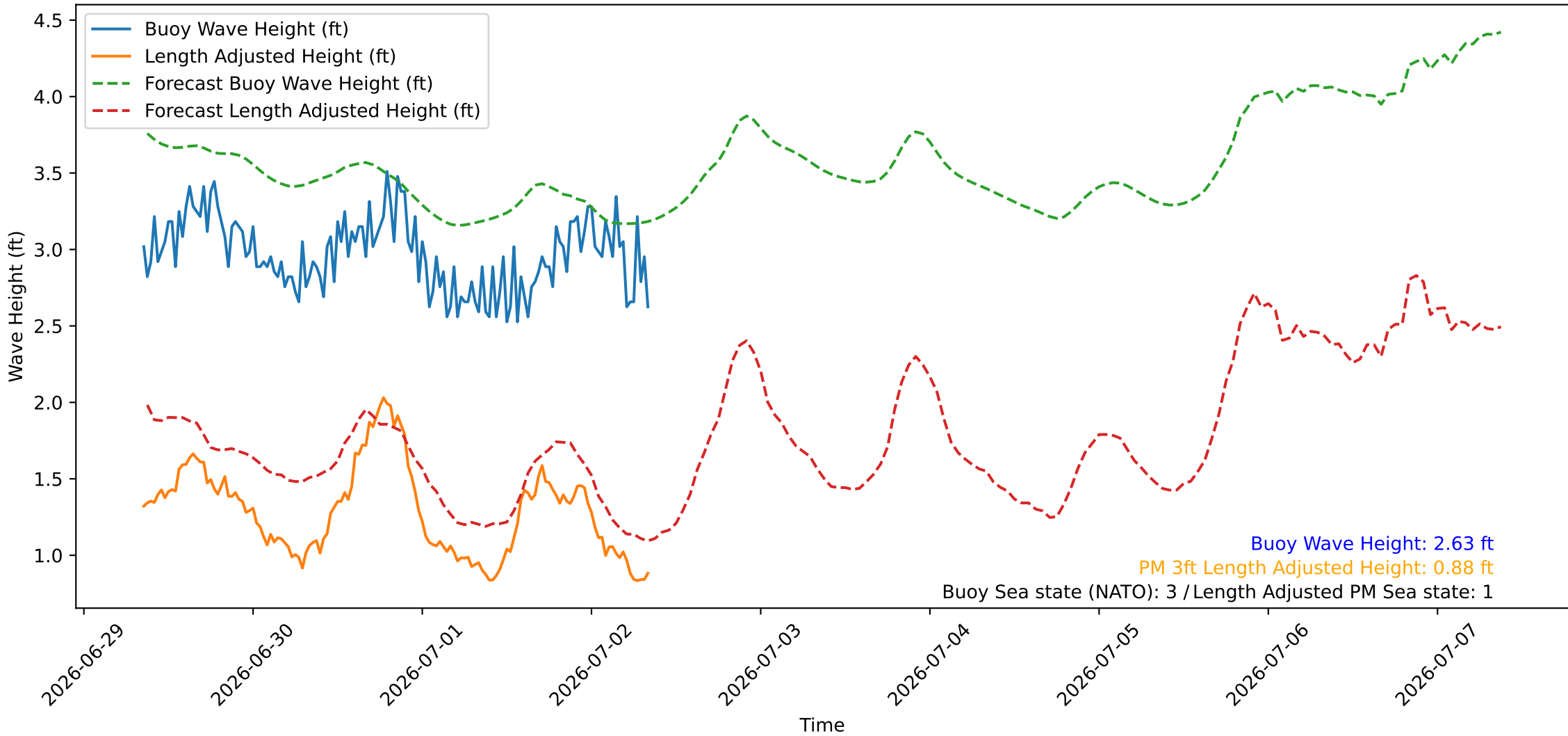
Wave Heights over Time for Green Beach at 2026-07-02 08:41:09
