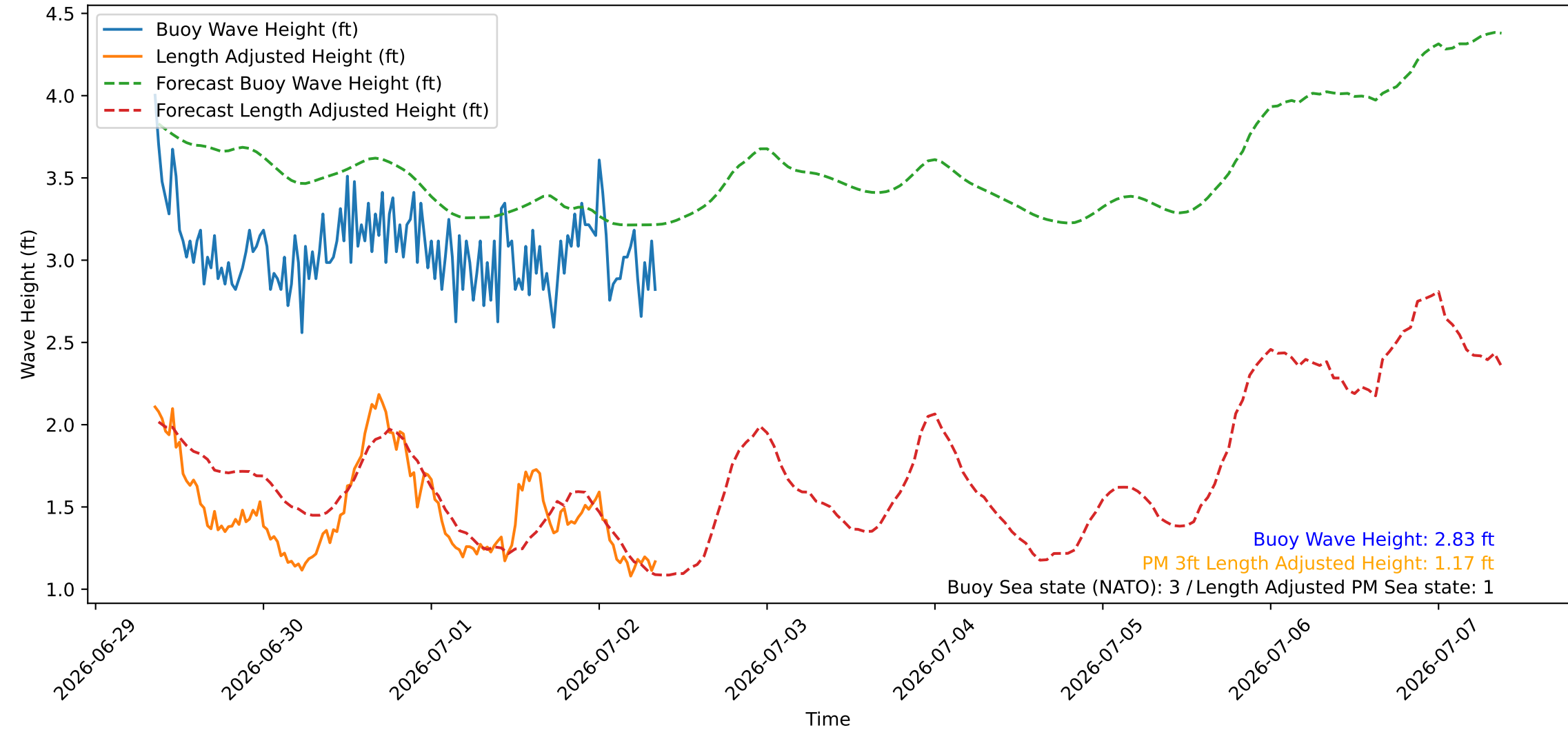
Wave Heights over Time for Oceanside Harbor at 2026-07-02 08:40:27
