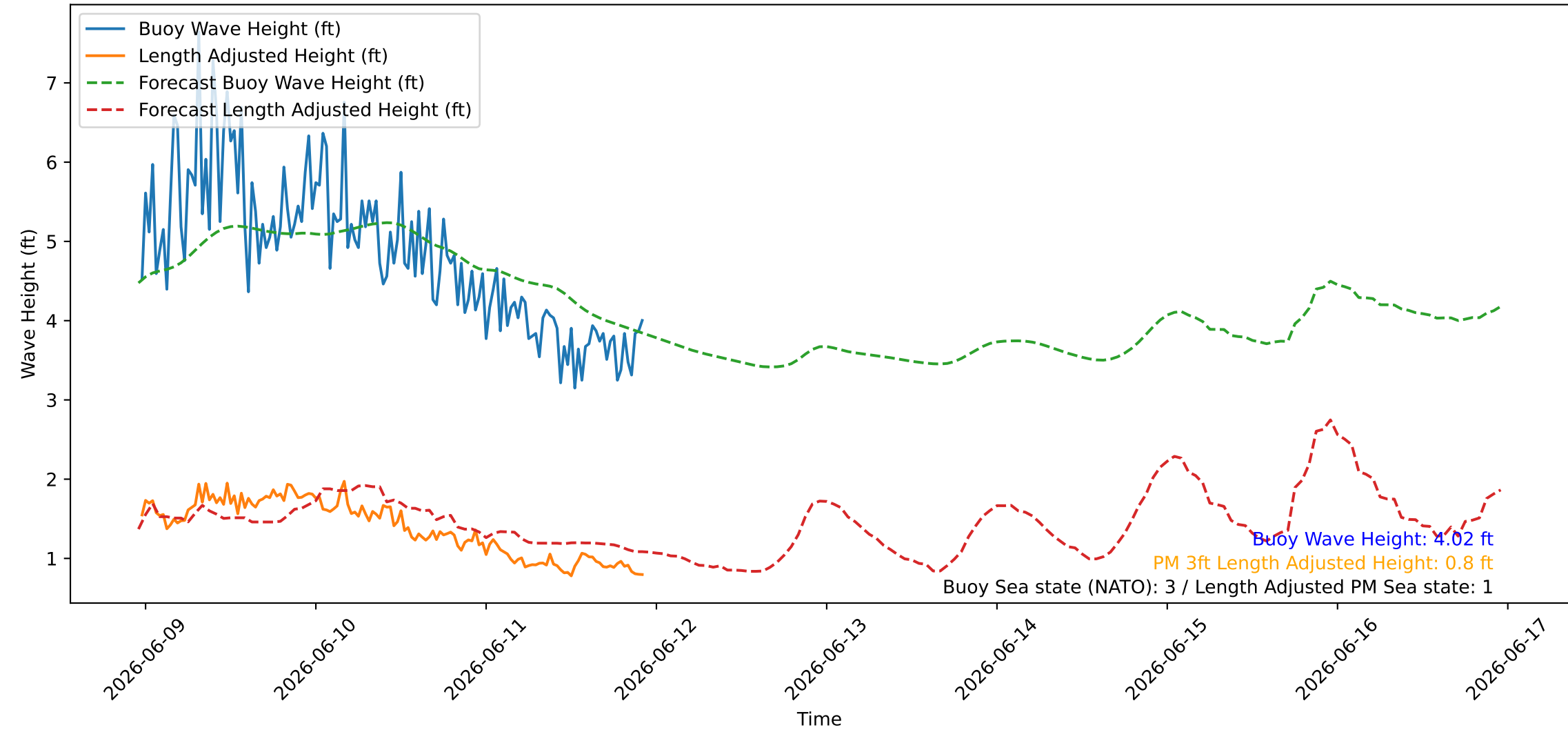
Wave Heights over Time for Red Beach at 2026-06-11 23:00:46
