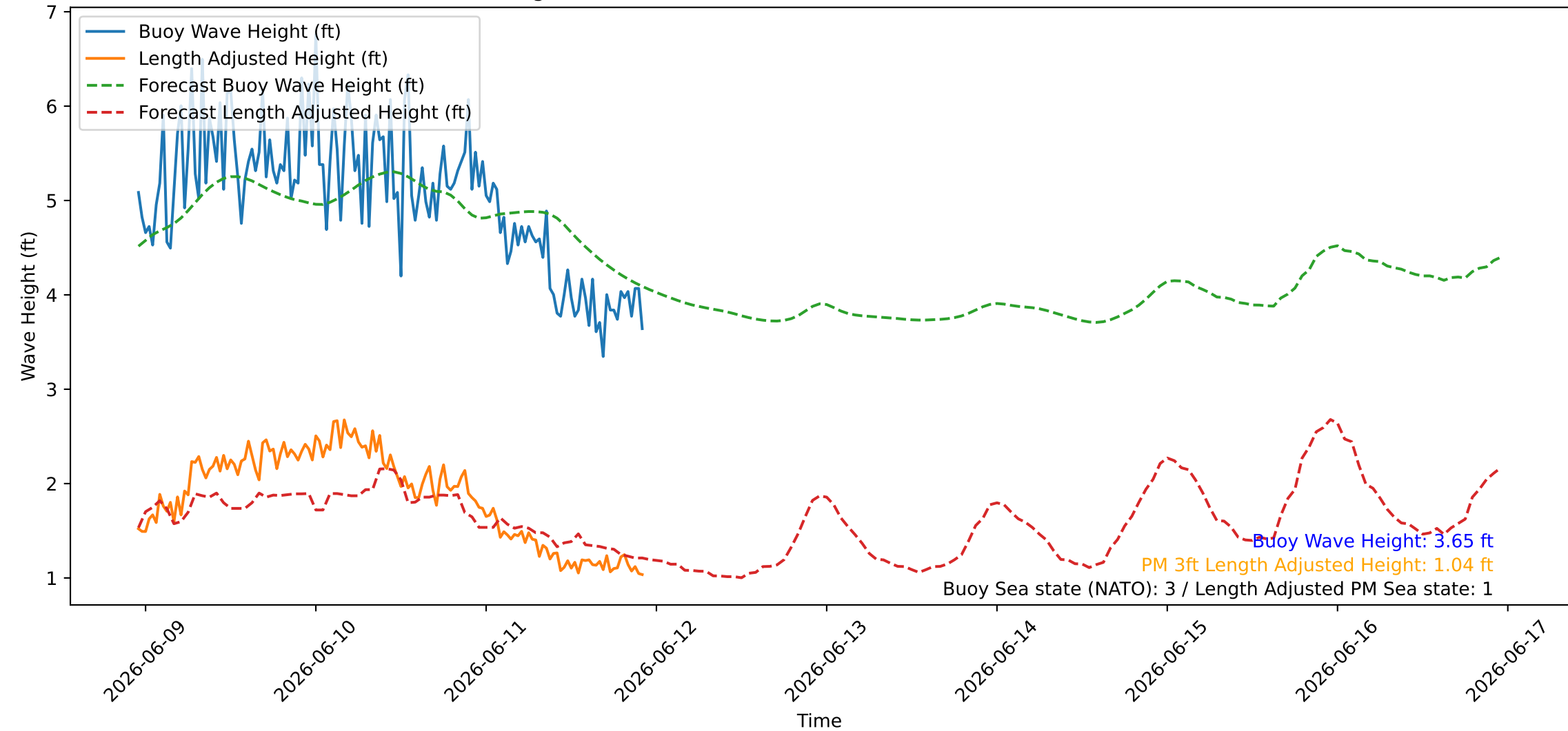
Wave Heights over Time for Oceanside Harbor at 2026-06-11 23:00:26
