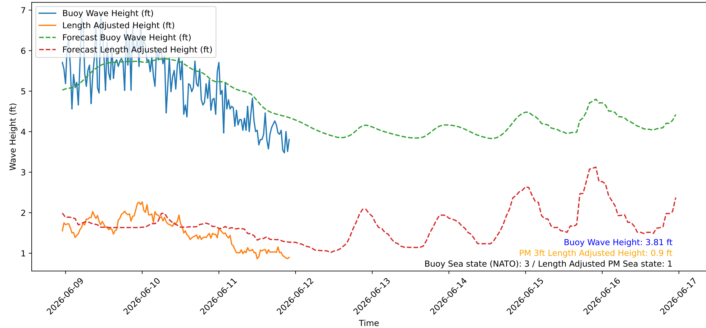
Wave Heights over Time for Green Beach at 2026-06-11 23:01:09
