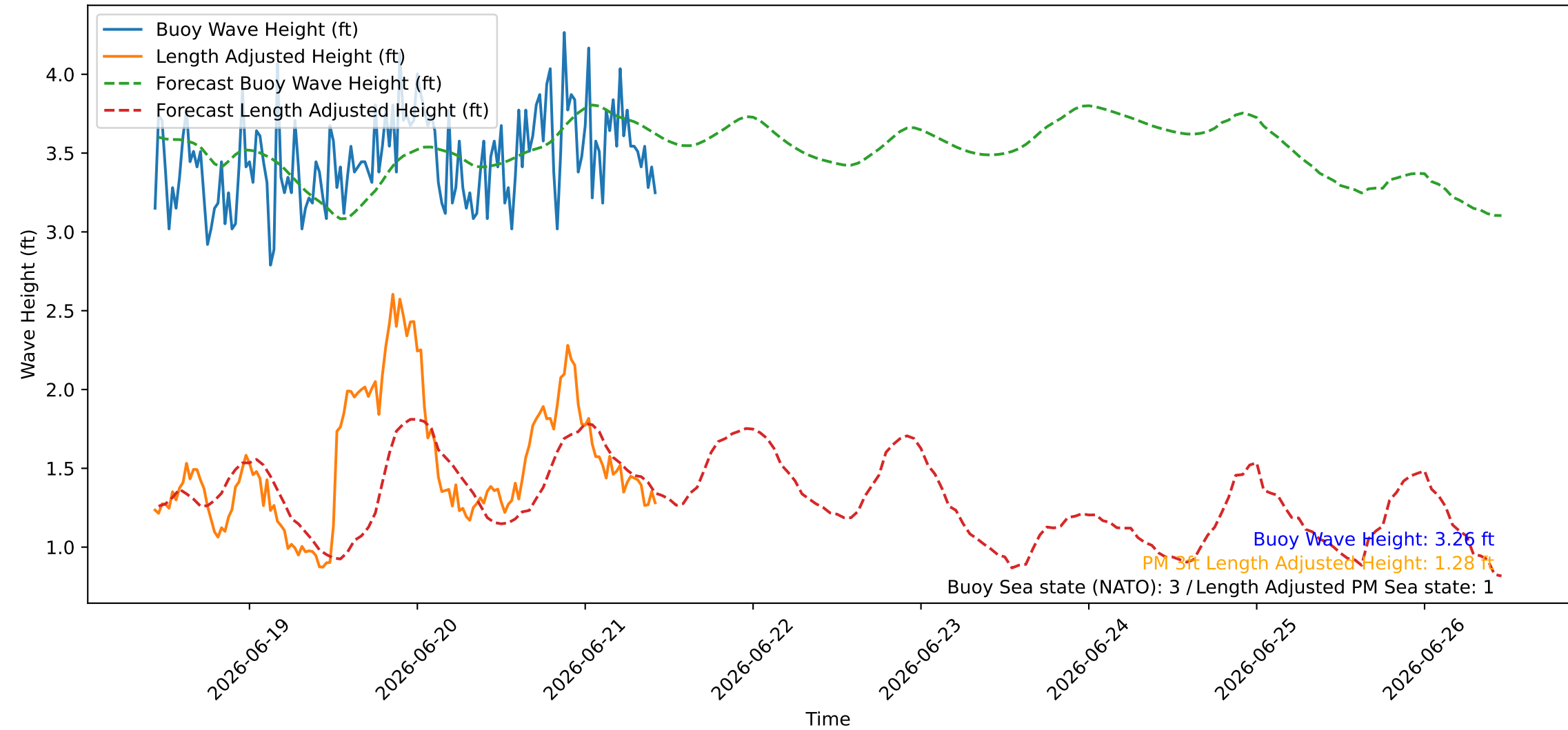
Wave Heights over Time for Oceanside Harbor at 2026-06-21 10:40:26
