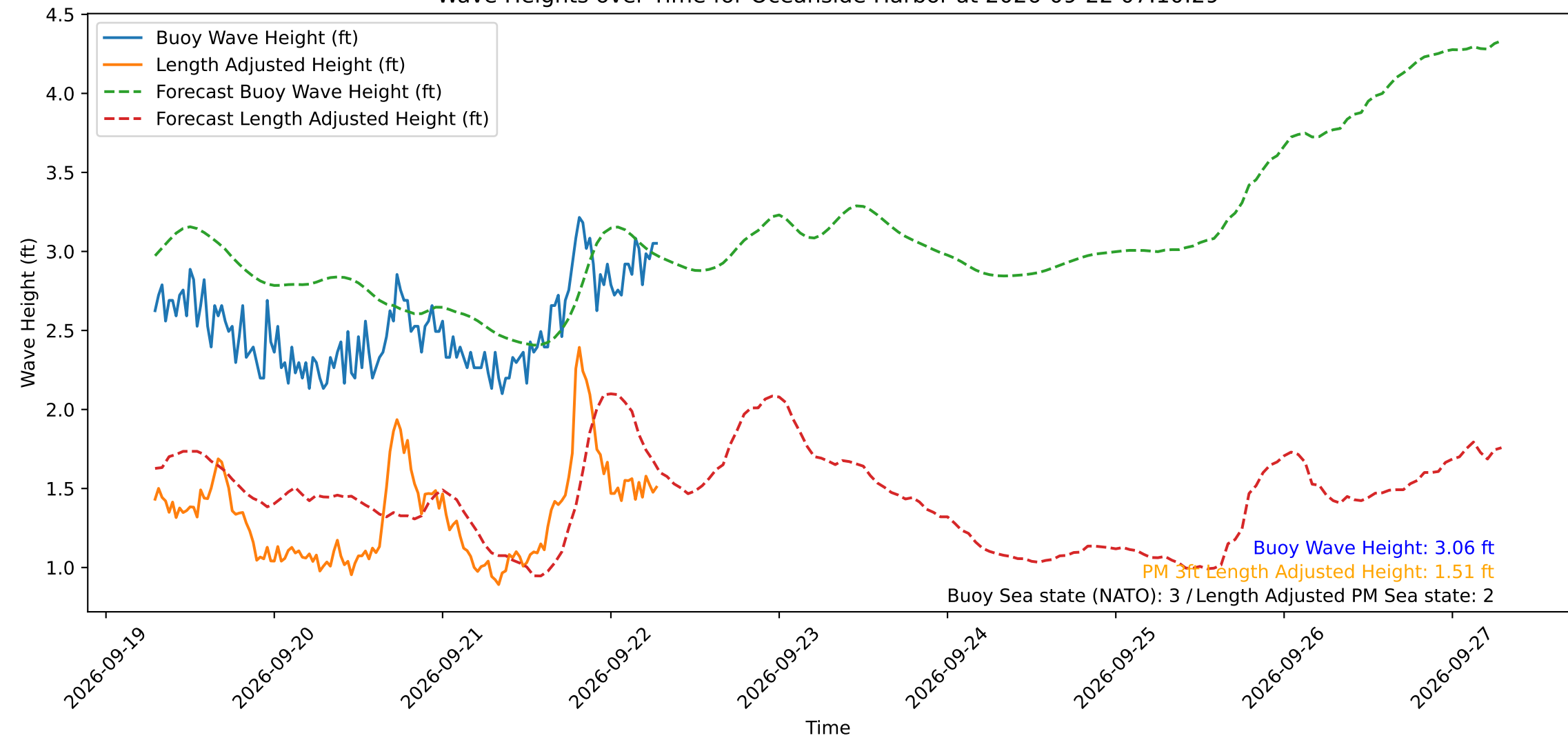
Wave Heights over Time for Oceanside Harbor at 2026-09-22 07:10:29
