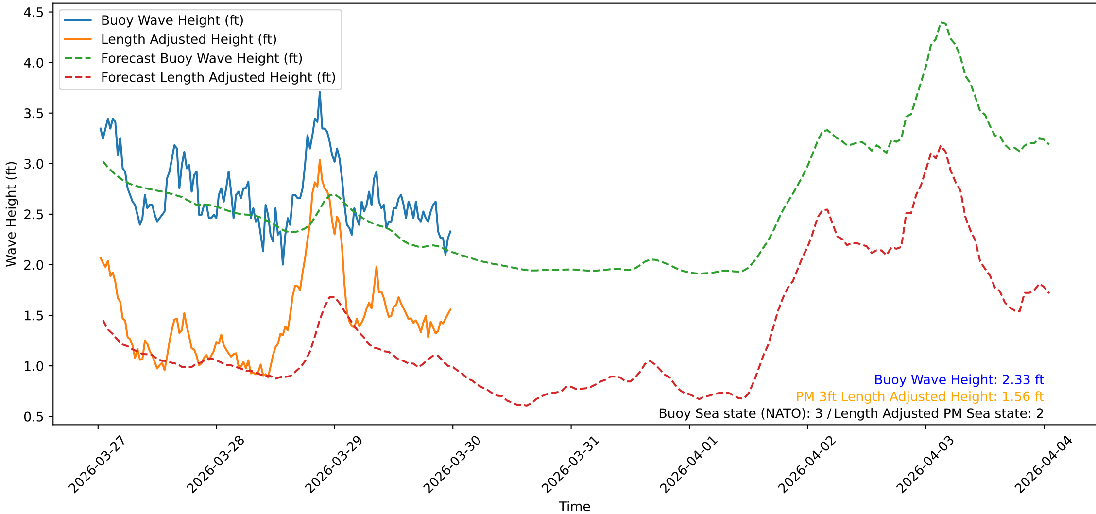
Wave Heights over Time for Green Beach at 2026-03-30 00:31:09
