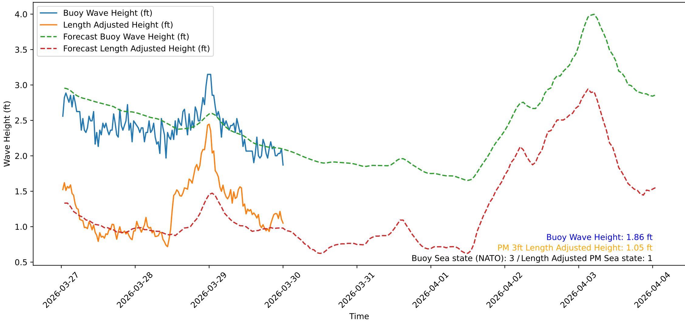
Wave Heights over Time for Oceanside Harbor at 2026-03-30 00:30:31
