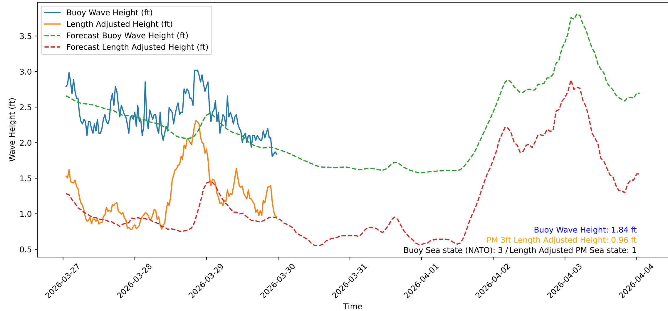
Wave Heights over Time for Red Beach at 2026-03-30 00:30:47
