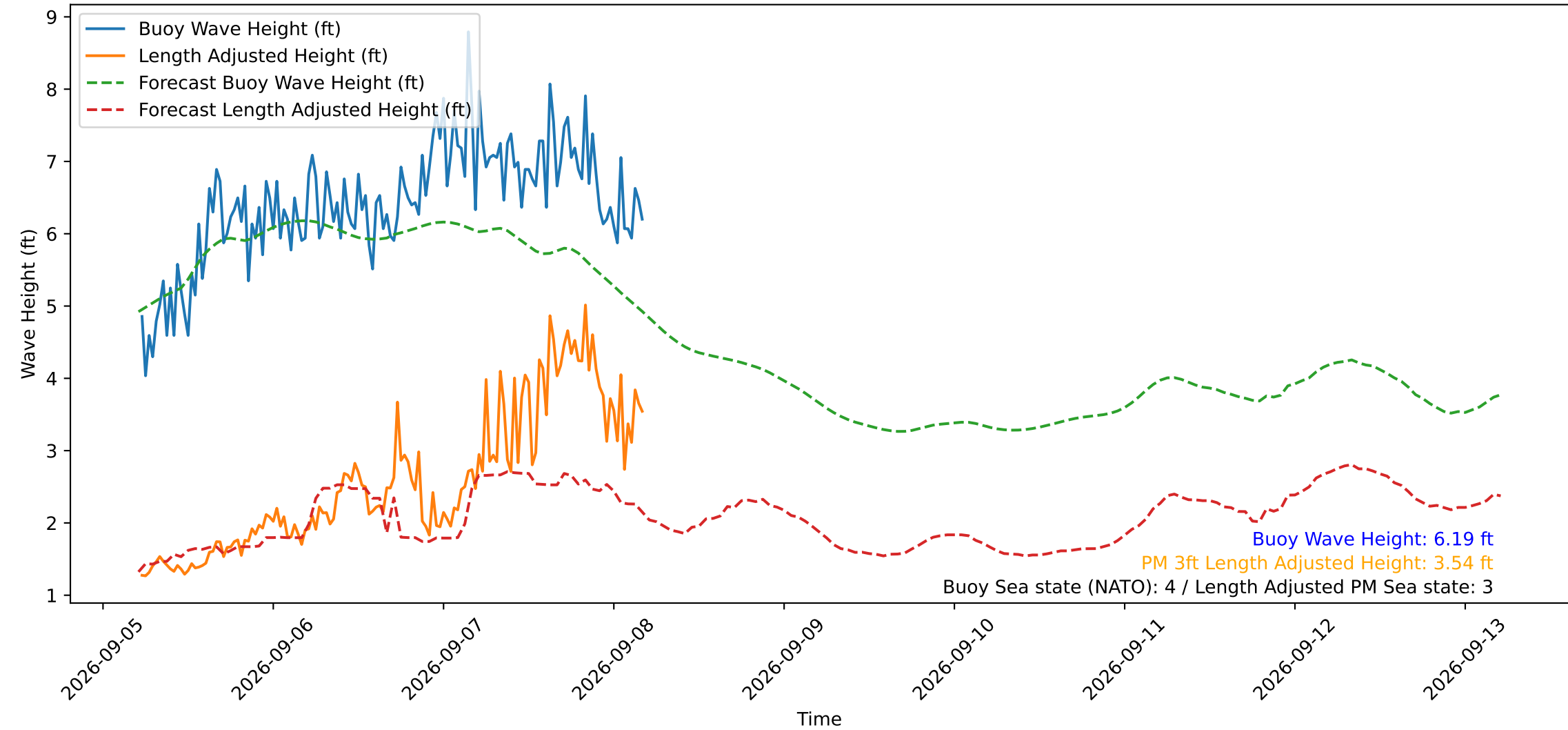
Wave Heights over Time for Green Beach at 2026-09-08 05:01:12
