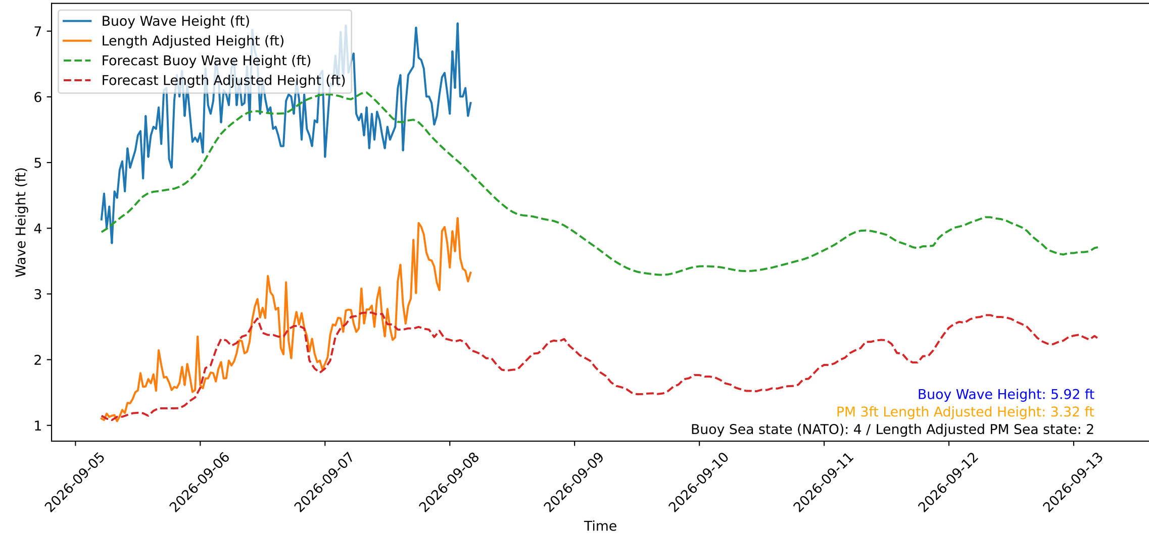
Wave Heights over Time for Oceanside Harbor at 2026-09-08 05:00:30
