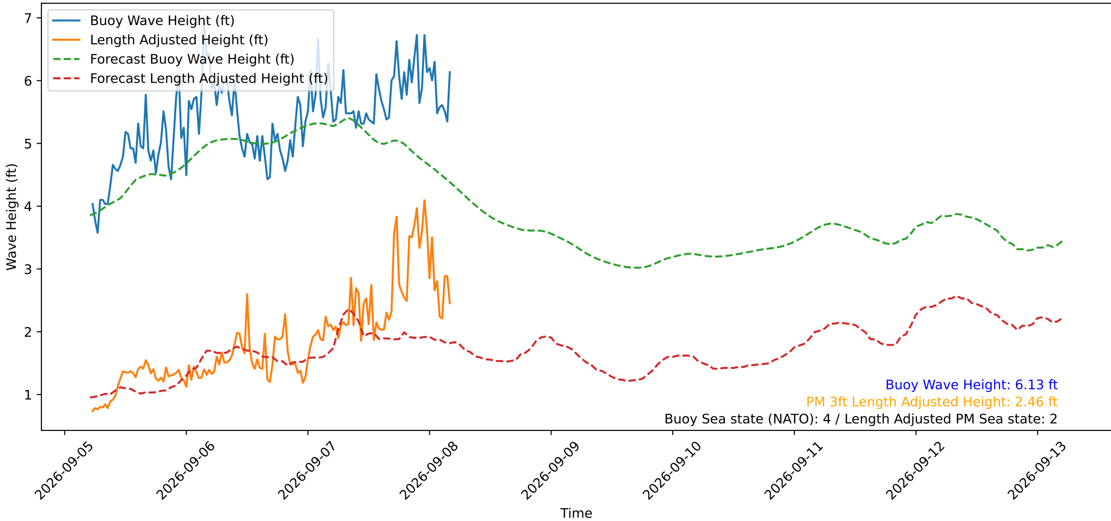
Wave Heights over Time for Red Beach at 2026-09-08 05:00:49
