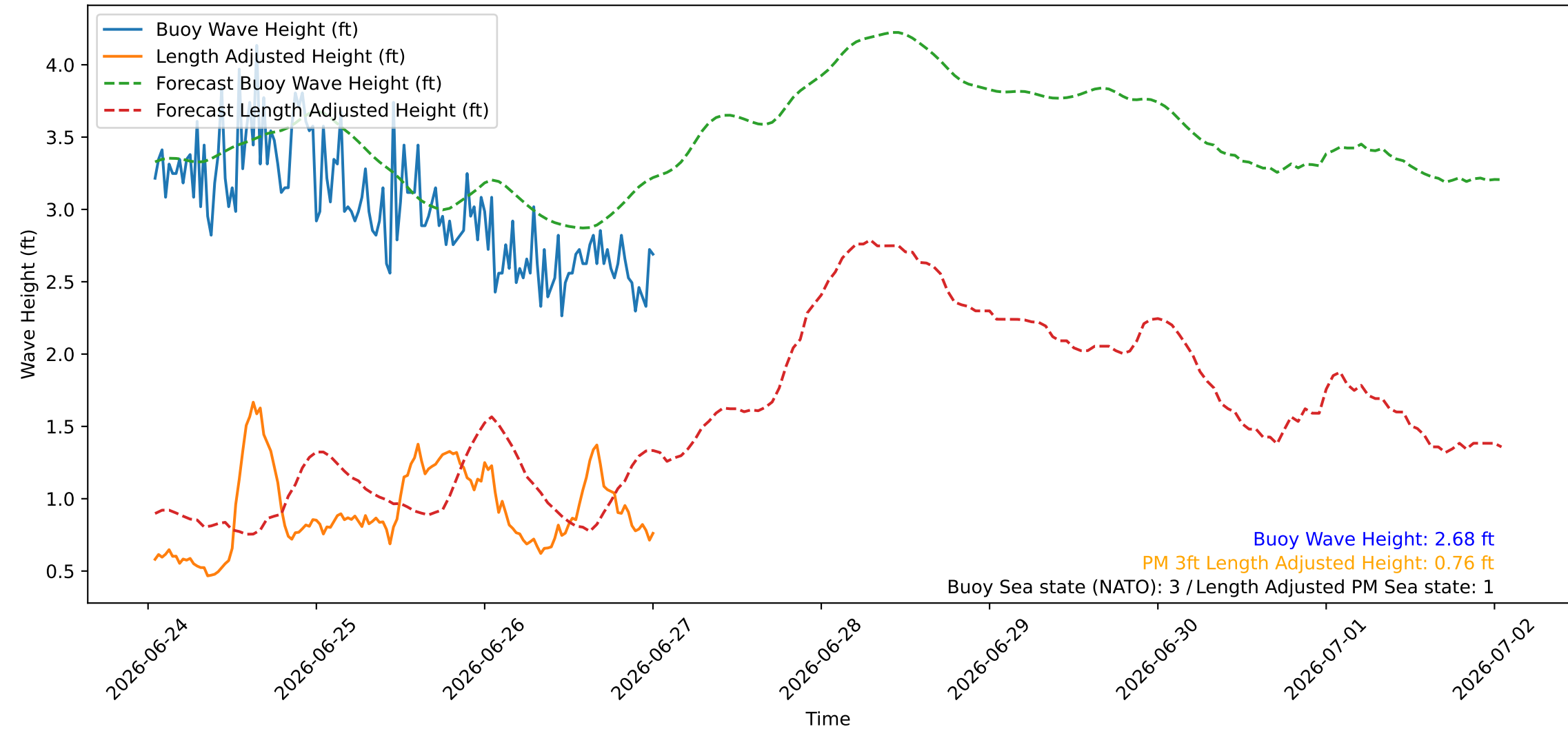
Wave Heights over Time for Red Beach at 2026-06-27 00:40:45
