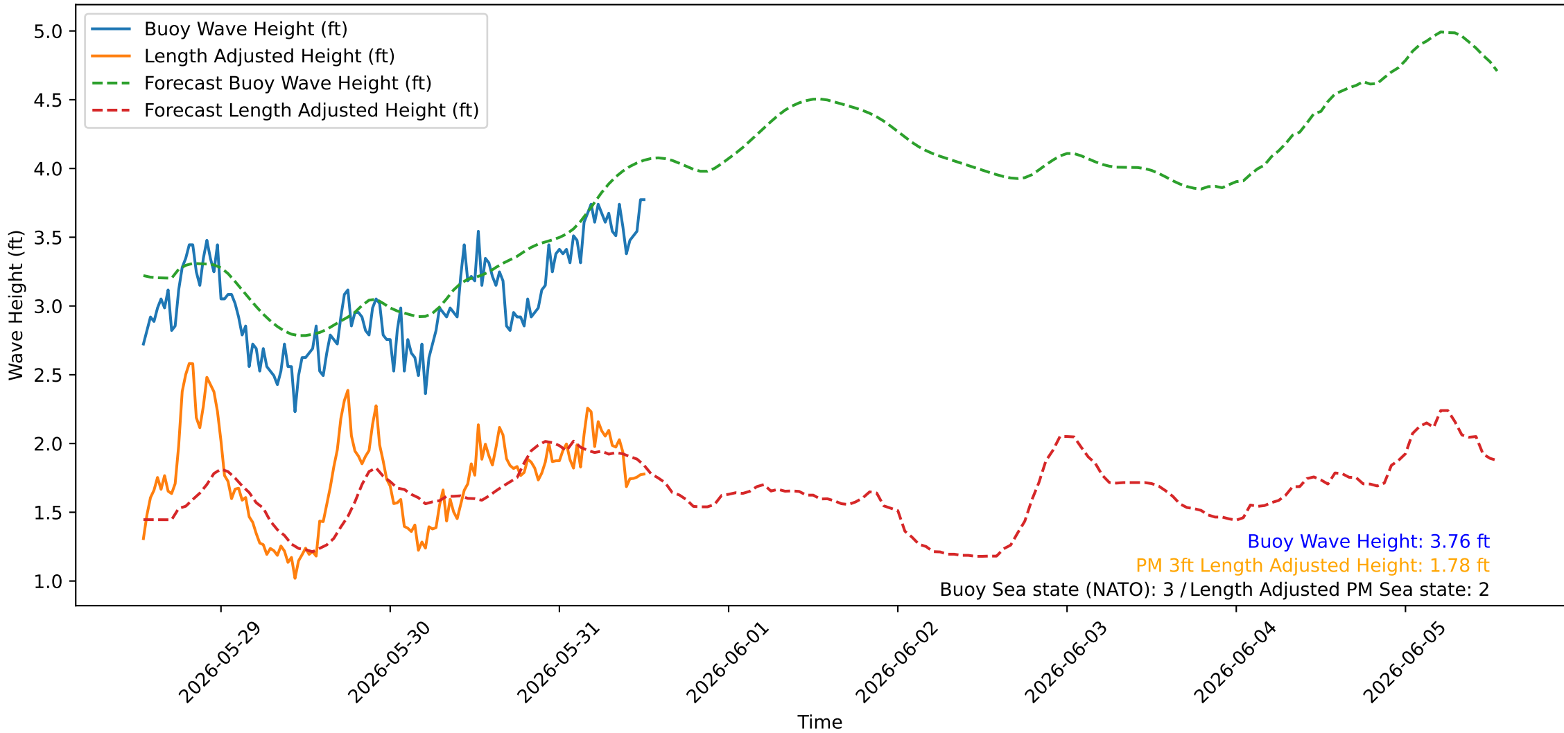
Wave Heights over Time for Oceanside Harbor at 2026-05-31 13:00:26
