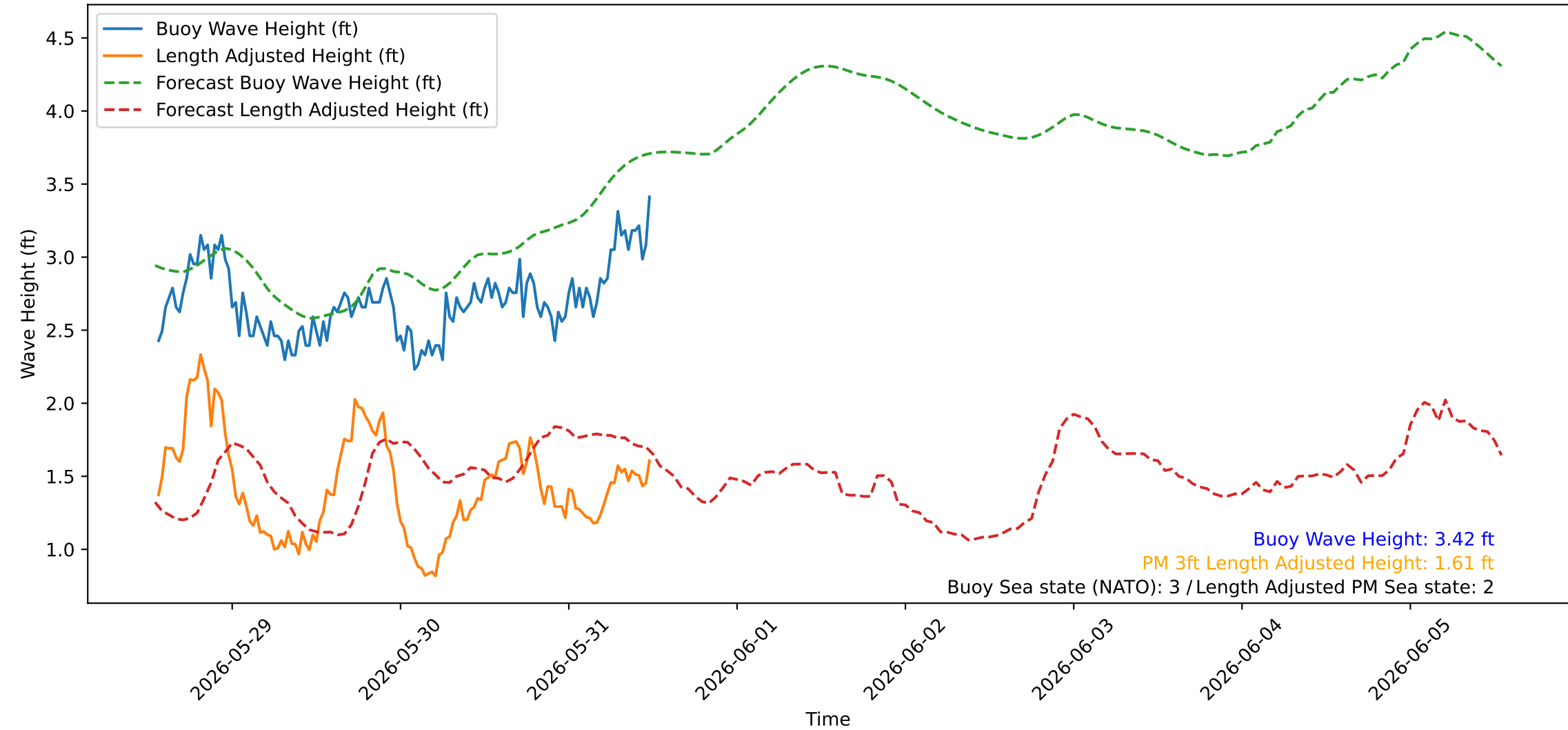
Wave Heights over Time for Red Beach at 2026-05-31 13:00:45
