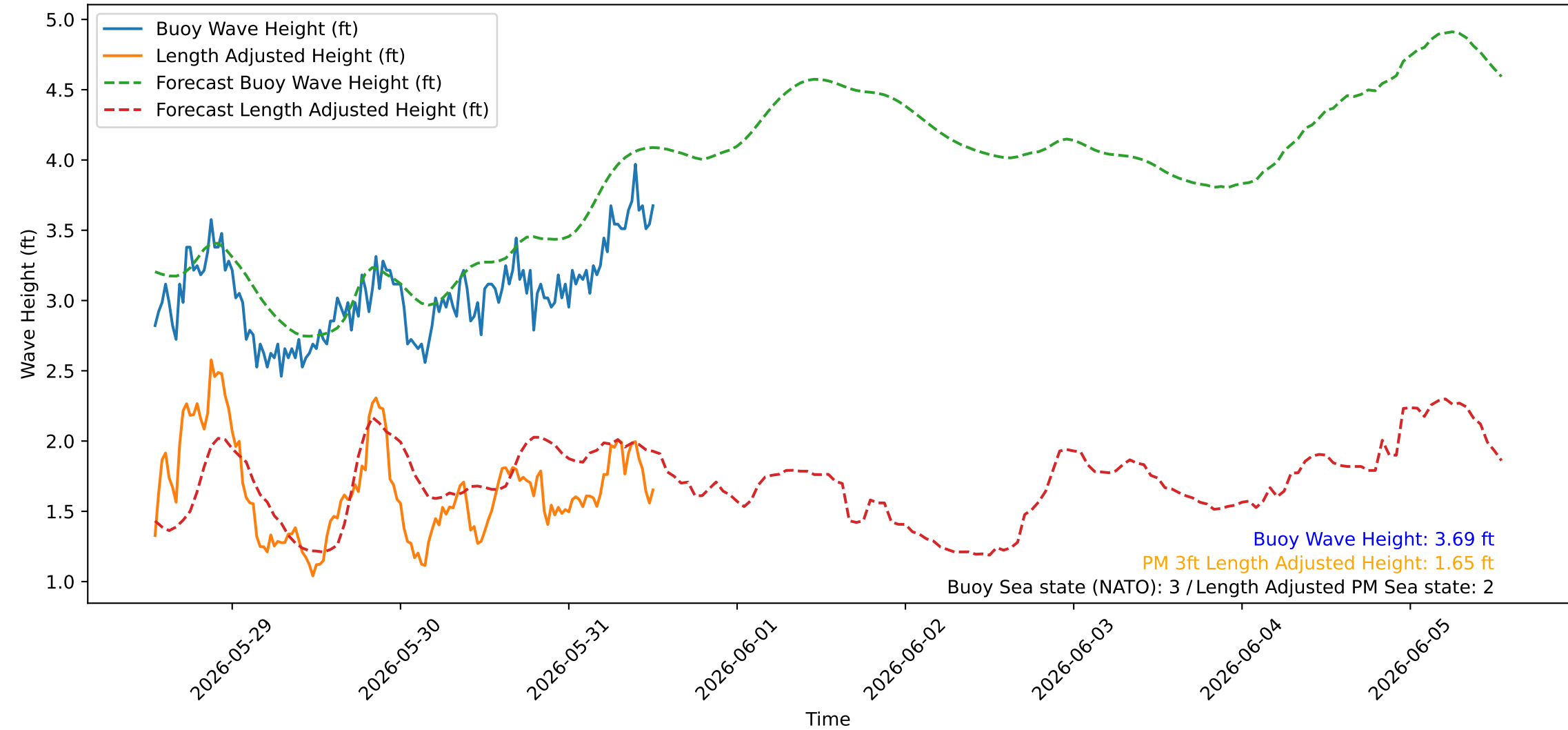
Wave Heights over Time for Green Beach at 2026-05-31 13:01:08
