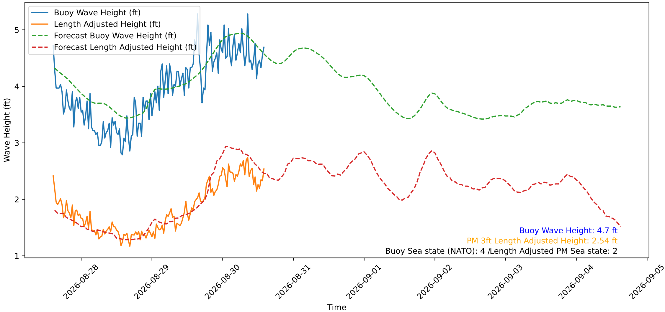
Wave Heights over Time for Oceanside Harbor at 2026-08-30 14:40:29
