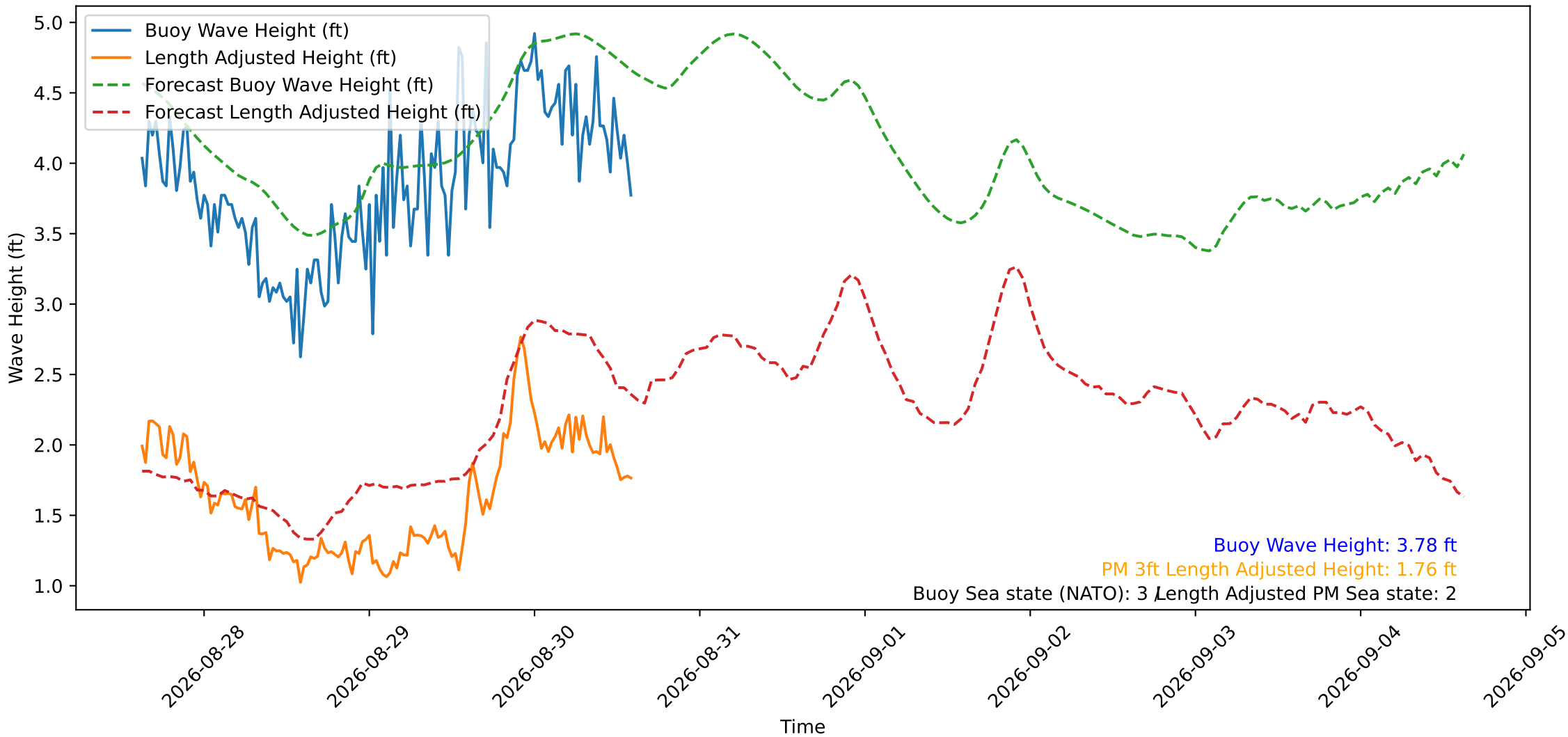
Wave Heights over Time for Green Beach at 2026-08-30 14:41:12
