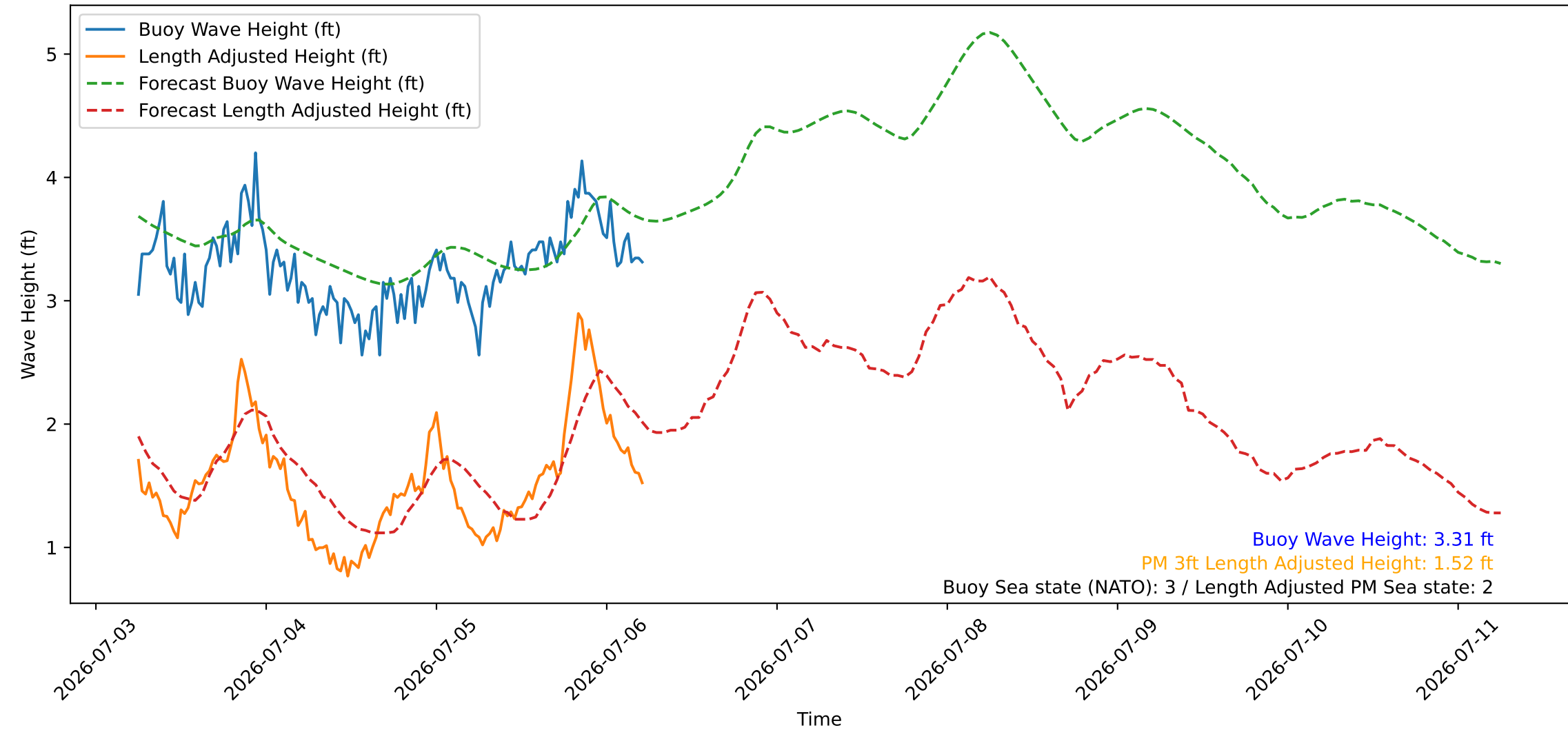
Wave Heights over Time for Green Beach at 2026-07-06 05:51:10
