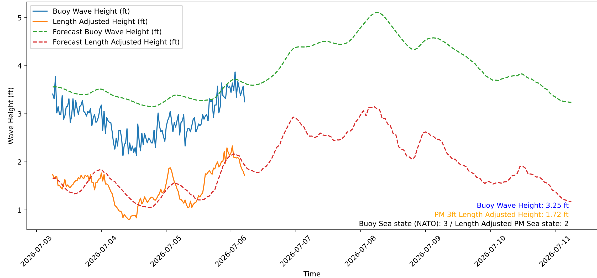
Wave Heights over Time for Oceanside Harbor at 2026-07-06 05:50:27
