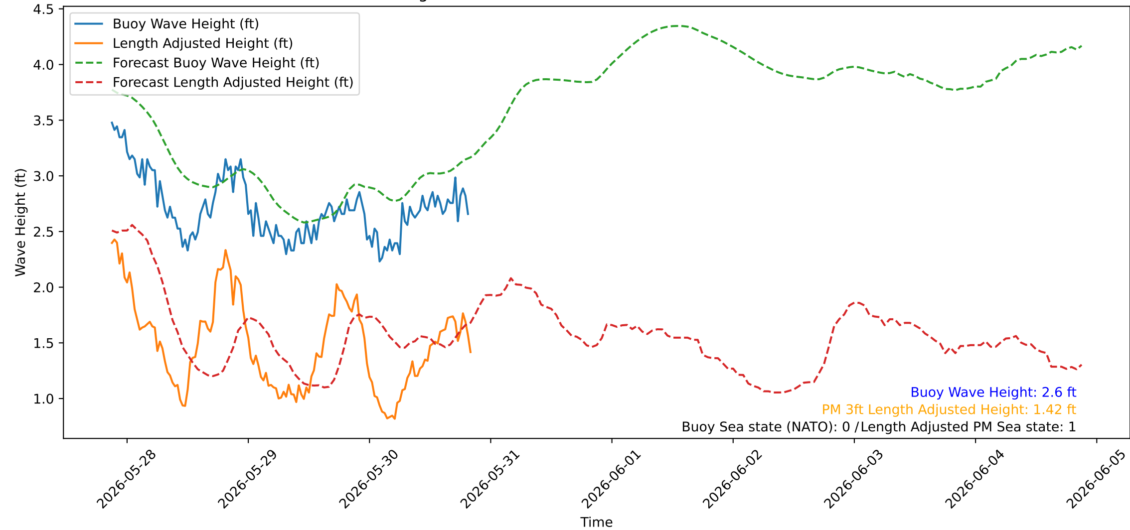
Wave Heights over Time for Red Beach at 2026-05-30 20:40:43
