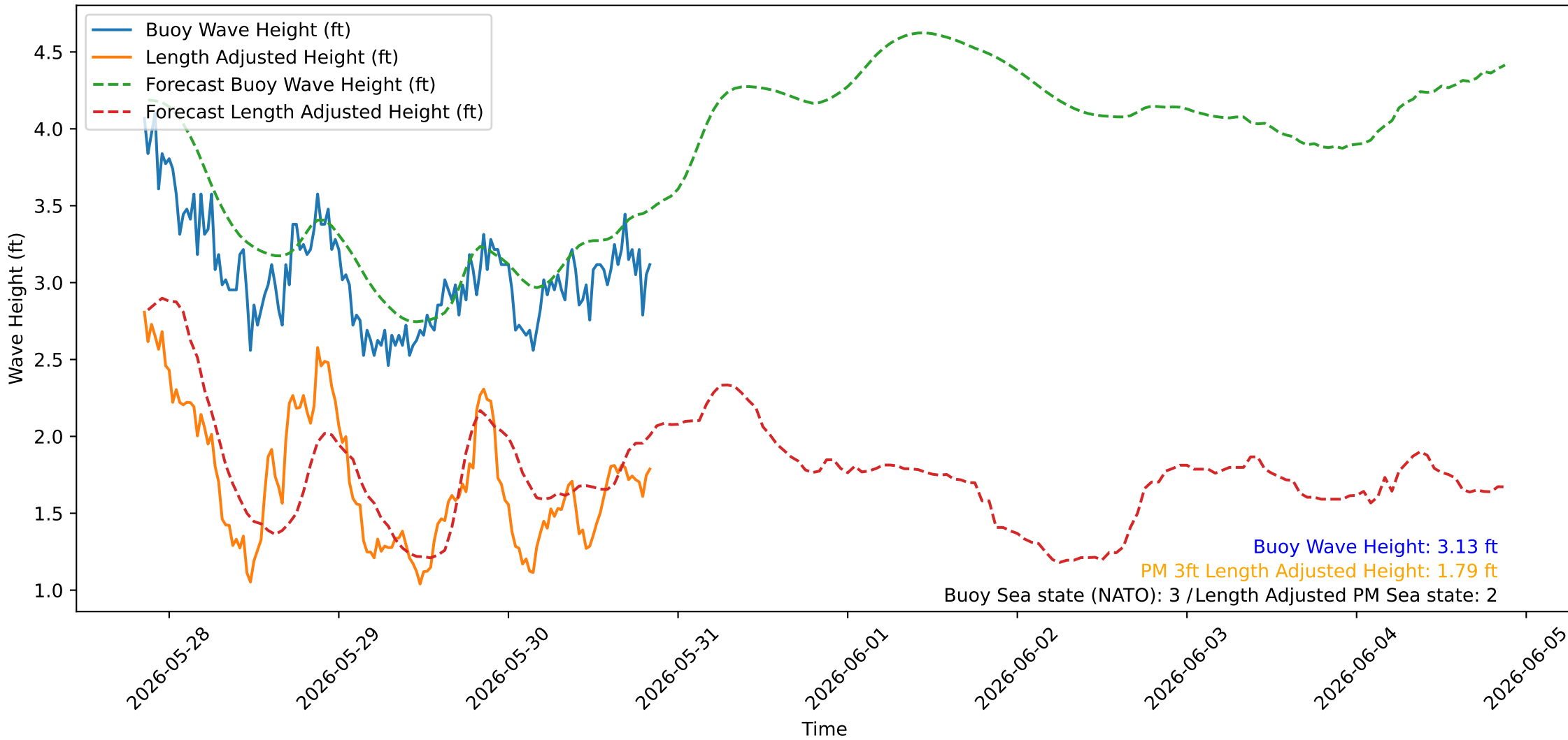
Wave Heights over Time for Green Beach at 2026-05-30 20:41:06
