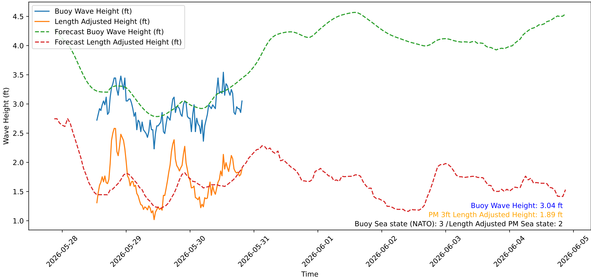
Wave Heights over Time for Oceanside Harbor at 2026-05-30 20:40:24
