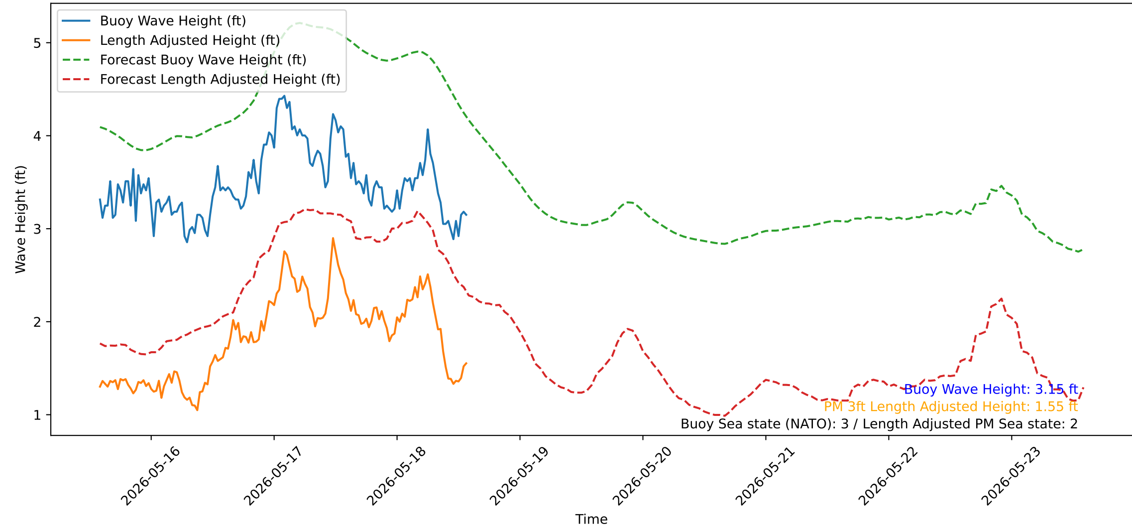
Wave Heights over Time for Green Beach at 2026-05-18 14:11:13
