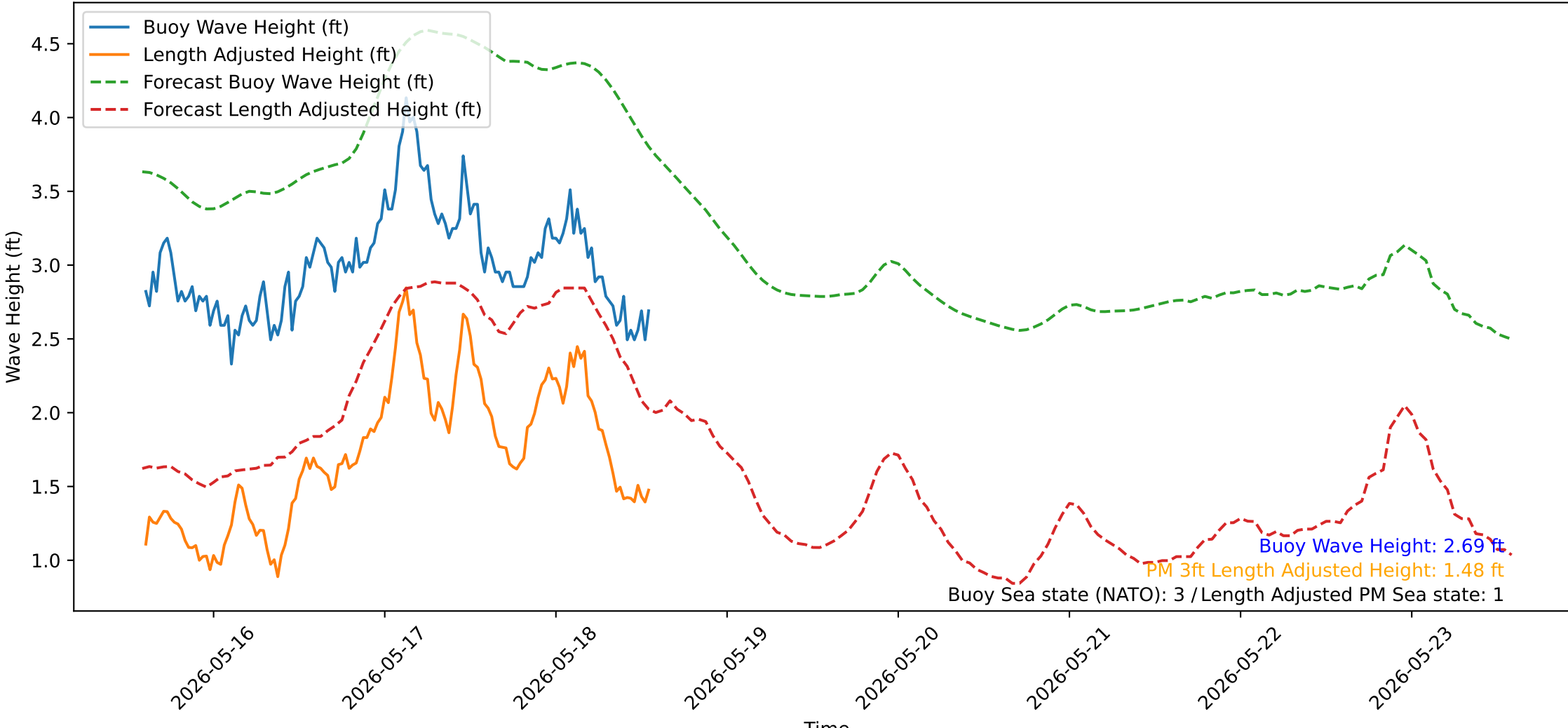
Wave Heights over Time for Red Beach at 2026-05-18 14:10:51
