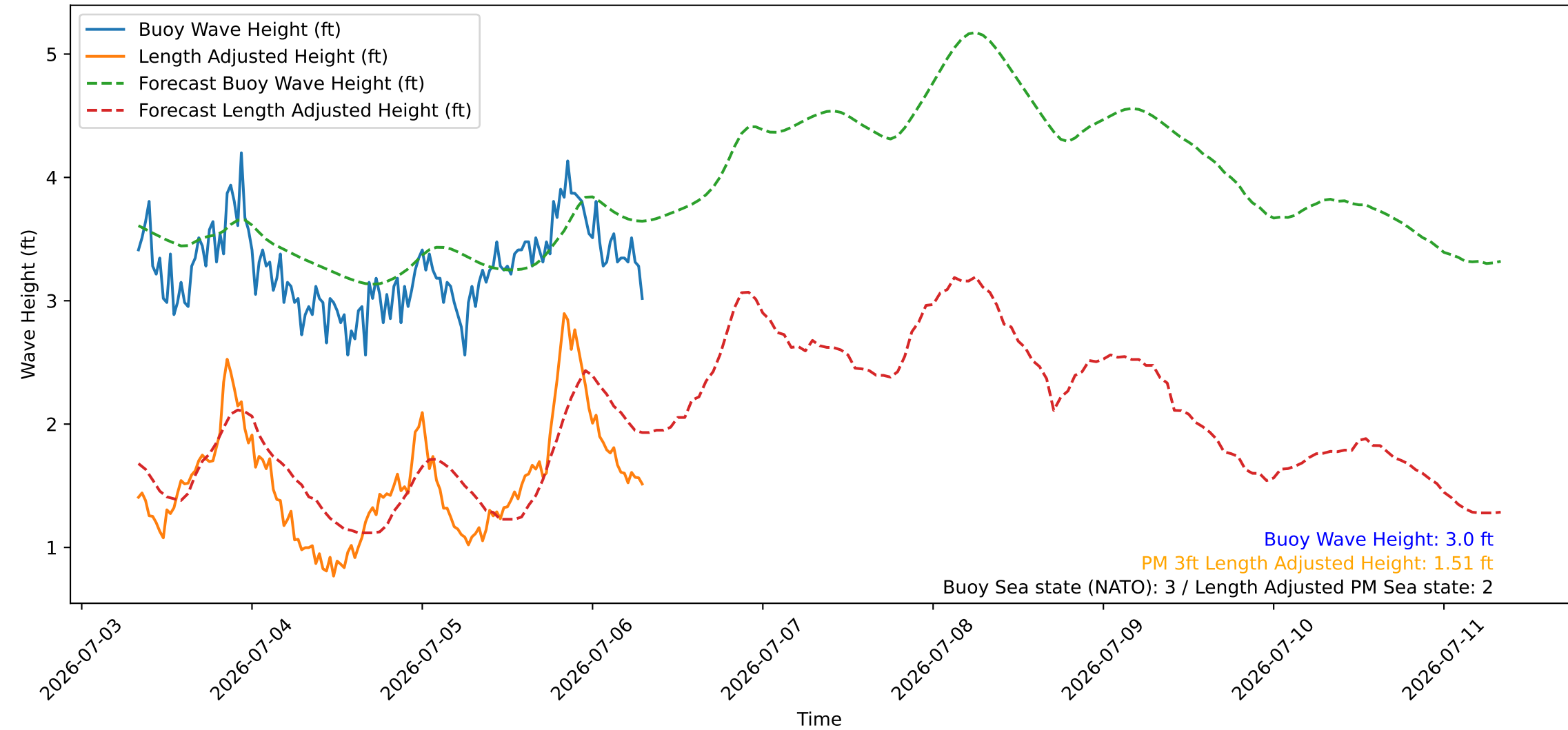
Wave Heights over Time for Green Beach at 2026-07-06 08:01:09
