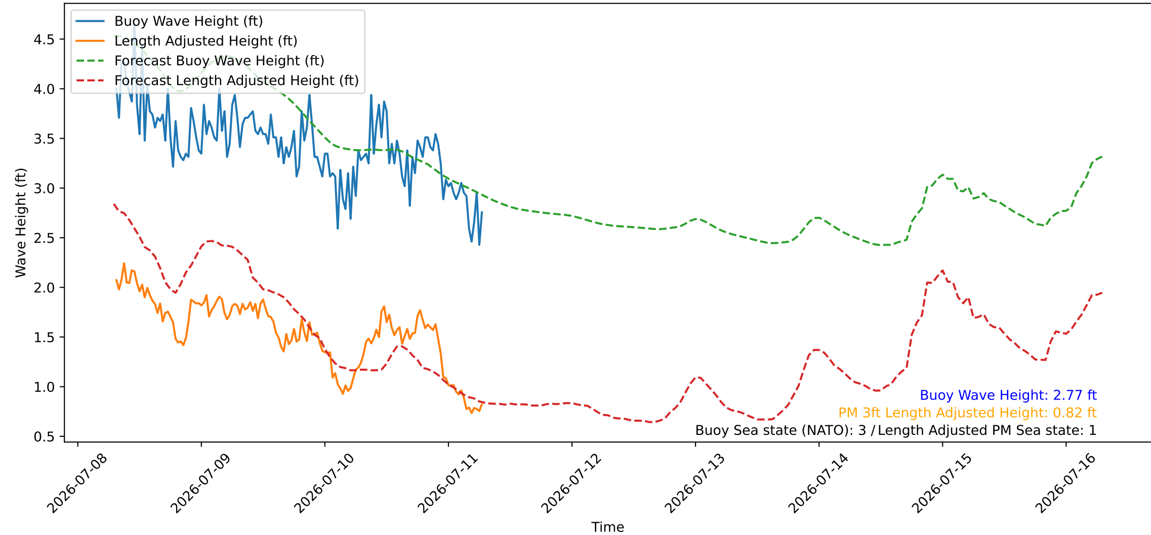
Wave Heights over Time for Red Beach at 2026-07-11 07:20:47
