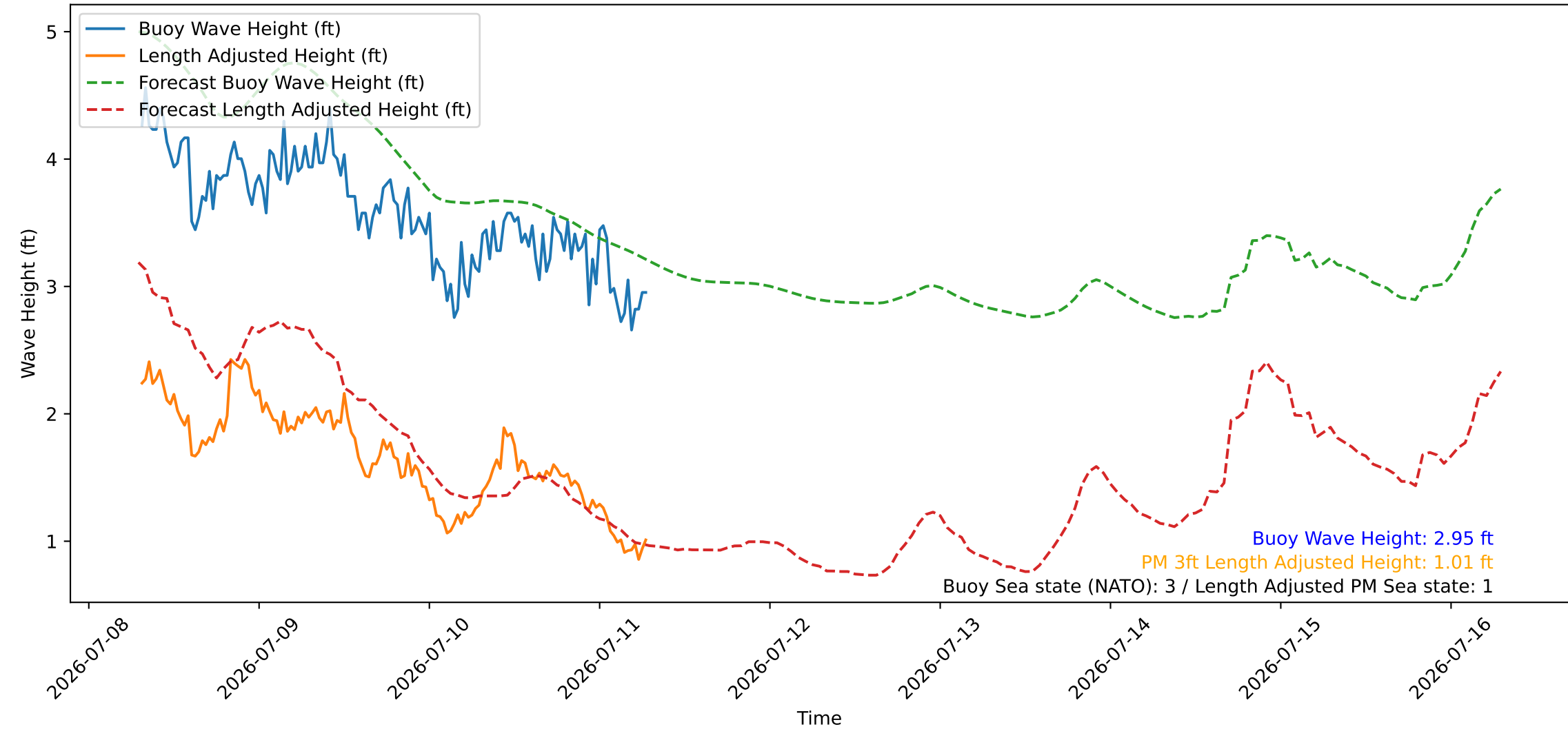
Wave Heights over Time for Green Beach at 2026-07-11 07:21:09
