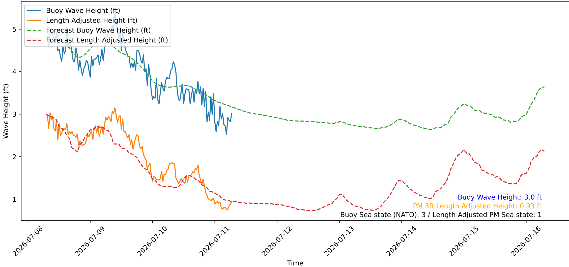
Wave Heights over Time for Oceanside Harbor at 2026-07-11 07:20:26
