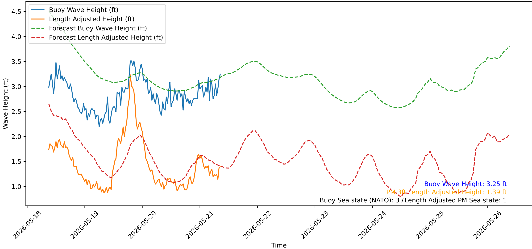
Wave Heights over Time for Oceanside Harbor at 2026-05-21 09:10:31
