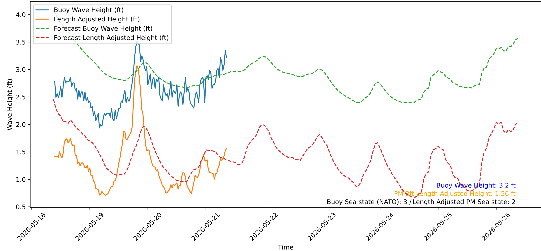
Wave Heights over Time for Red Beach at 2026-05-21 09:10:52
