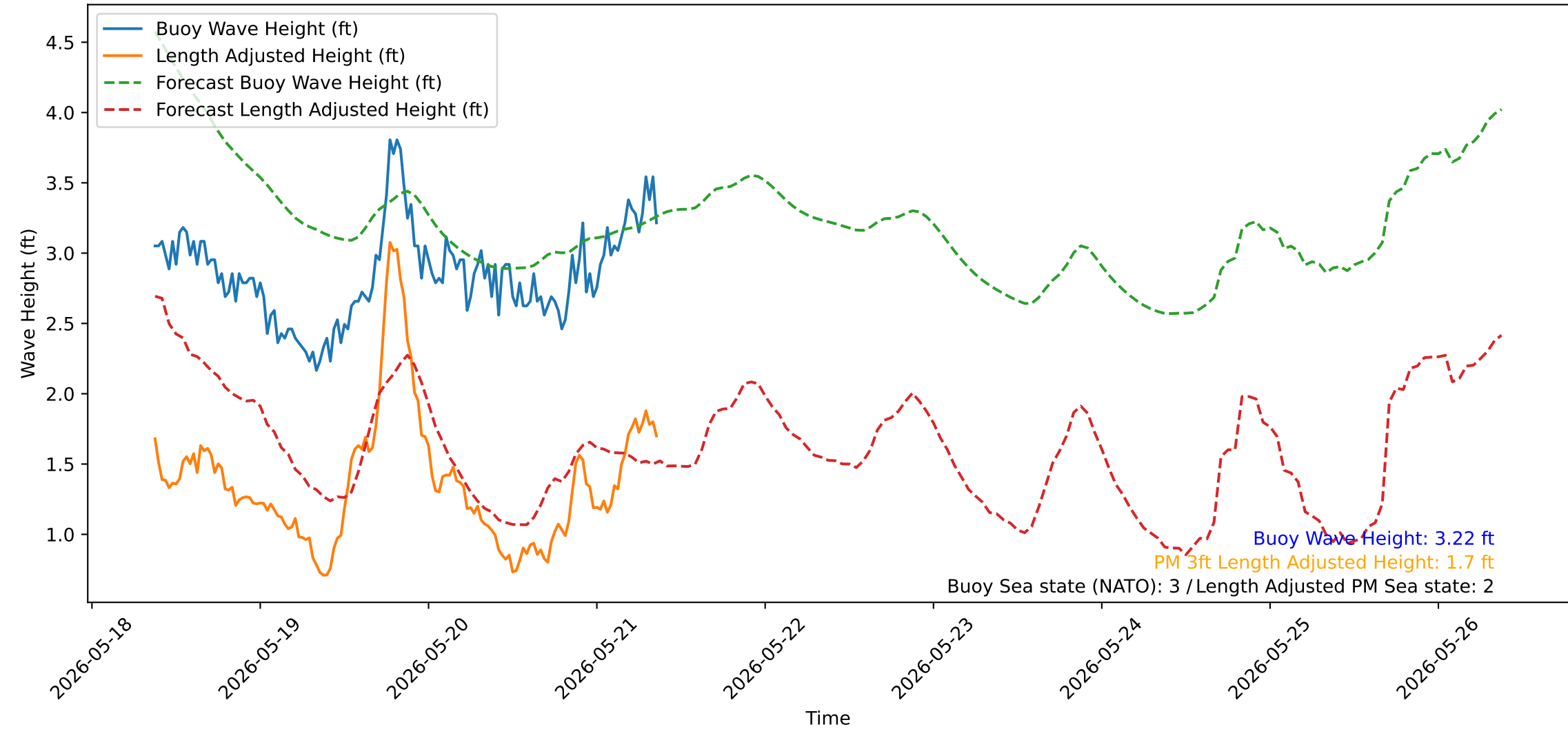
Wave Heights over Time for Green Beach at 2026-05-21 09:11:14
