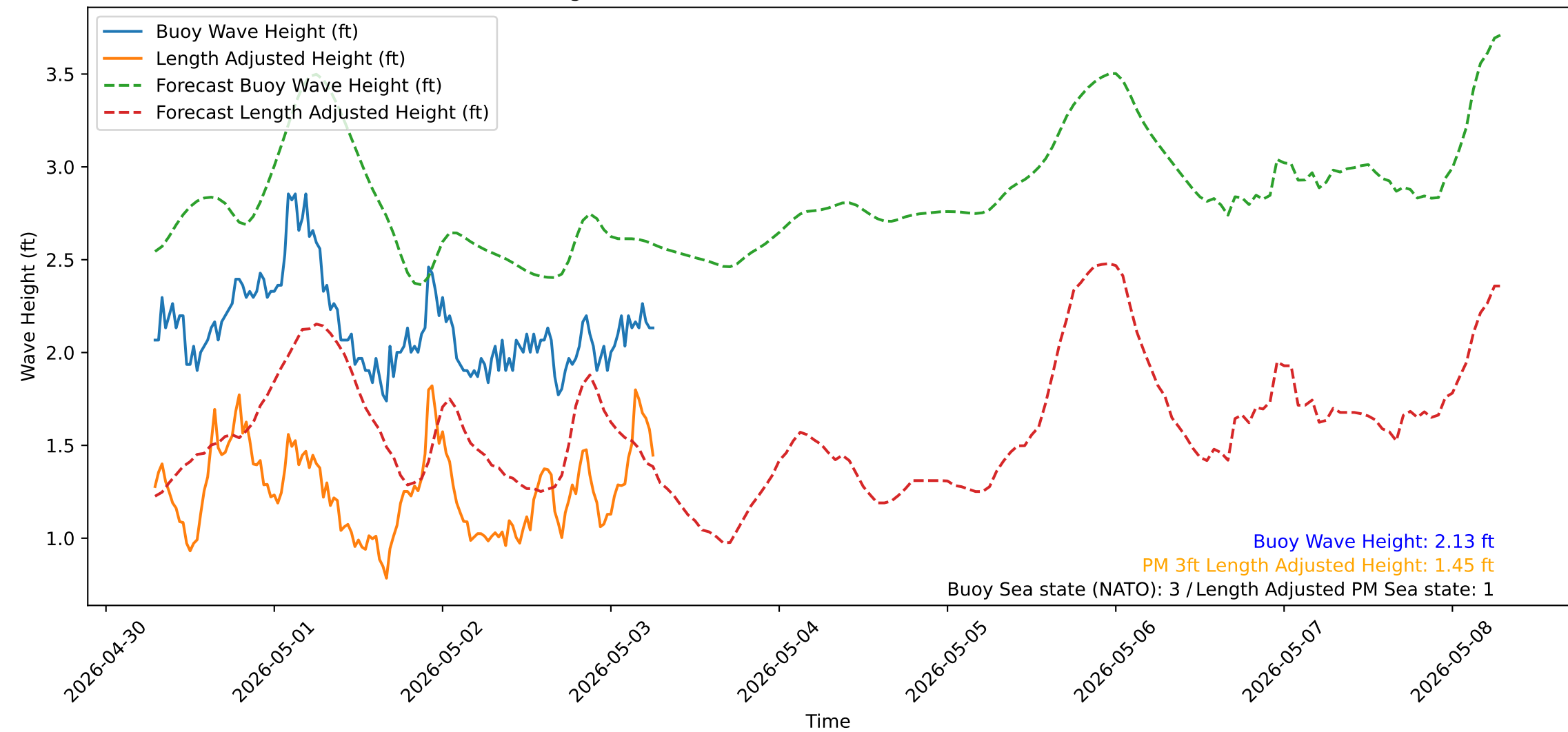
Wave Heights over Time for Green Beach at 2026-05-03 07:01:12
