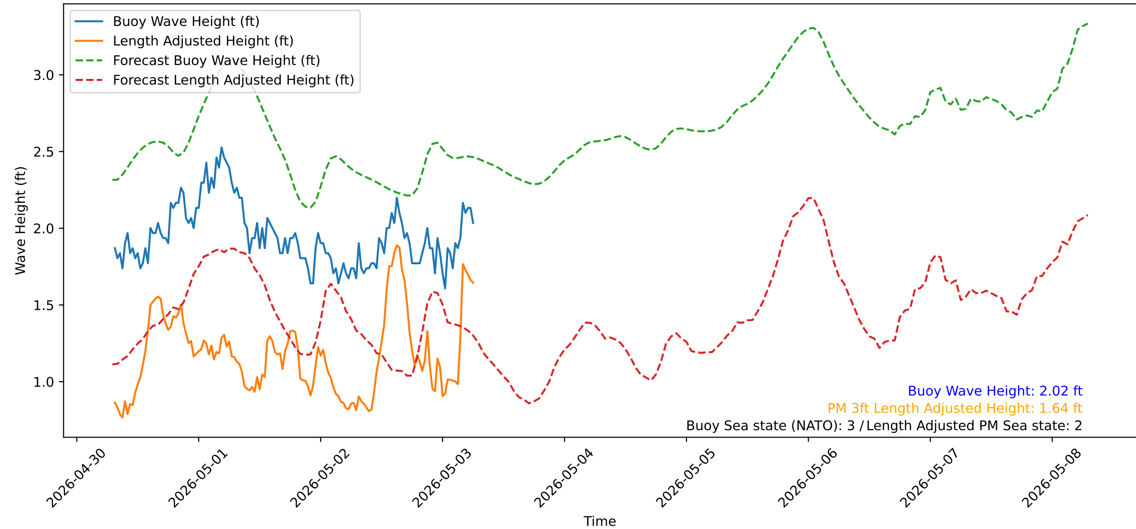
Wave Heights over Time for Red Beach at 2026-05-03 07:00:50
