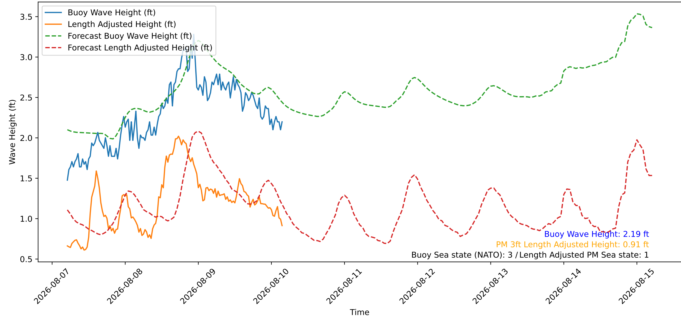
Wave Heights over Time for Red Beach at 2026-08-10 04:30:46
