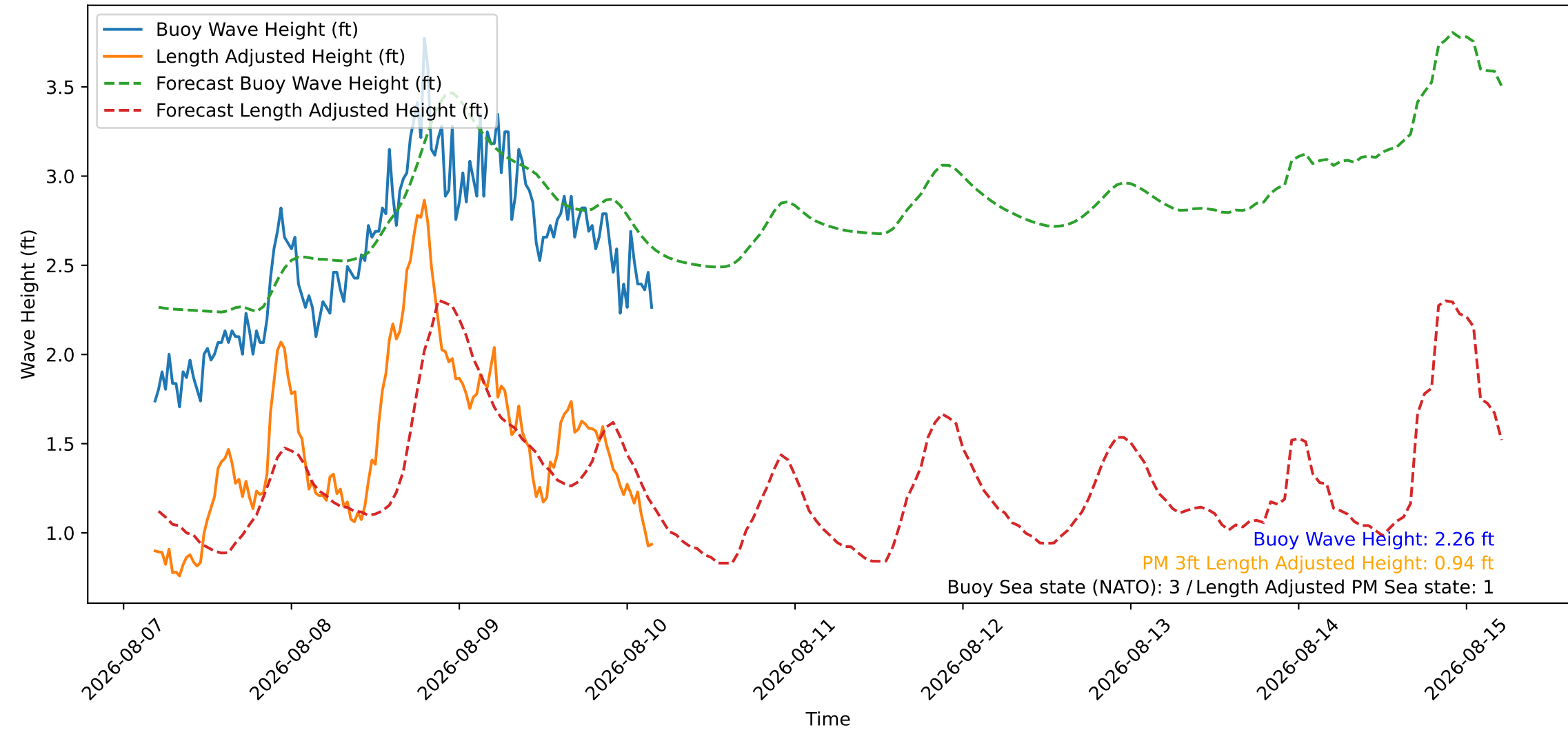
Wave Heights over Time for Green Beach at 2026-08-10 04:31:09
