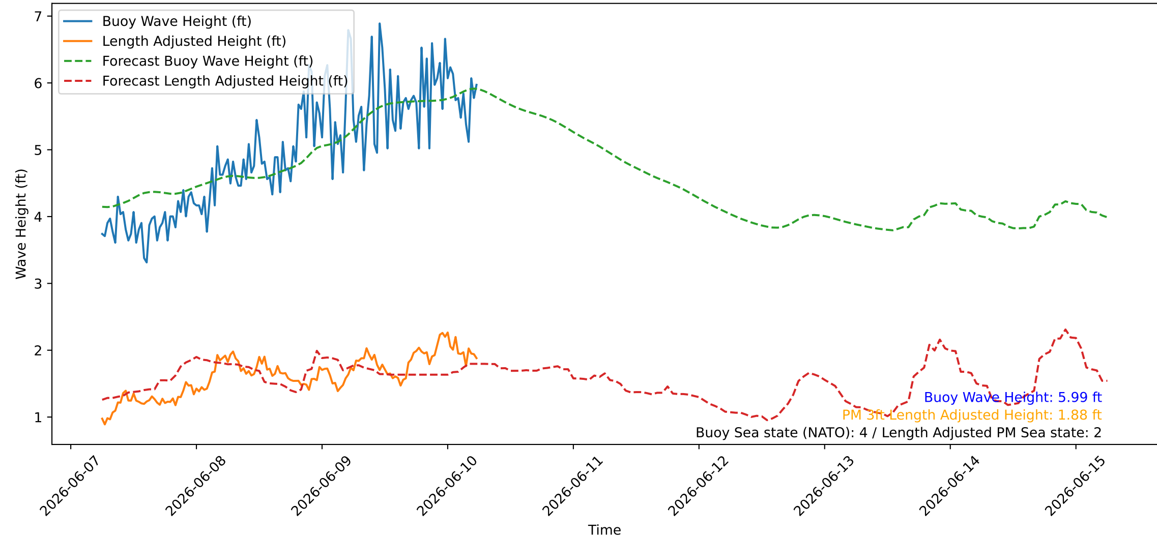
Wave Heights over Time for Green Beach at 2026-06-10 06:11:09
