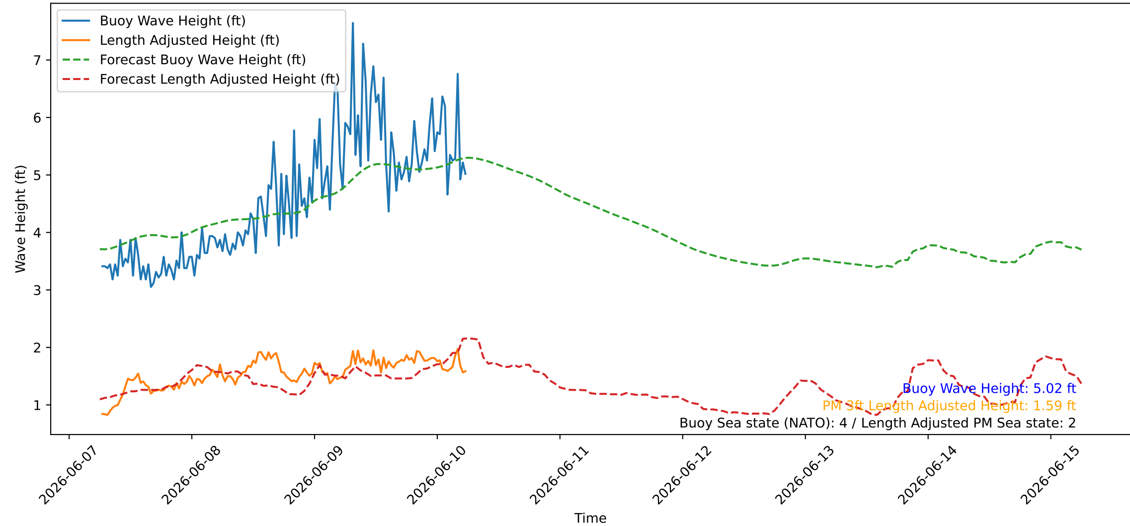
Wave Heights over Time for Red Beach at 2026-06-10 06:10:46
