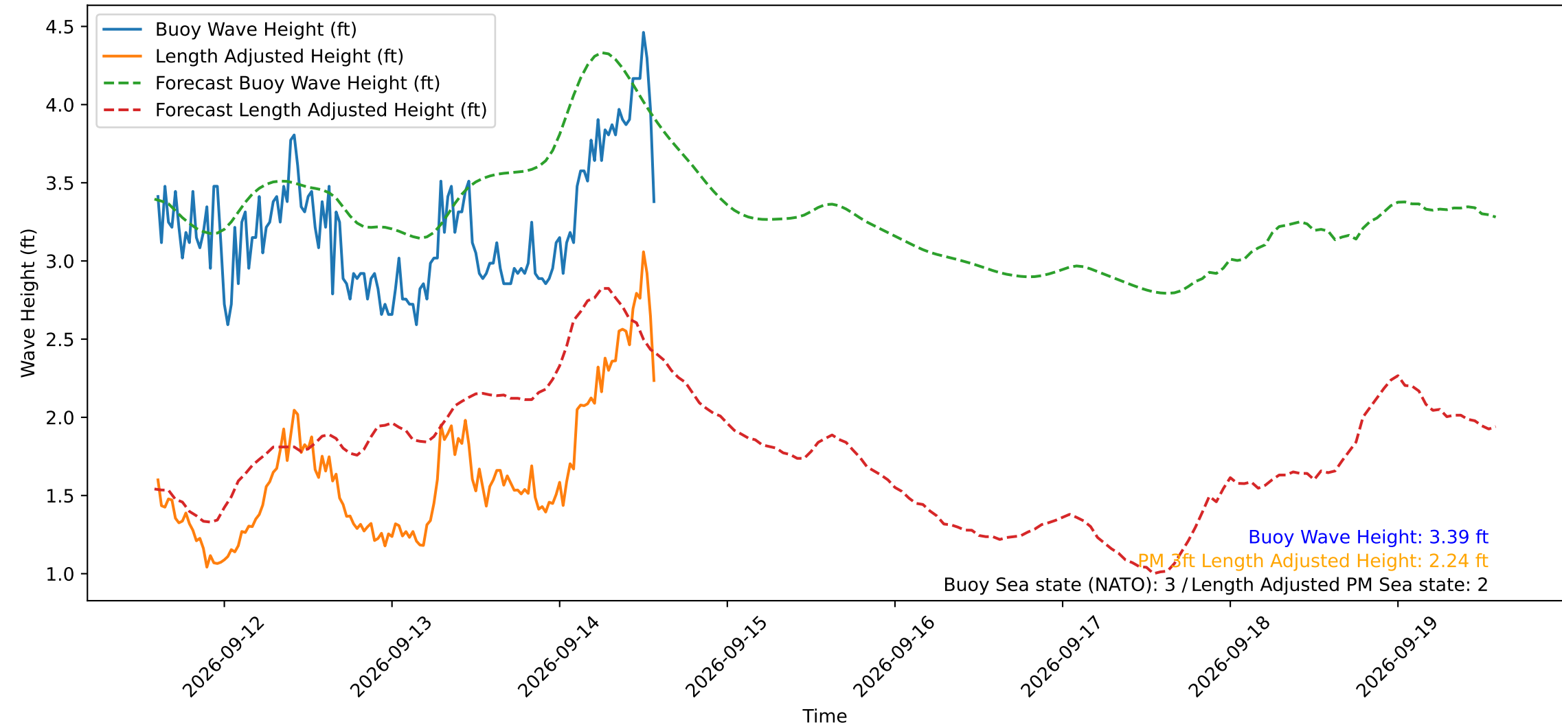
Wave Heights over Time for Oceanside Harbor at 2026-09-14 14:20:30
