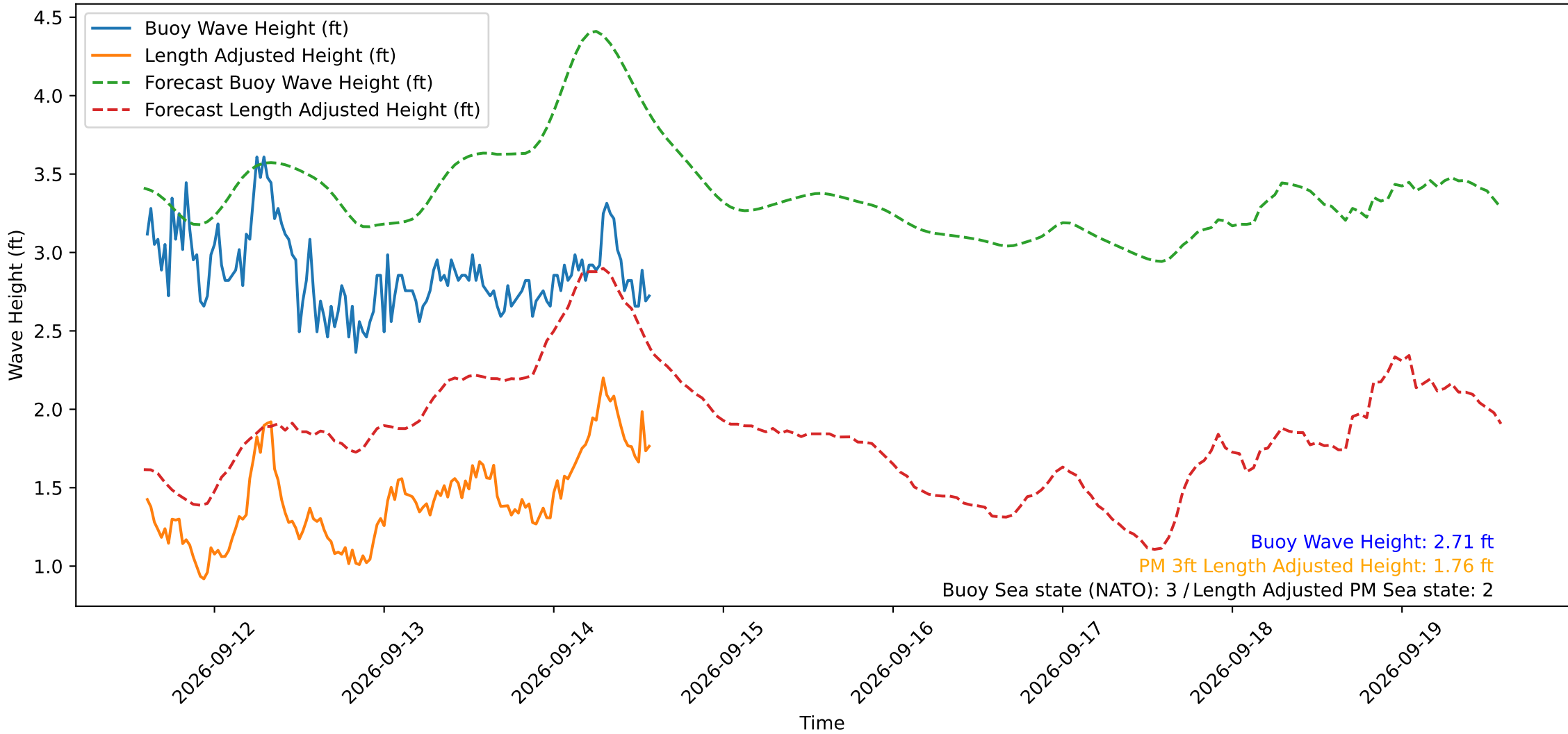
Wave Heights over Time for Green Beach at 2026-09-14 14:21:15
