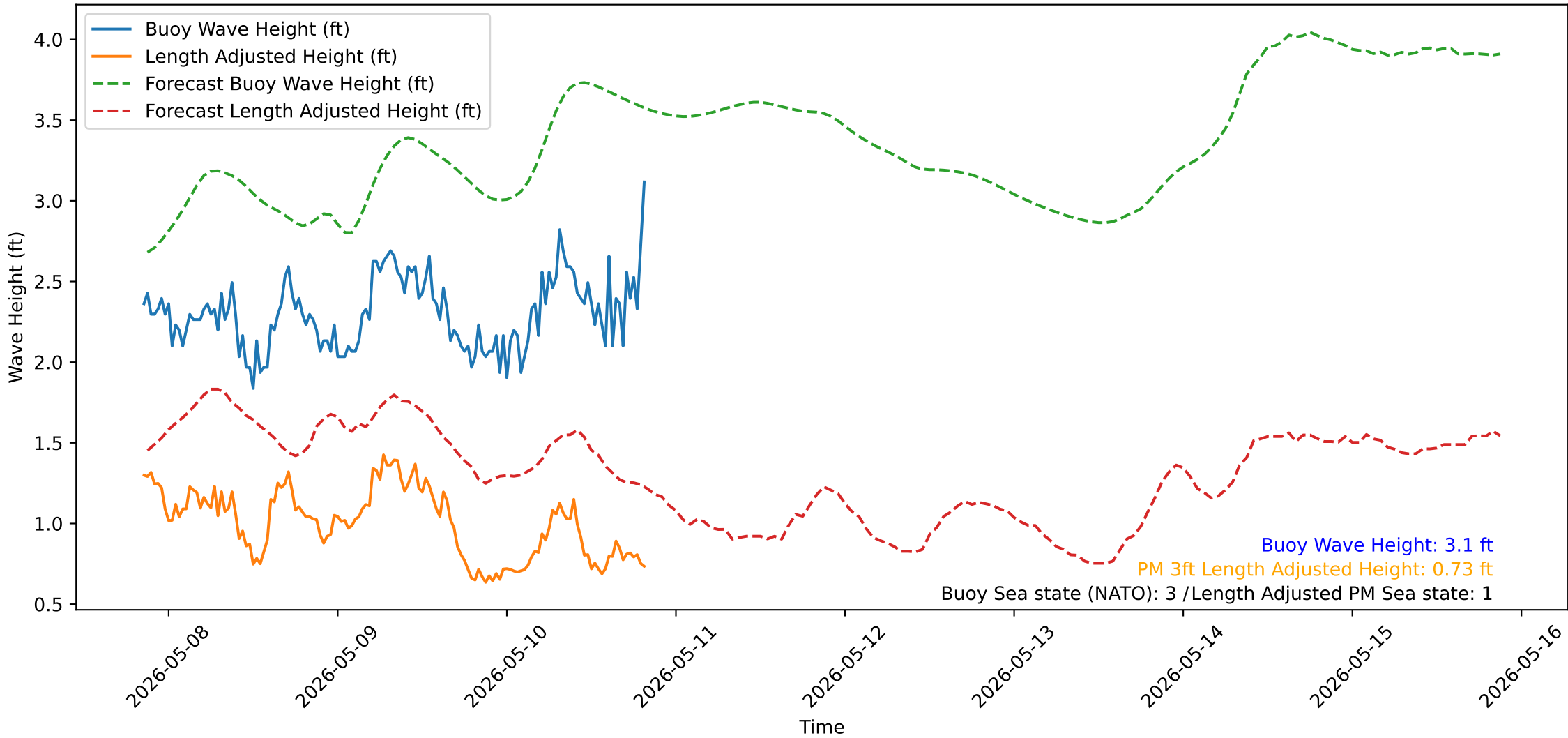
Wave Heights over Time for Green Beach at 2026-05-10 20:31:14
