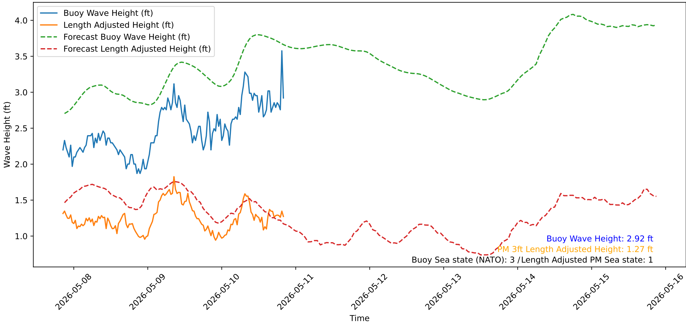
Wave Heights over Time for Oceanside Harbor at 2026-05-10 20:30:31
