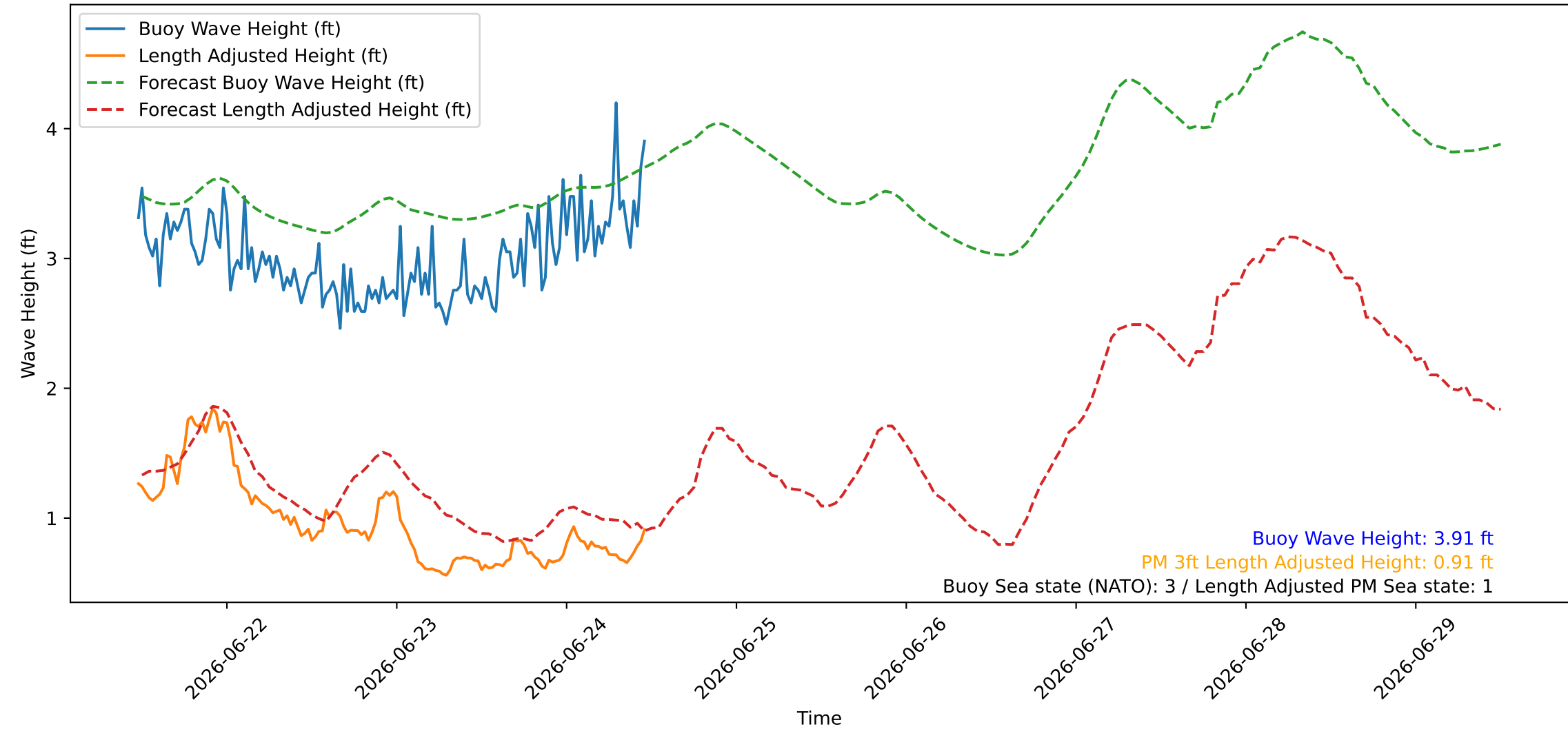
Wave Heights over Time for Green Beach at 2026-06-24 11:41:07
