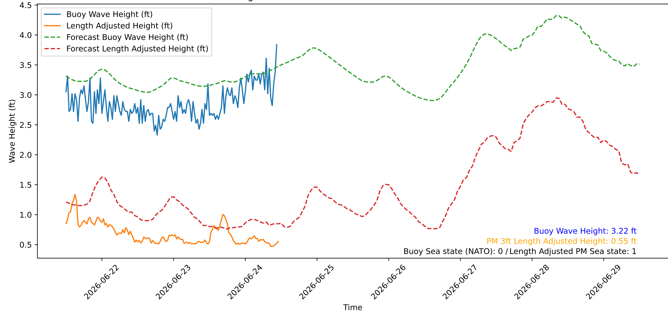
Wave Heights over Time for Red Beach at 2026-06-24 11:40:45
