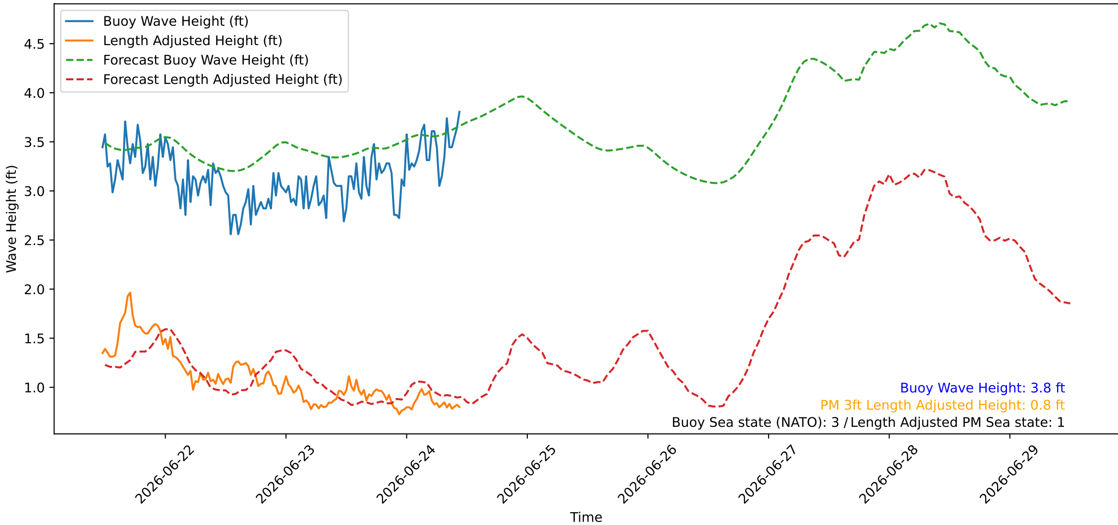
Wave Heights over Time for Oceanside Harbor at 2026-06-24 11:40:26
