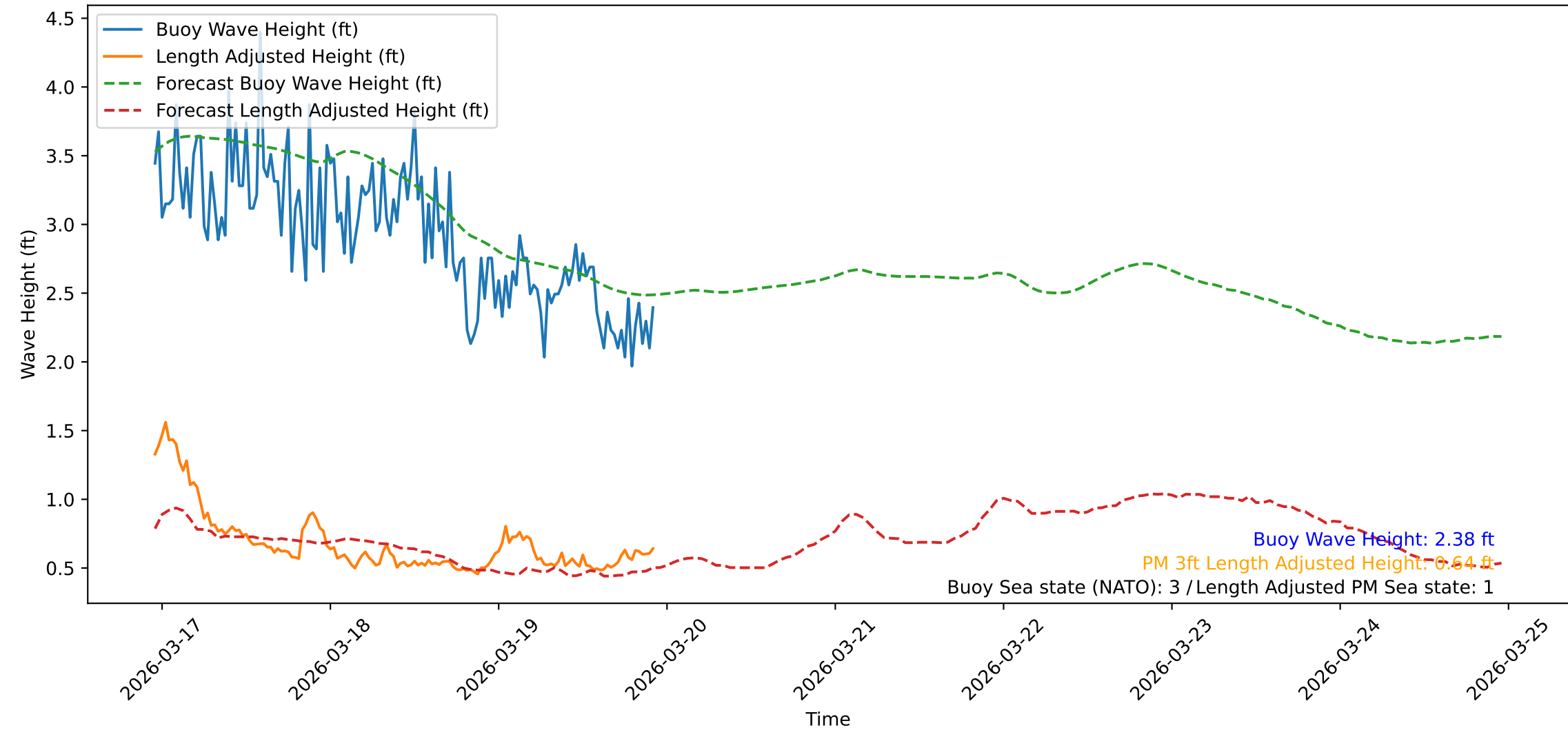
Wave Heights over Time for Oceanside Harbor at 2026-03-19 23:10:31
