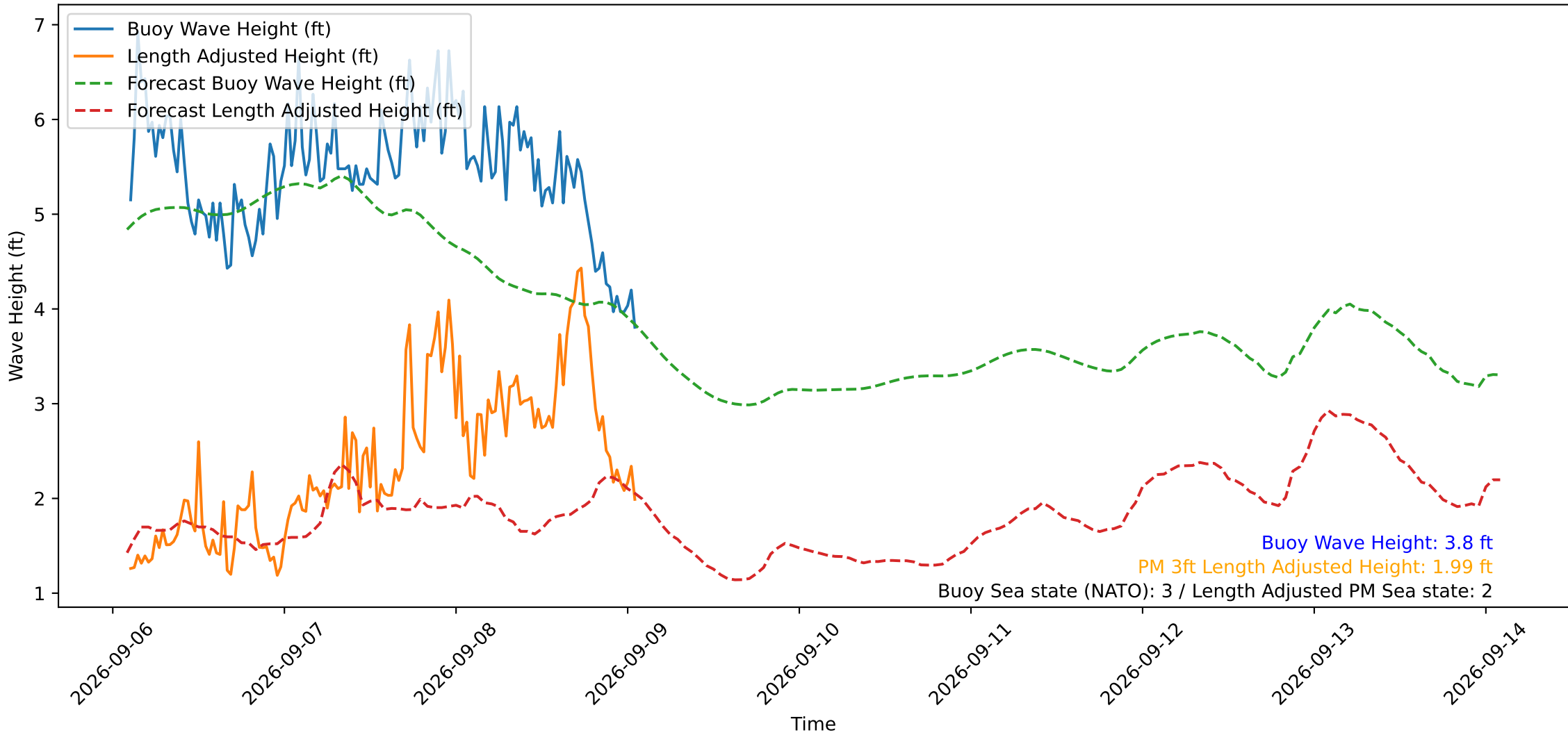
Wave Heights over Time for Red Beach at 2026-09-09 02:00:49
