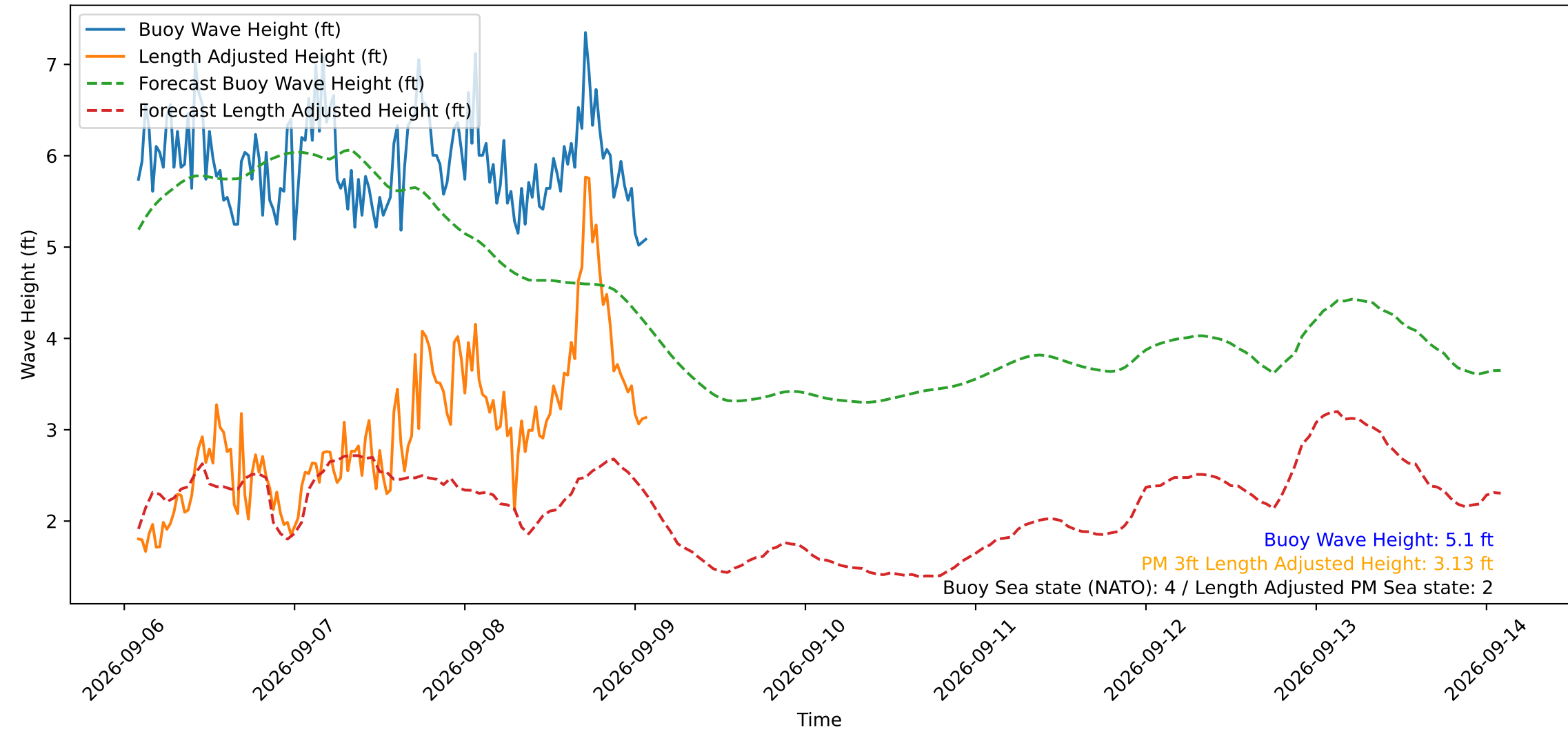
Wave Heights over Time for Oceanside Harbor at 2026-09-09 02:00:30
