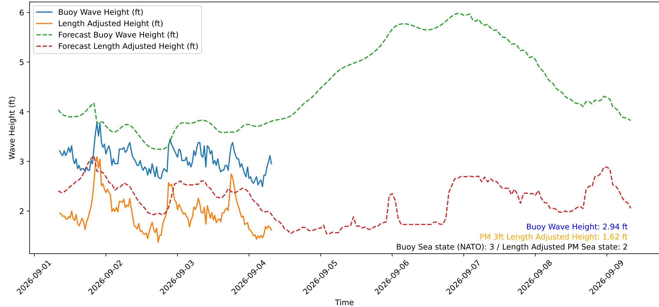
Wave Heights over Time for Green Beach at 2026-09-04 08:21:15
