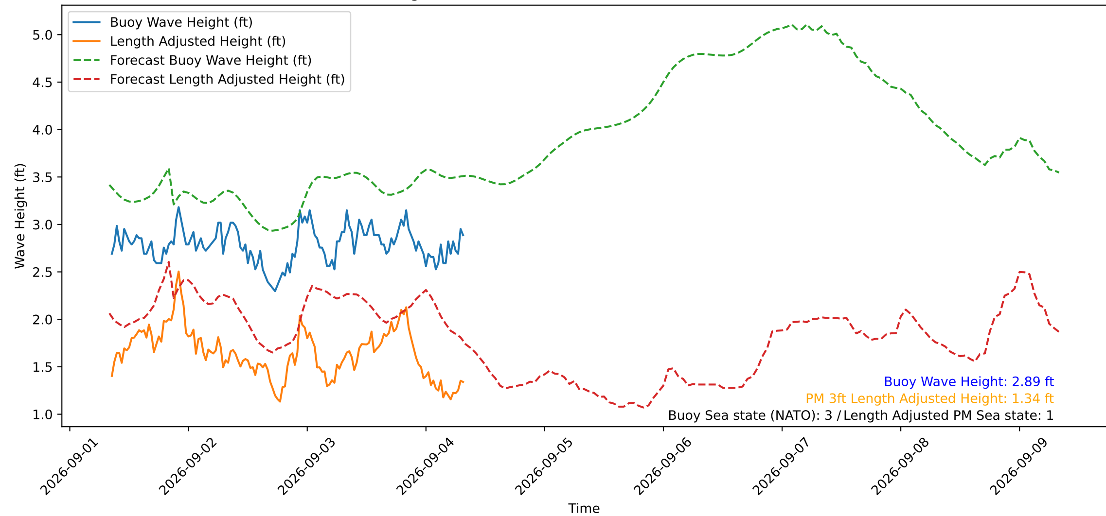
Wave Heights over Time for Red Beach at 2026-09-04 08:20:51
