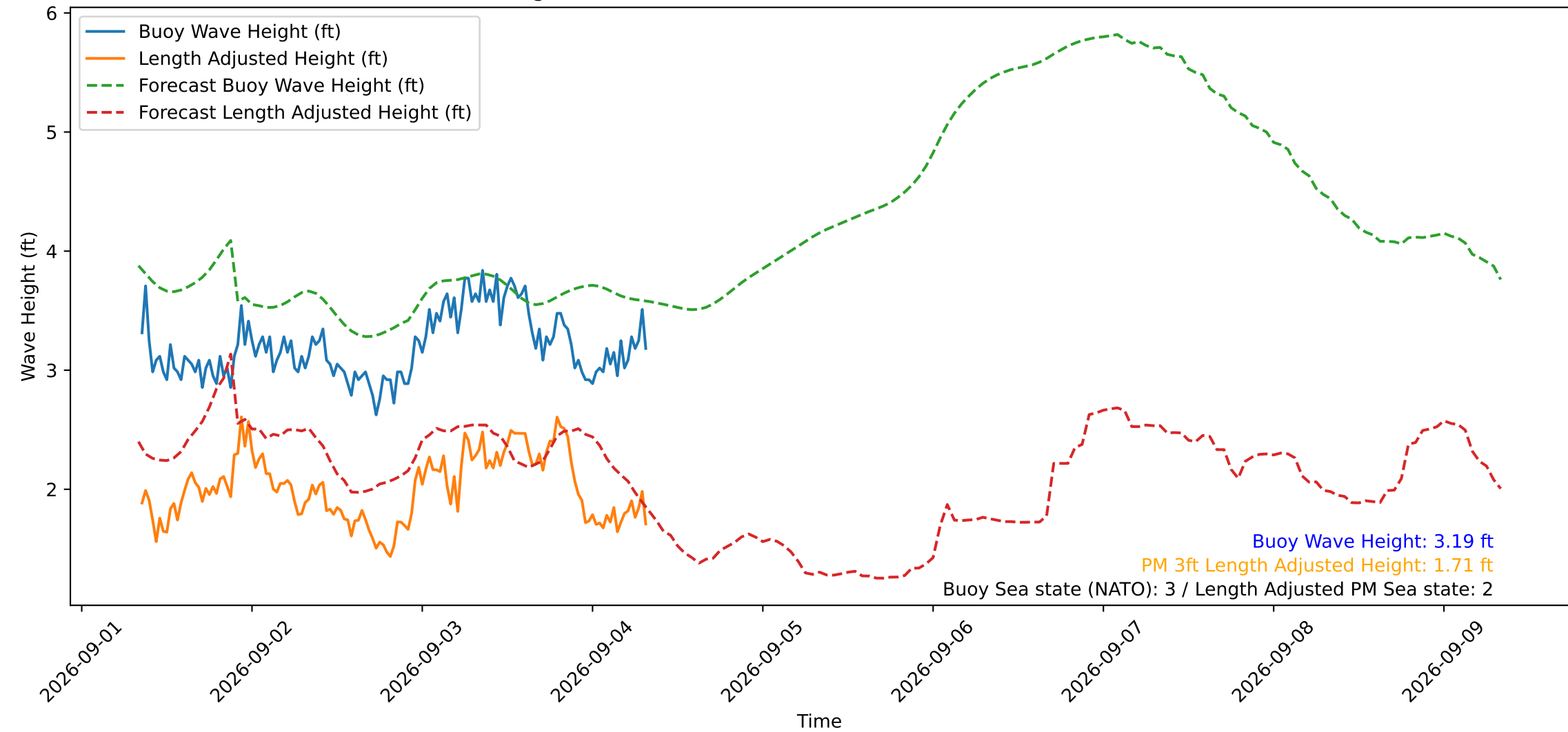
Wave Heights over Time for Oceanside Harbor at 2026-09-04 08:20:29
