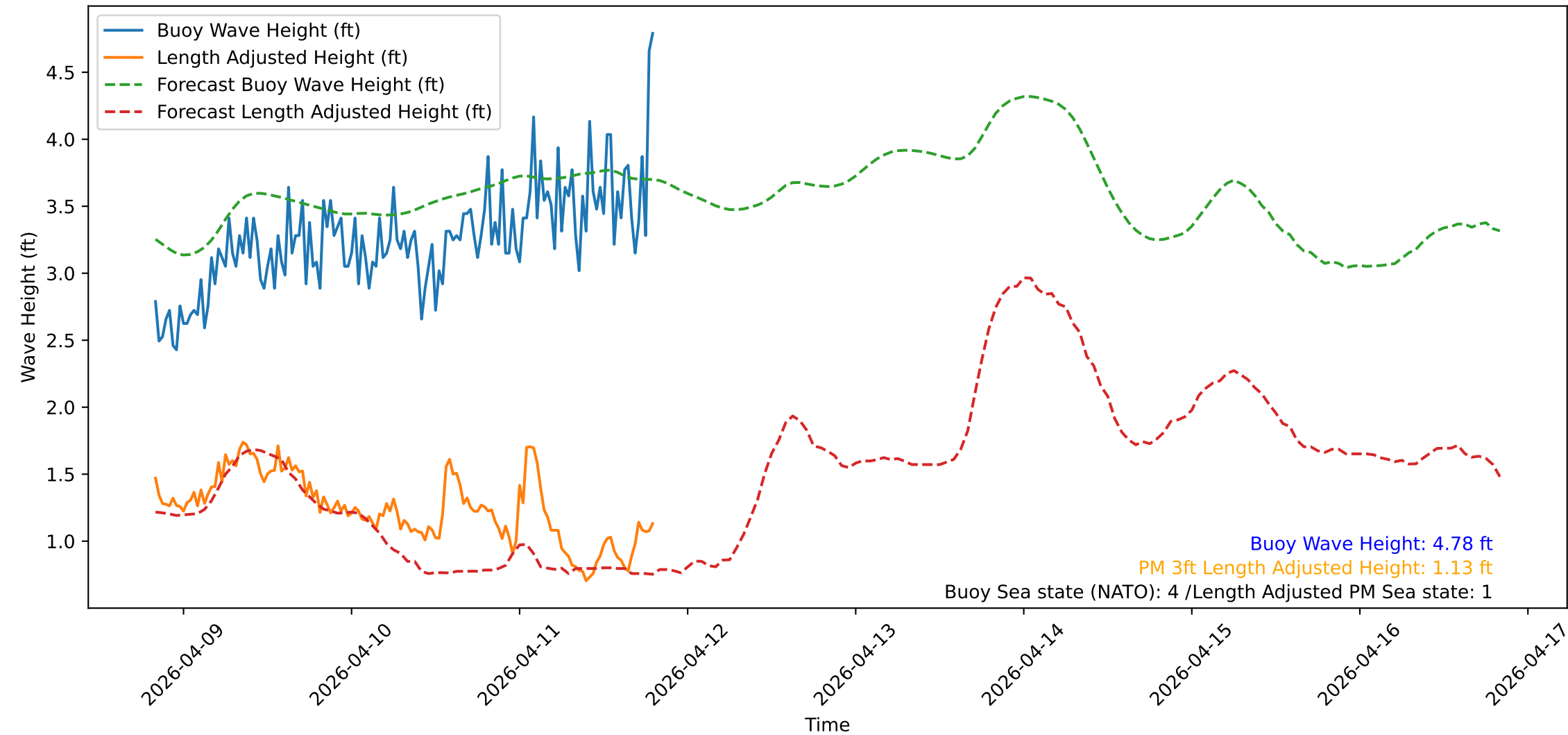
Wave Heights over Time for Oceanside Harbor at 2026-04-11 20:00:31
