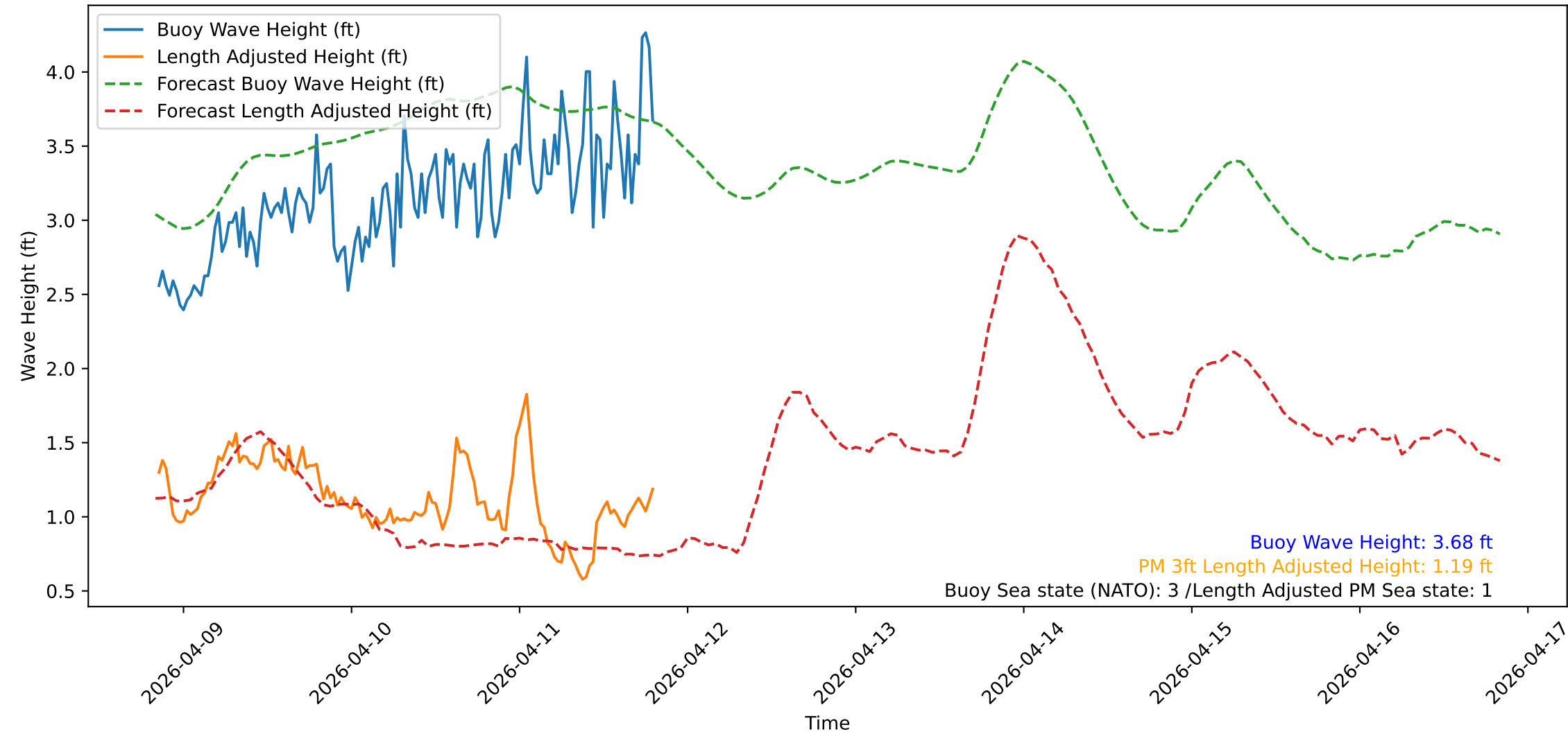
Wave Heights over Time for Red Beach at 2026-04-11 20:00:51
