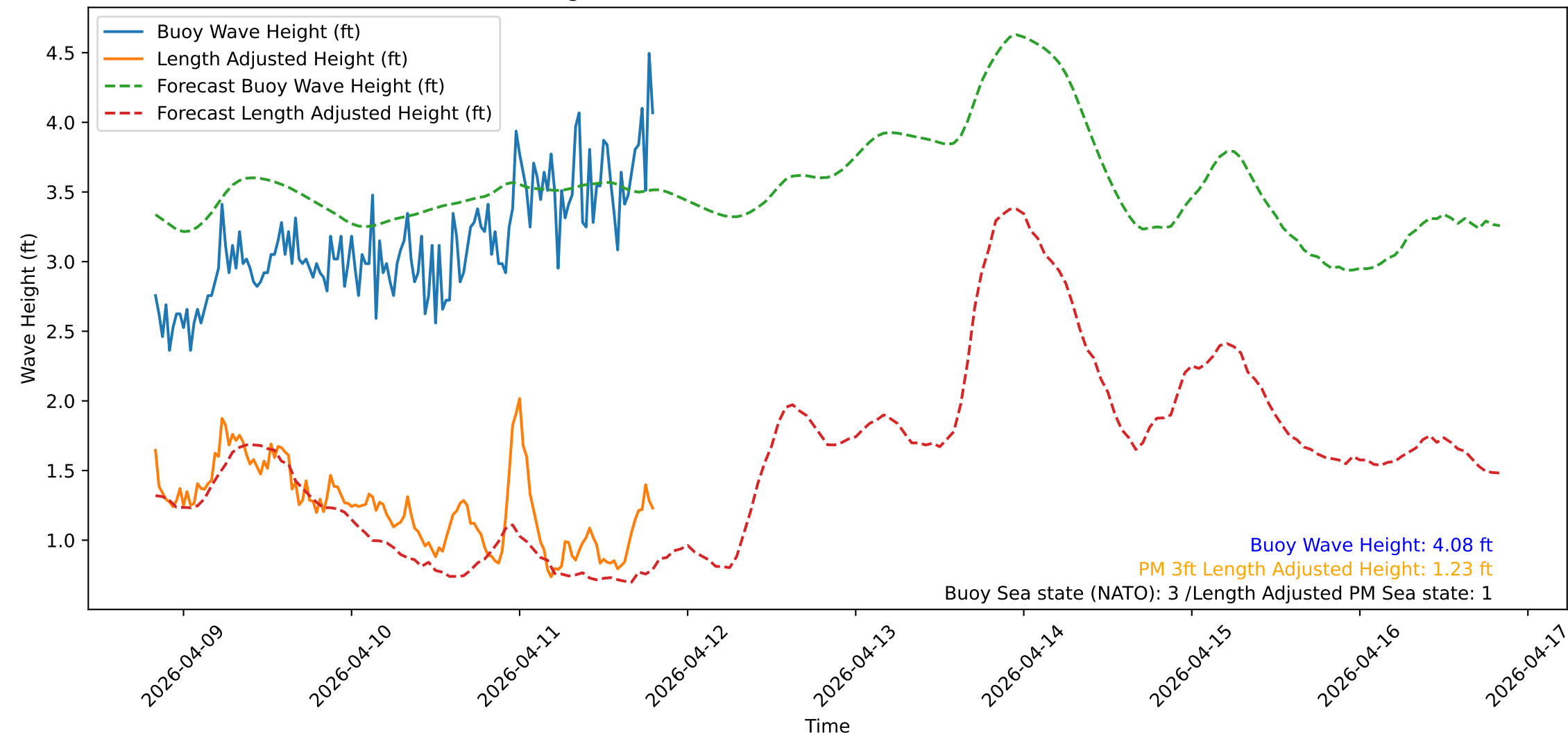
Wave Heights over Time for Green Beach at 2026-04-11 20:01:13
