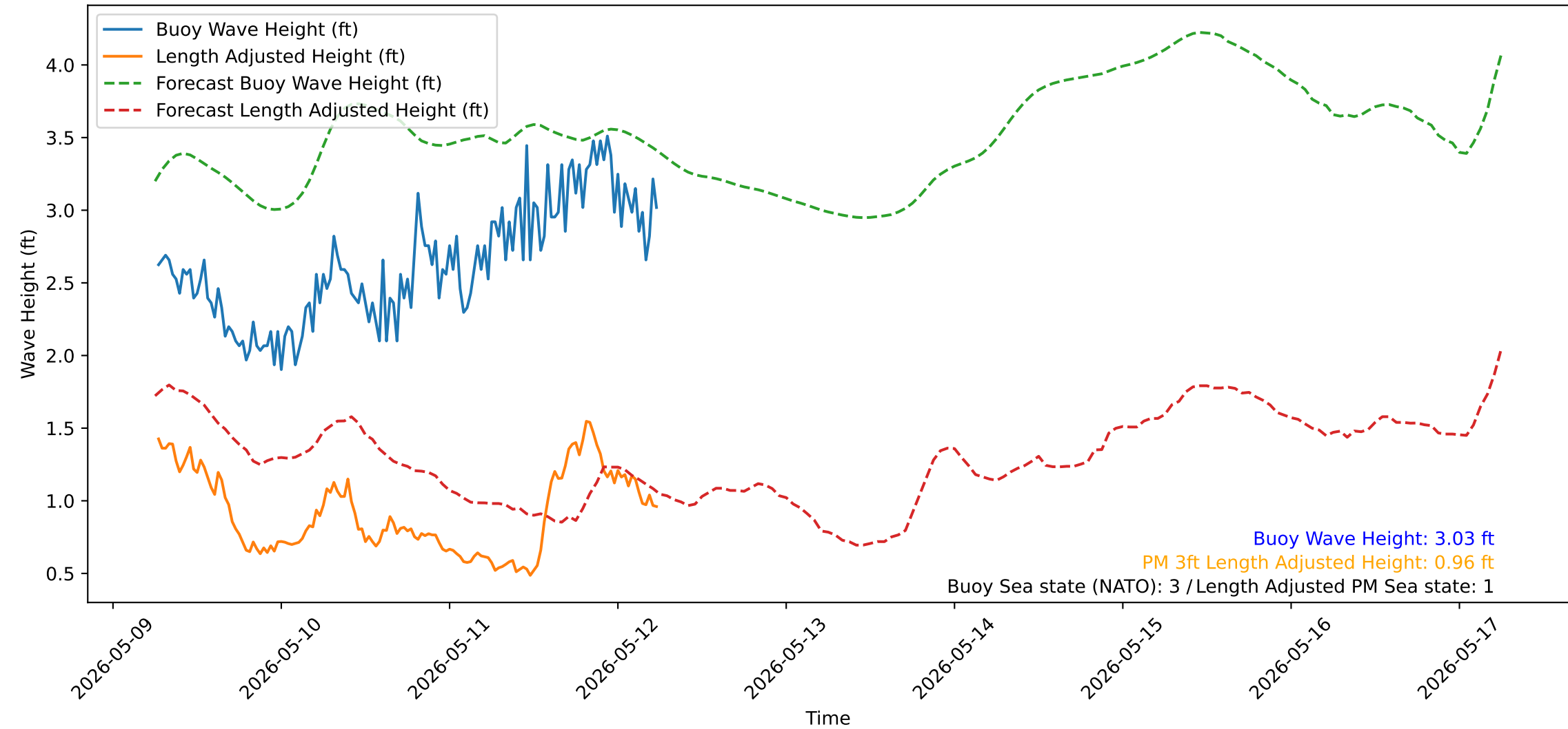
Wave Heights over Time for Green Beach at 2026-05-12 06:21:14
