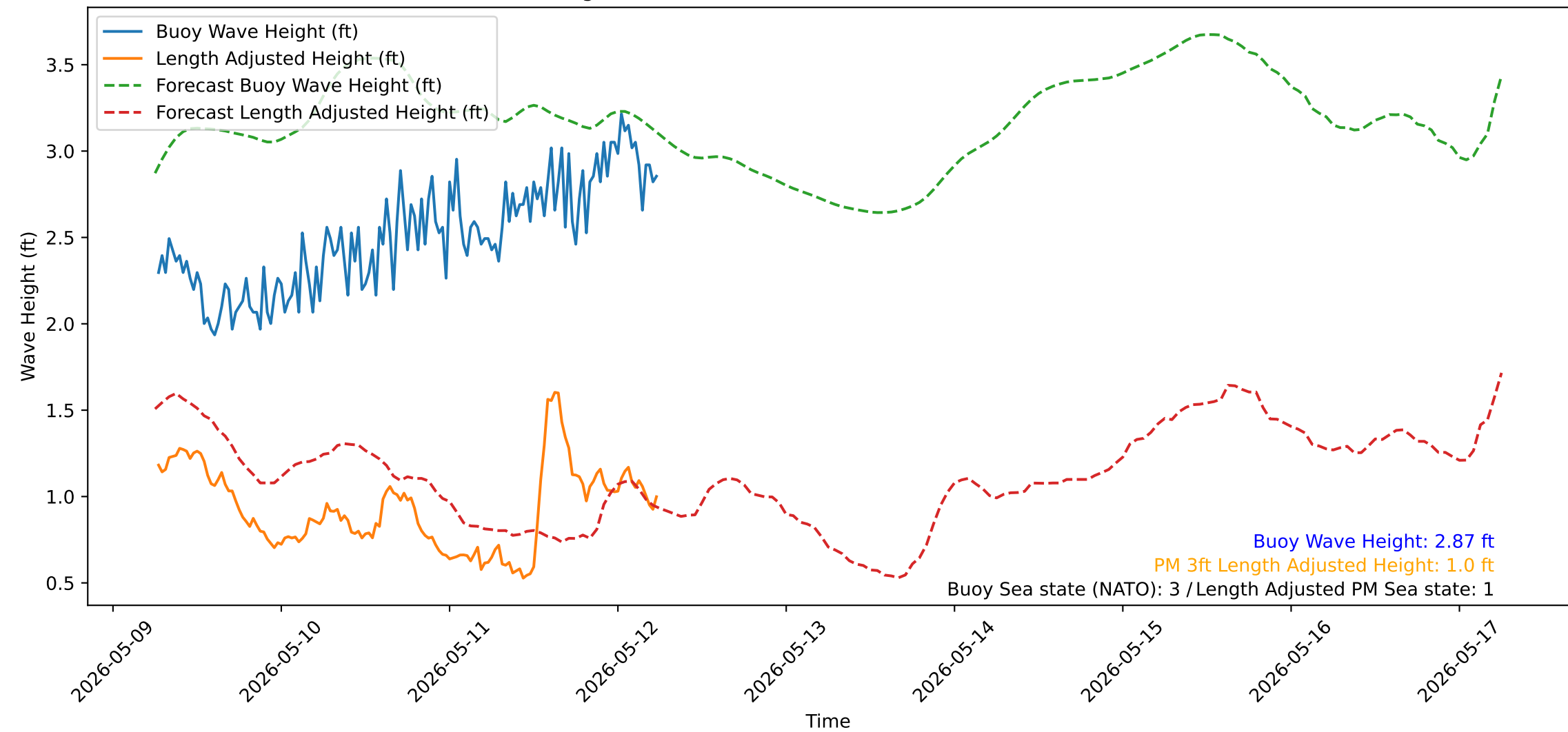
Wave Heights over Time for Red Beach at 2026-05-12 06:20:51
