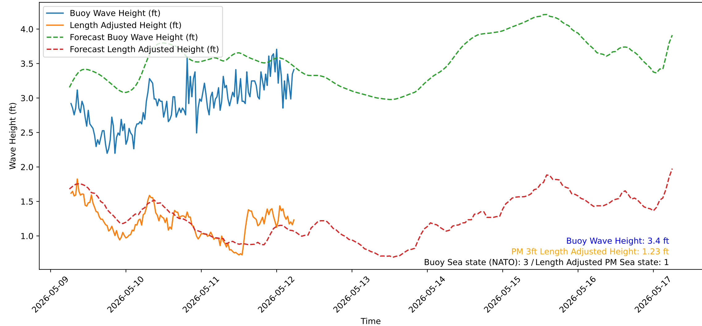
Wave Heights over Time for Oceanside Harbor at 2026-05-12 06:20:31
