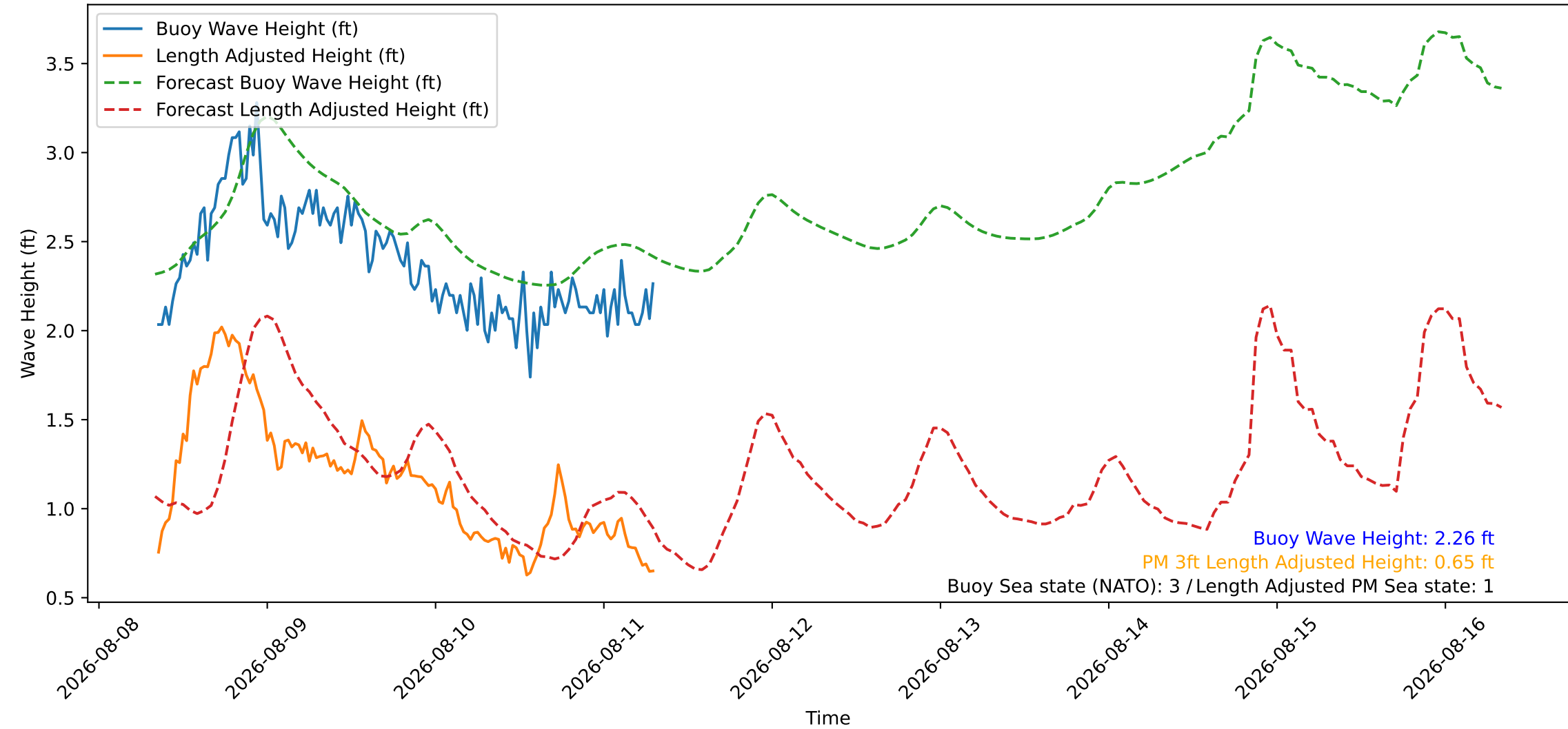
Wave Heights over Time for Red Beach at 2026-08-11 08:10:45
