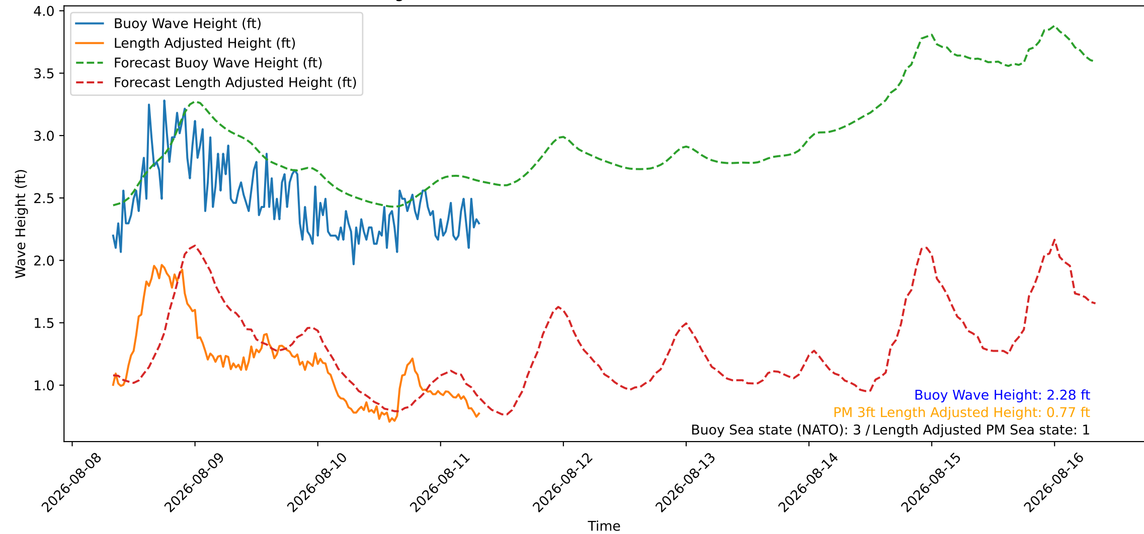
Wave Heights over Time for Oceanside Harbor at 2026-08-11 08:10:26
