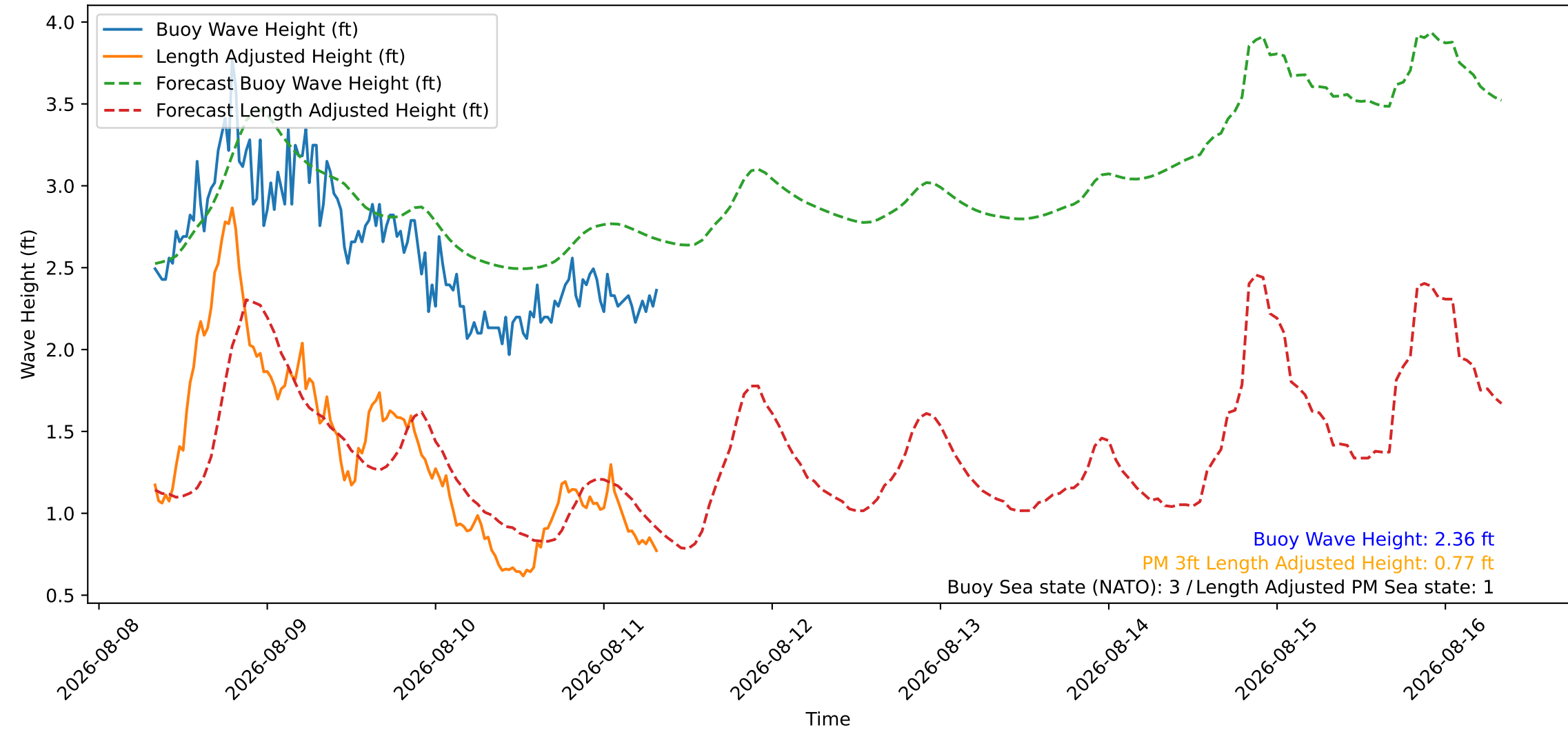
Wave Heights over Time for Green Beach at 2026-08-11 08:11:08
