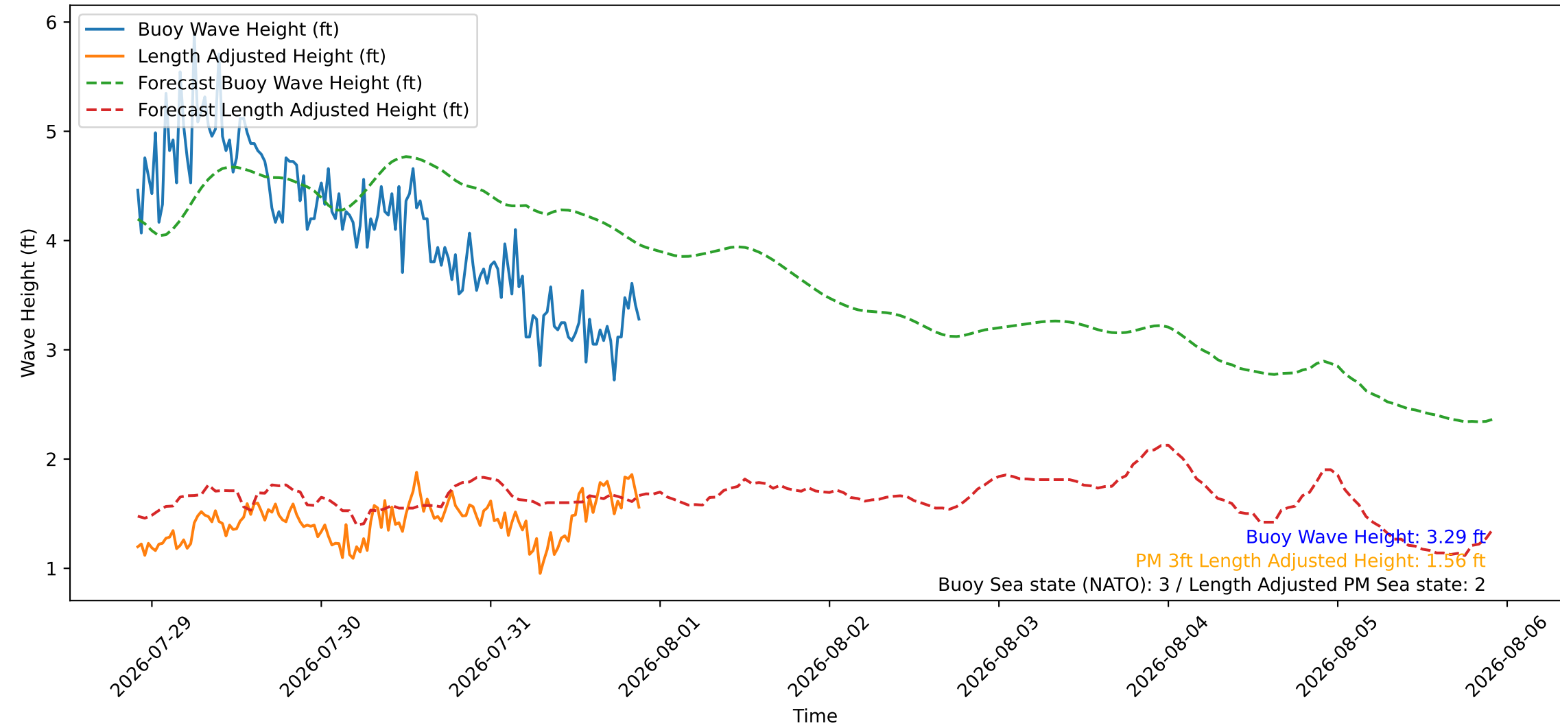
Wave Heights over Time for Oceanside Harbor at 2026-07-31 22:00:26
