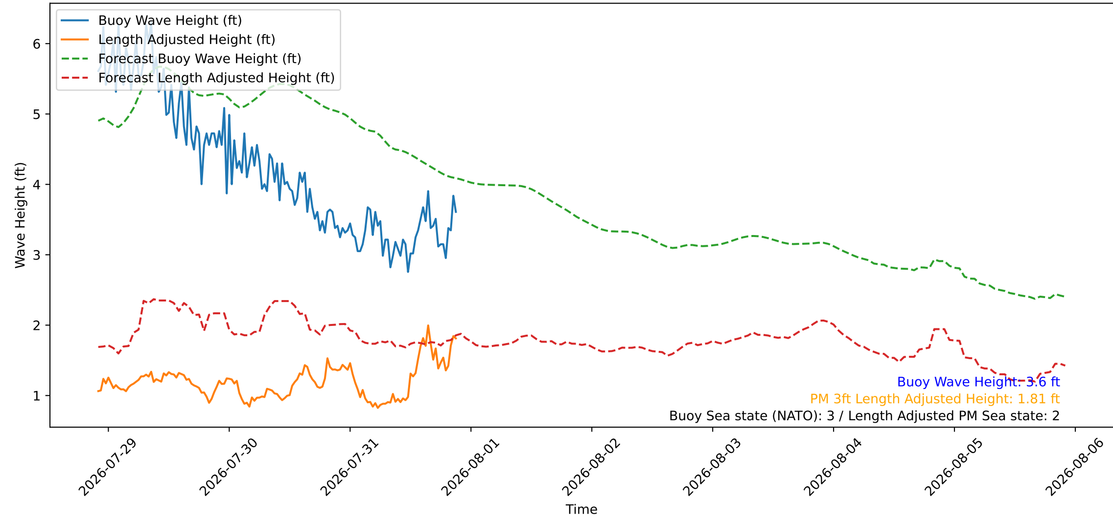
Wave Heights over Time for Green Beach at 2026-07-31 22:01:09
