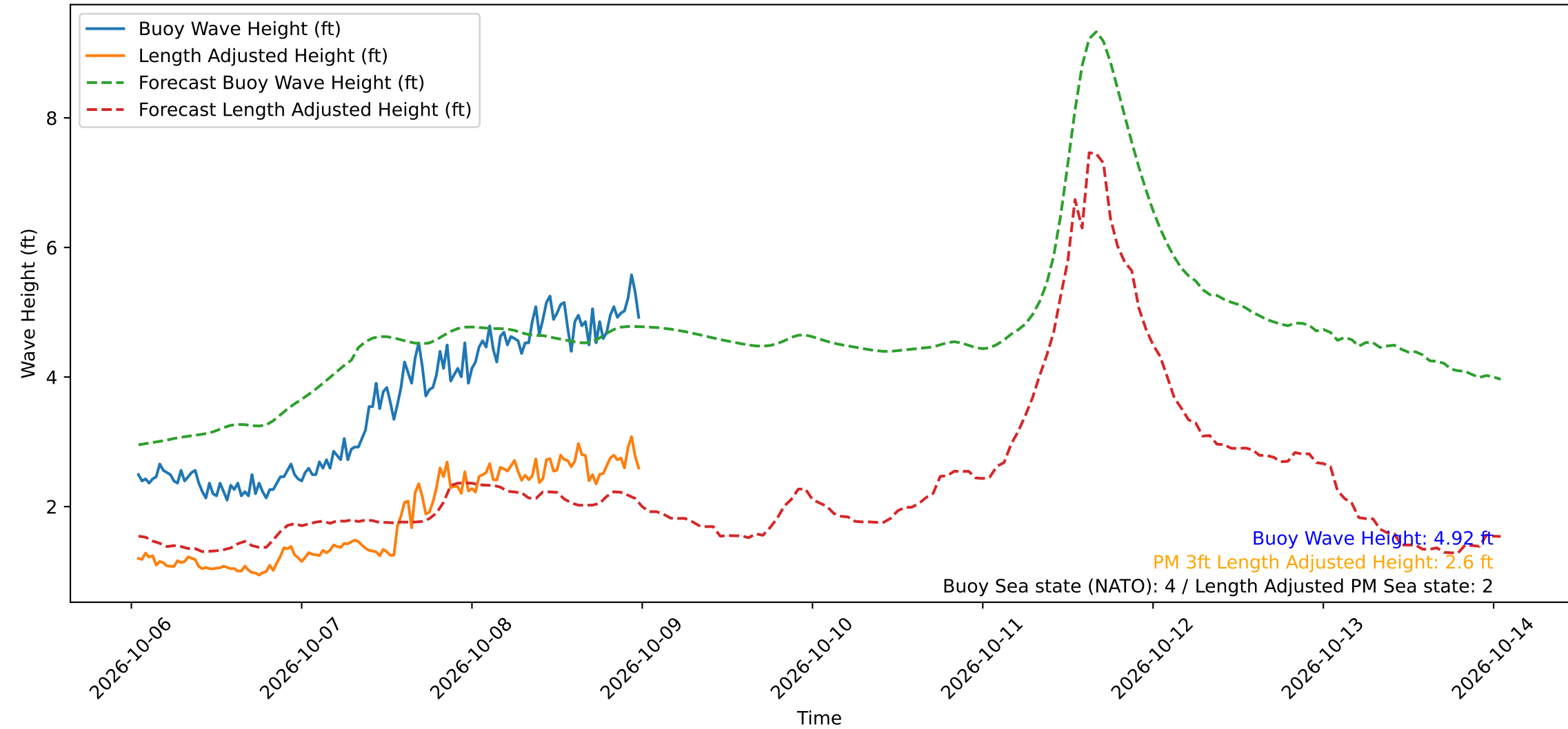
Wave Heights over Time for Green Beach at 2026-10-09 00:31:11
