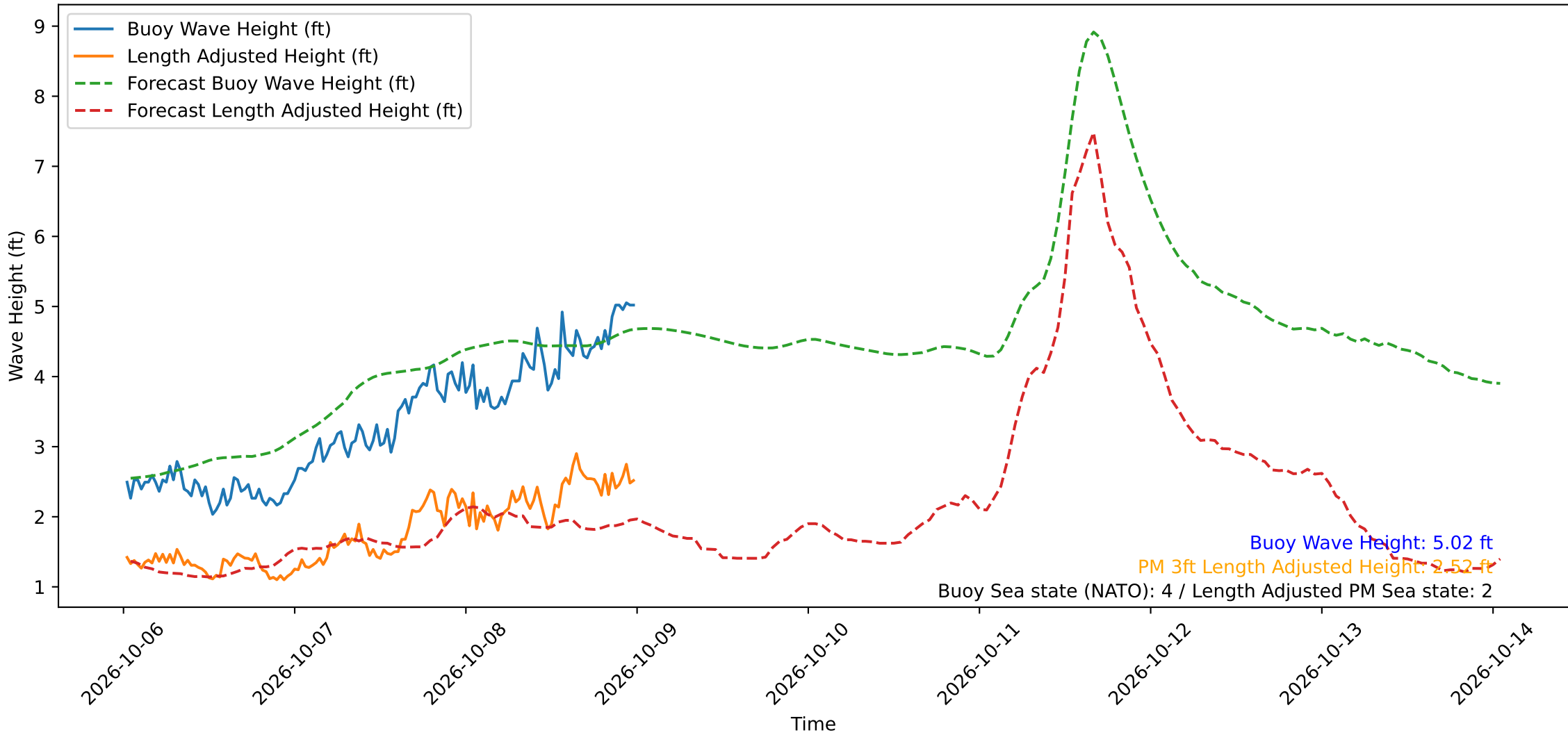
Wave Heights over Time for Oceanside Harbor at 2026-10-09 00:30:29
