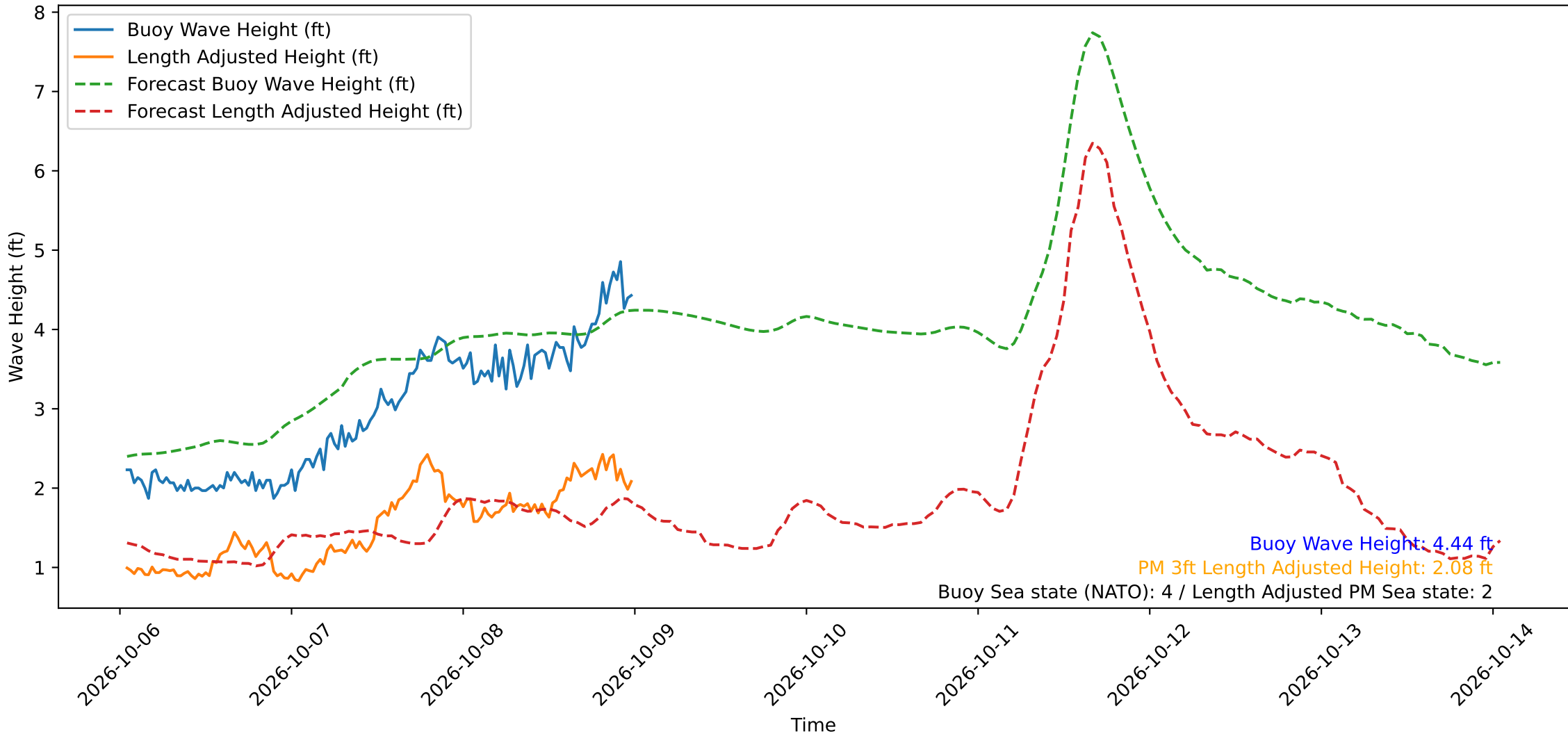
Wave Heights over Time for Red Beach at 2026-10-09 00:30:49
