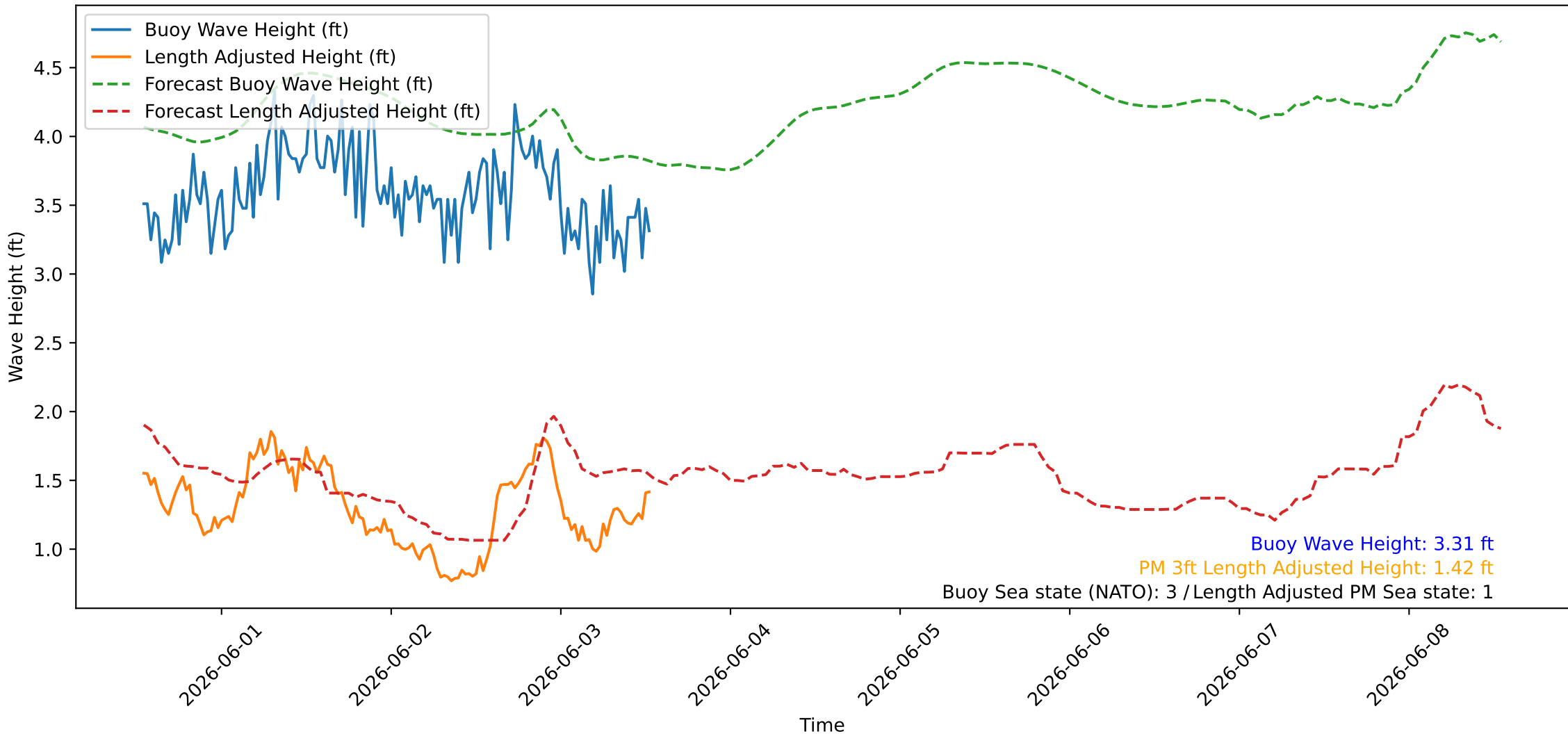
Wave Heights over Time for Green Beach at 2026-06-03 13:11:08
