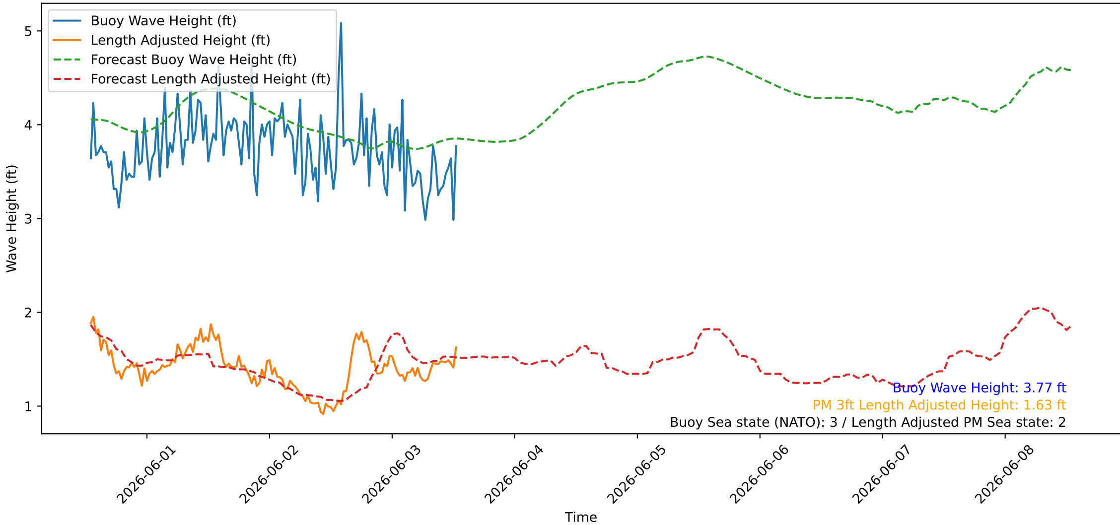
Wave Heights over Time for Oceanside Harbor at 2026-06-03 13:10:26
