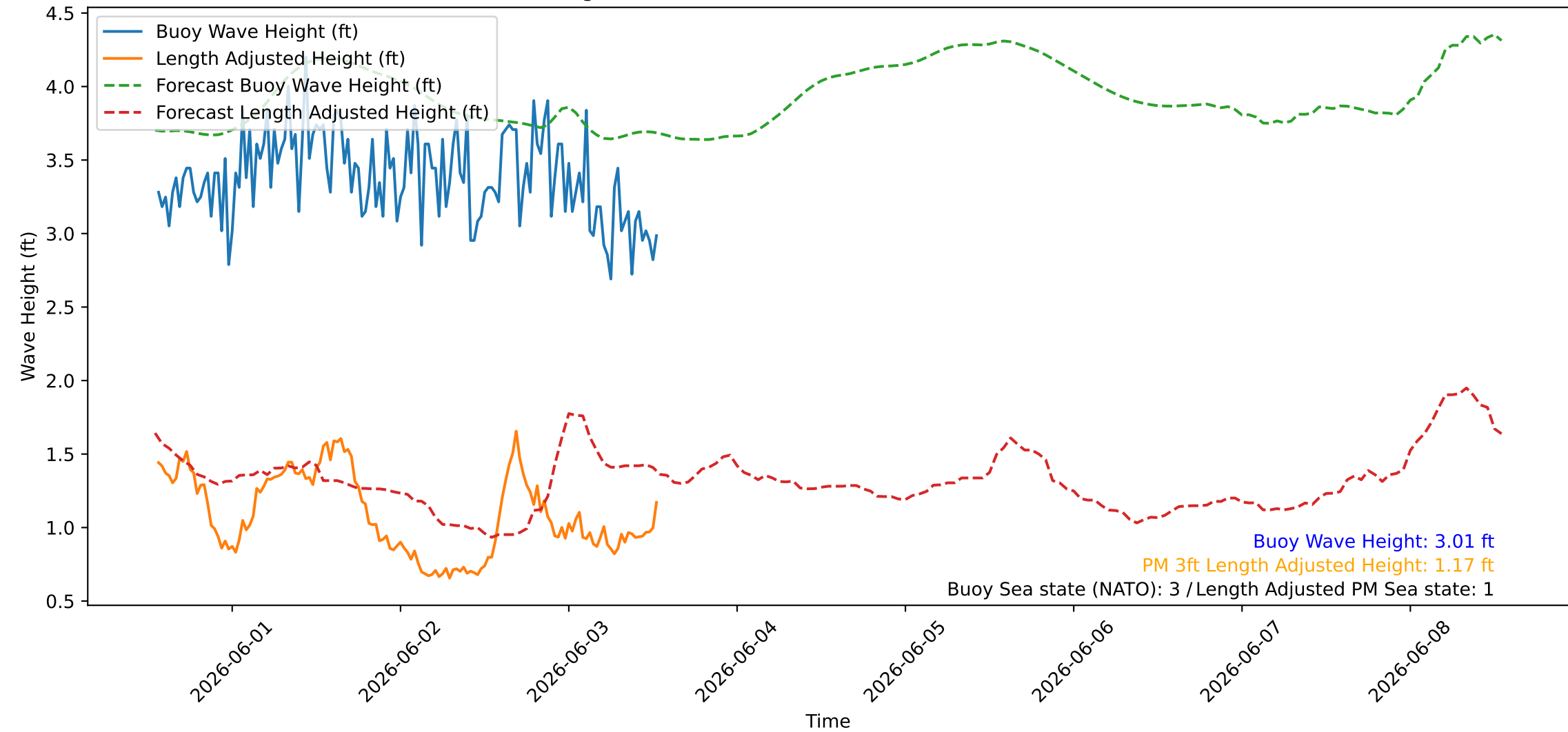
Wave Heights over Time for Red Beach at 2026-06-03 13:10:45
