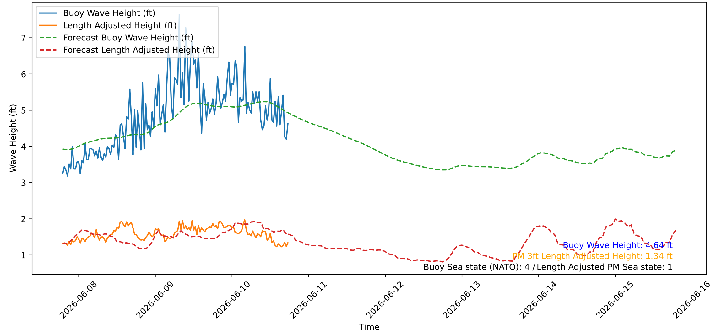
Wave Heights over Time for Red Beach at 2026-06-10 18:30:47
