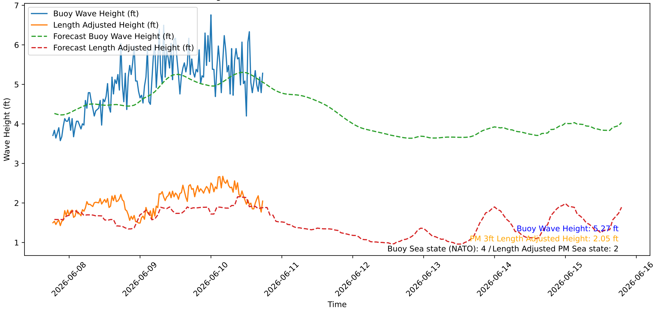
Wave Heights over Time for Oceanside Harbor at 2026-06-10 18:30:27
