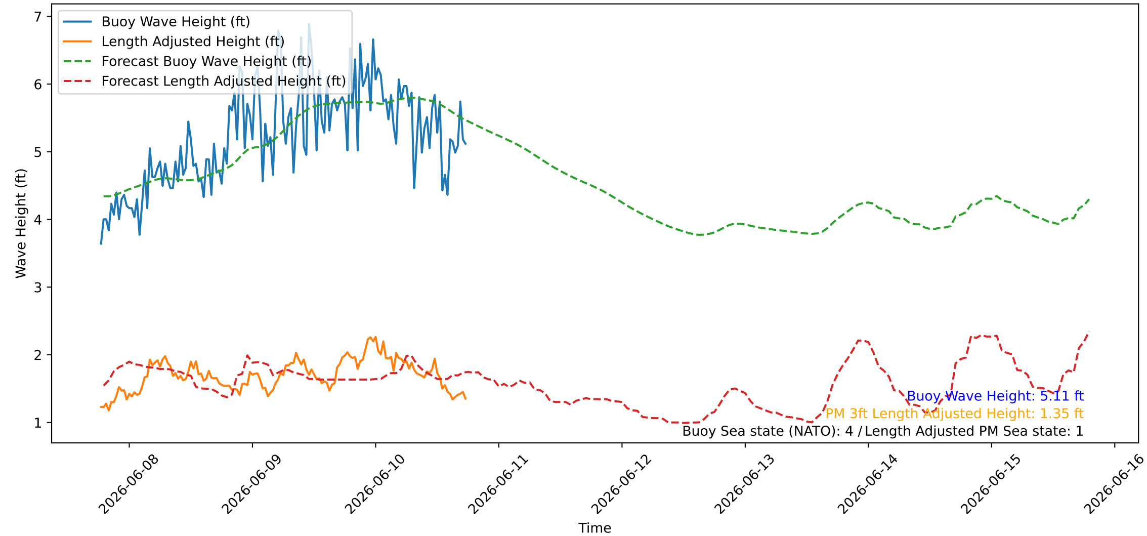
Wave Heights over Time for Green Beach at 2026-06-10 18:31:10
