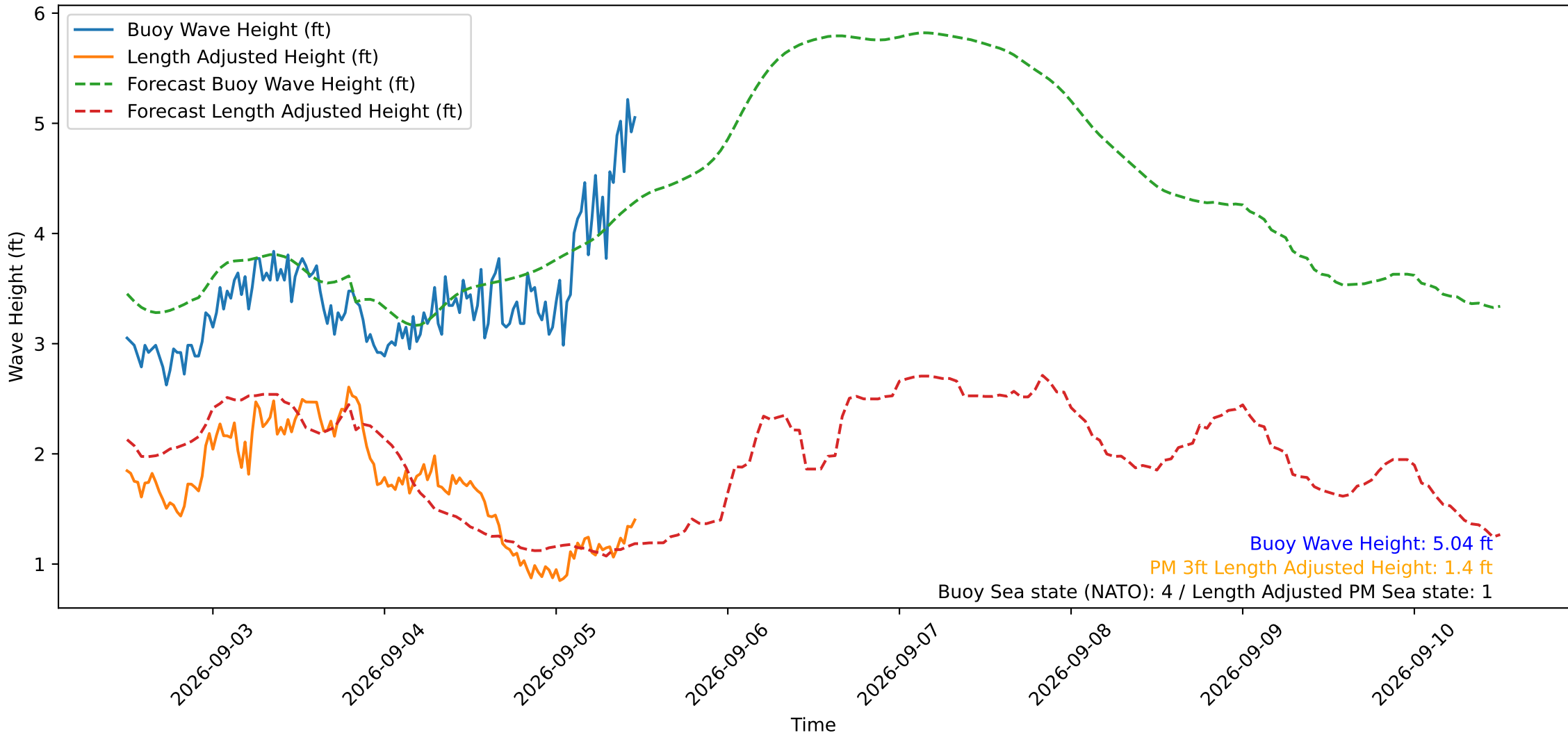
Wave Heights over Time for Oceanside Harbor at 2026-09-05 12:00:30
