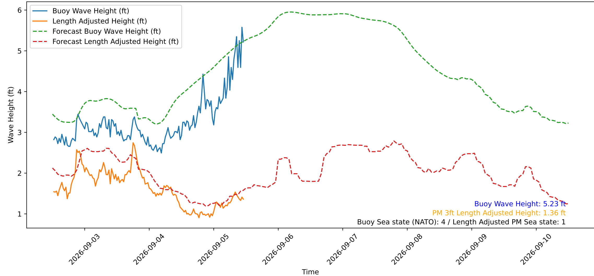
Wave Heights over Time for Green Beach at 2026-09-05 12:01:12
