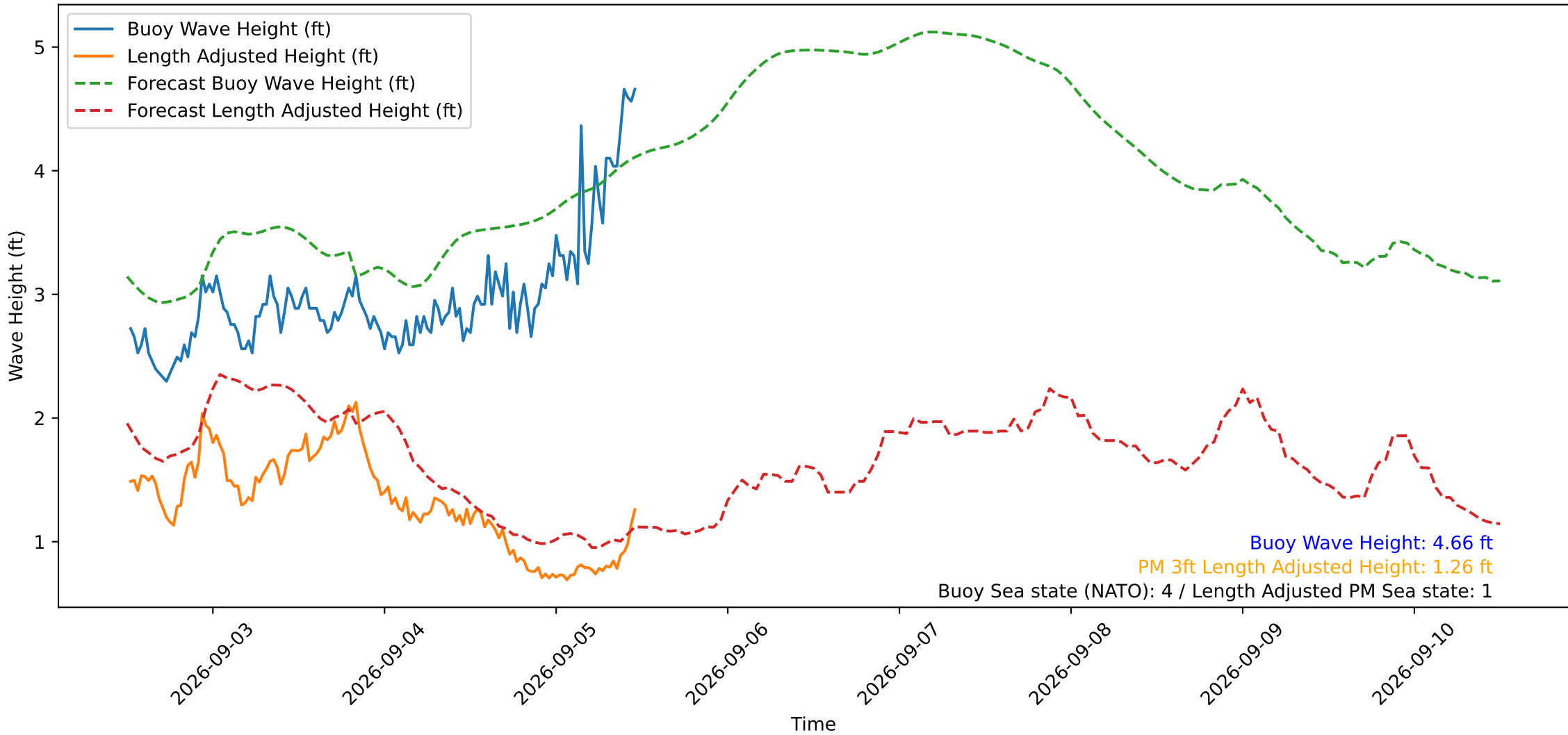
Wave Heights over Time for Red Beach at 2026-09-05 12:00:49
