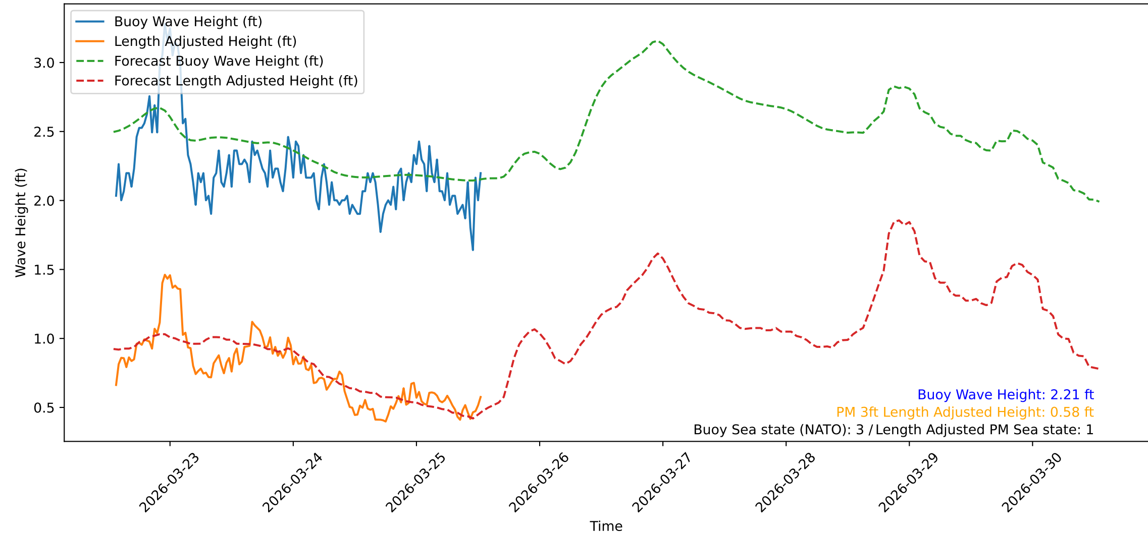
Wave Heights over Time for Green Beach at 2026-03-25 13:21:09
