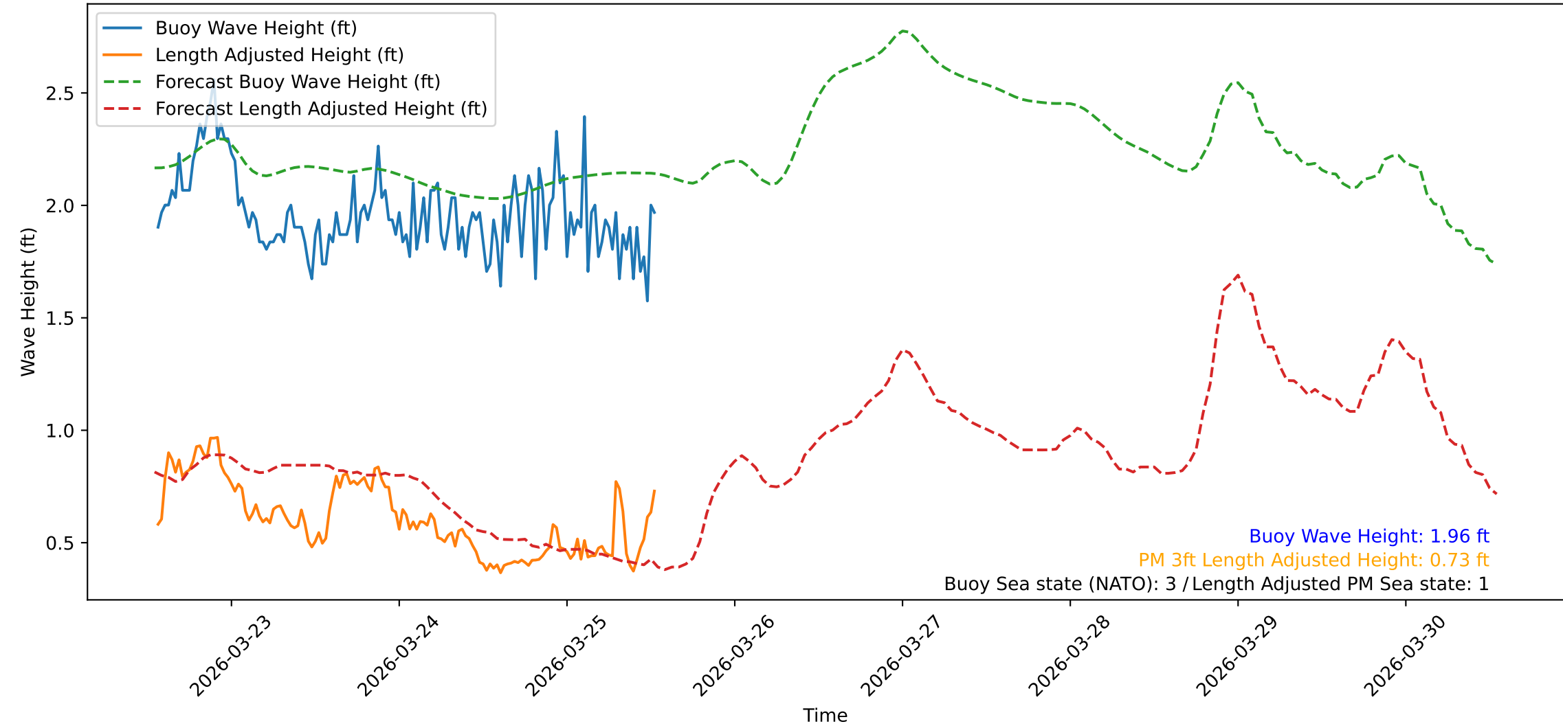
Wave Heights over Time for Red Beach at 2026-03-25 13:20:47
