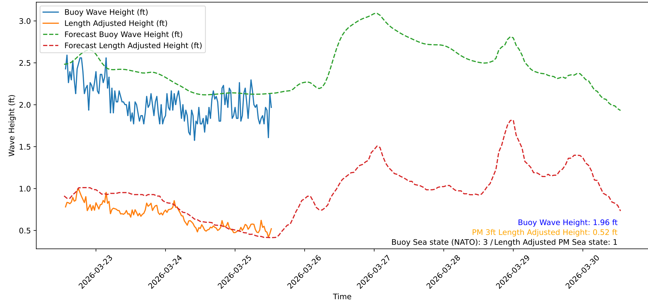
Wave Heights over Time for Oceanside Harbor at 2026-03-25 13:20:31
