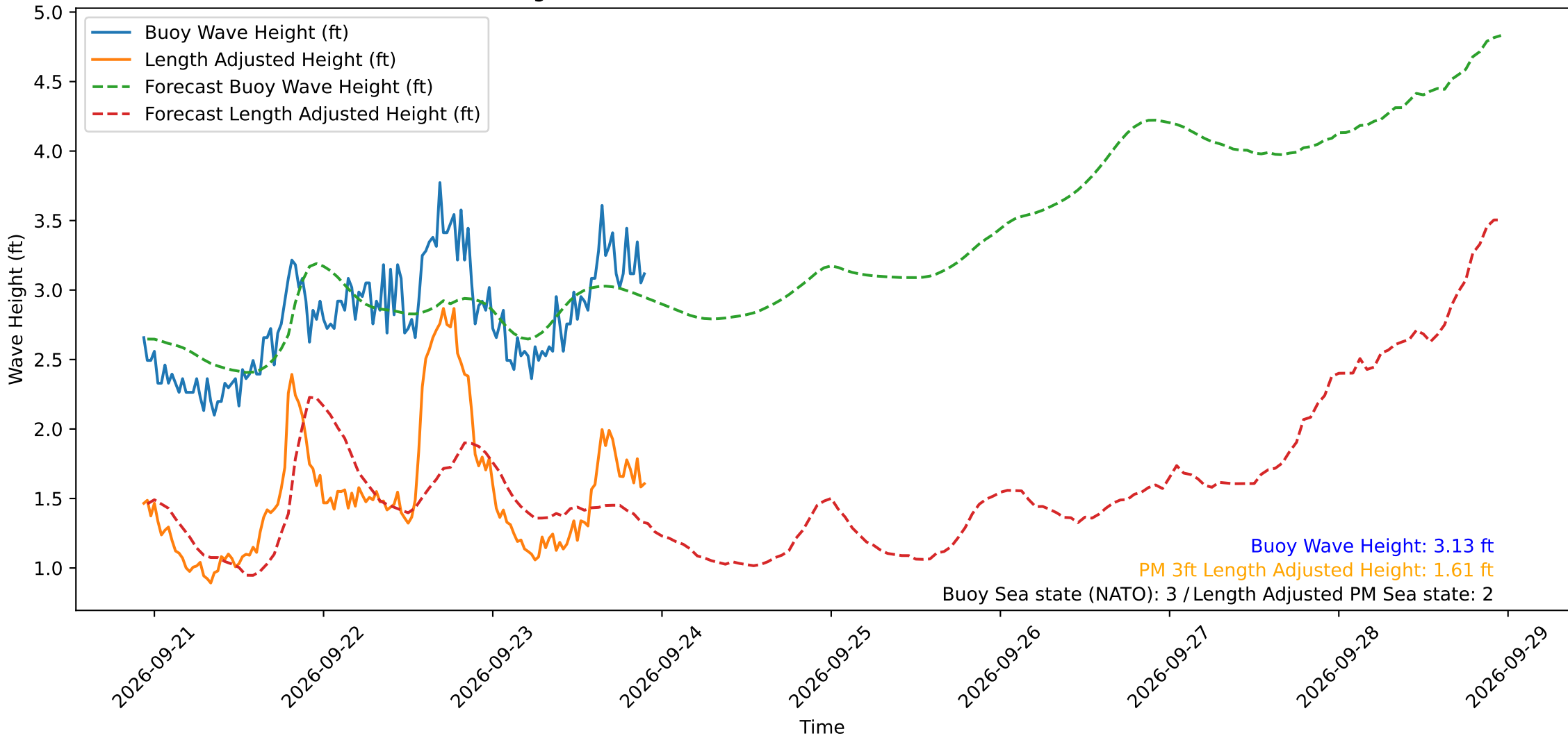
Wave Heights over Time for Oceanside Harbor at 2026-09-23 22:30:31
