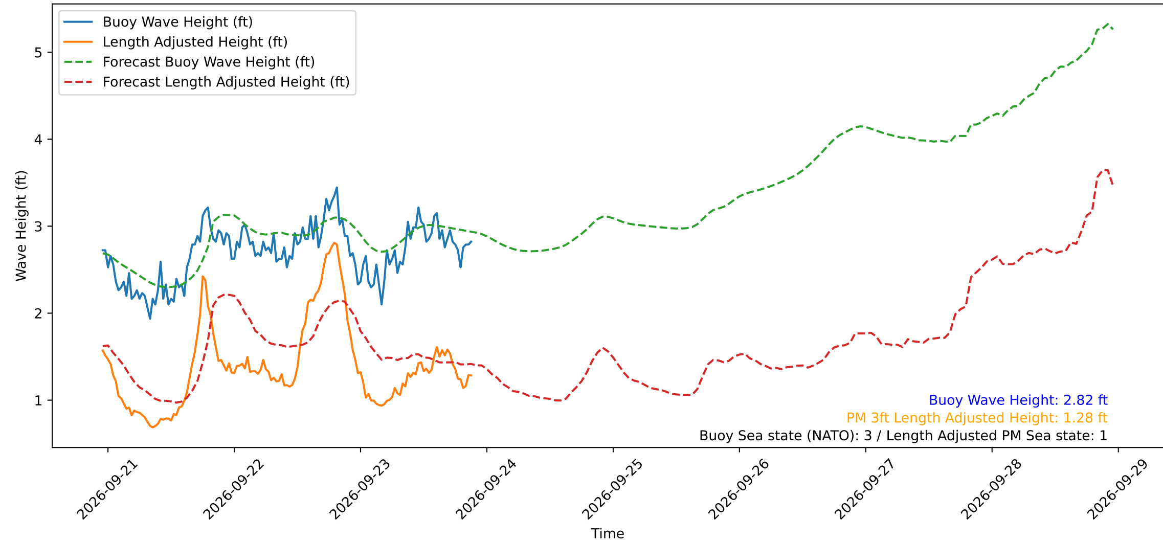
Wave Heights over Time for Green Beach at 2026-09-23 22:31:13
