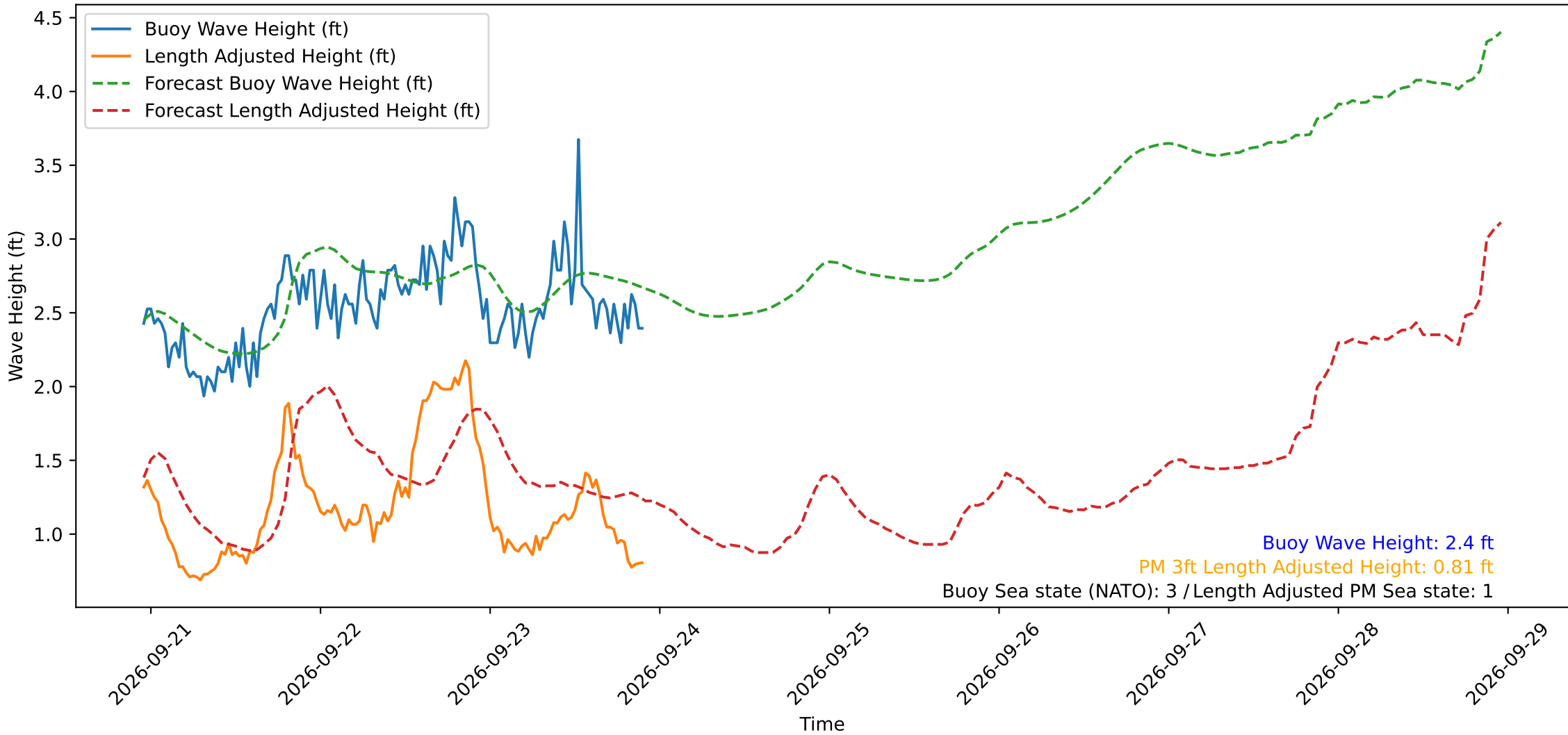
Wave Heights over Time for Red Beach at 2026-09-23 22:30:51
