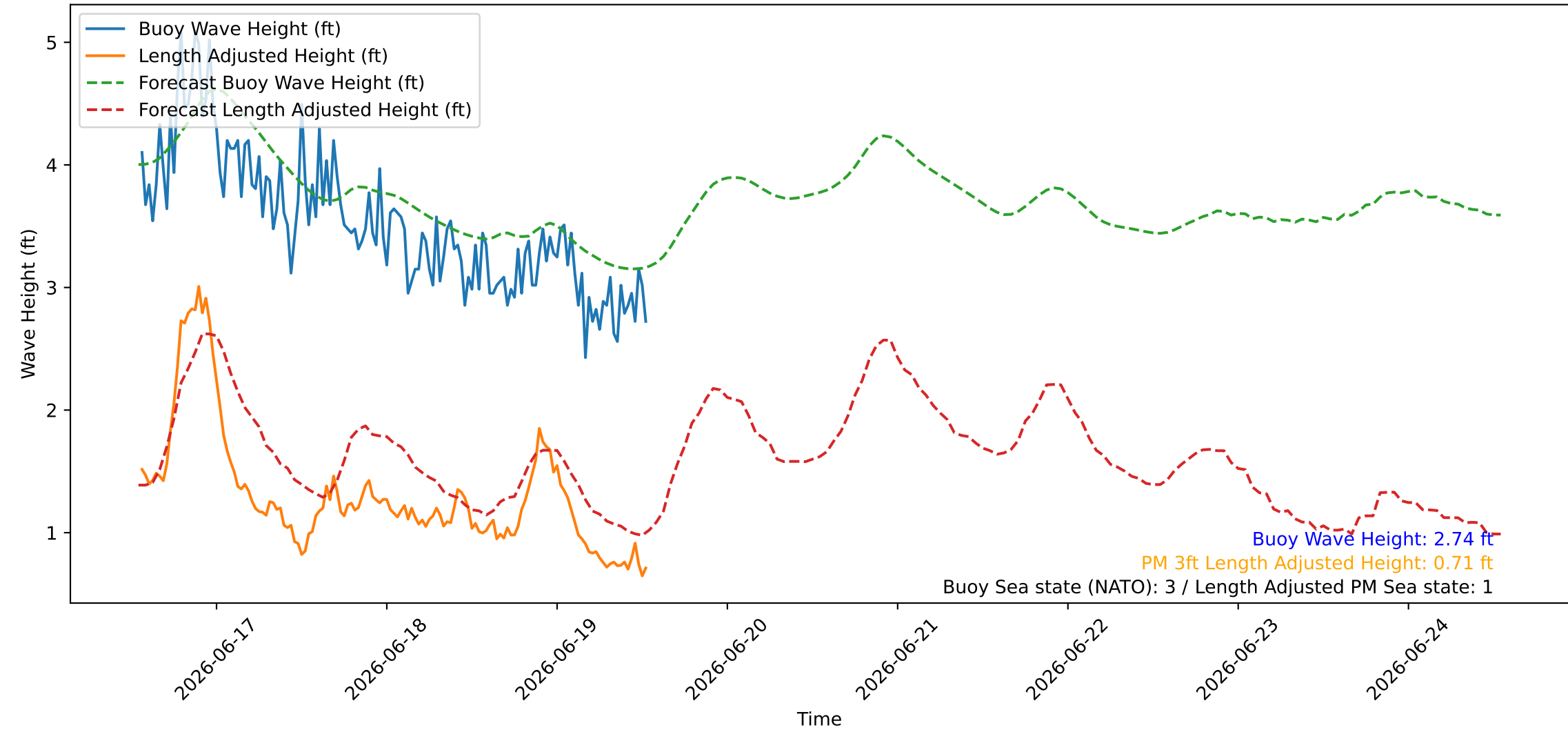
Wave Heights over Time for Green Beach at 2026-06-19 13:21:09
