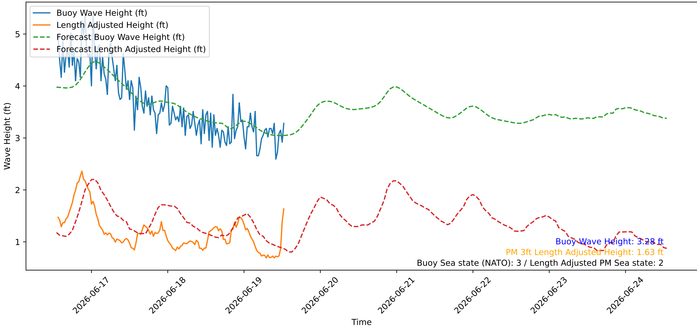
Wave Heights over Time for Red Beach at 2026-06-19 13:20:47
