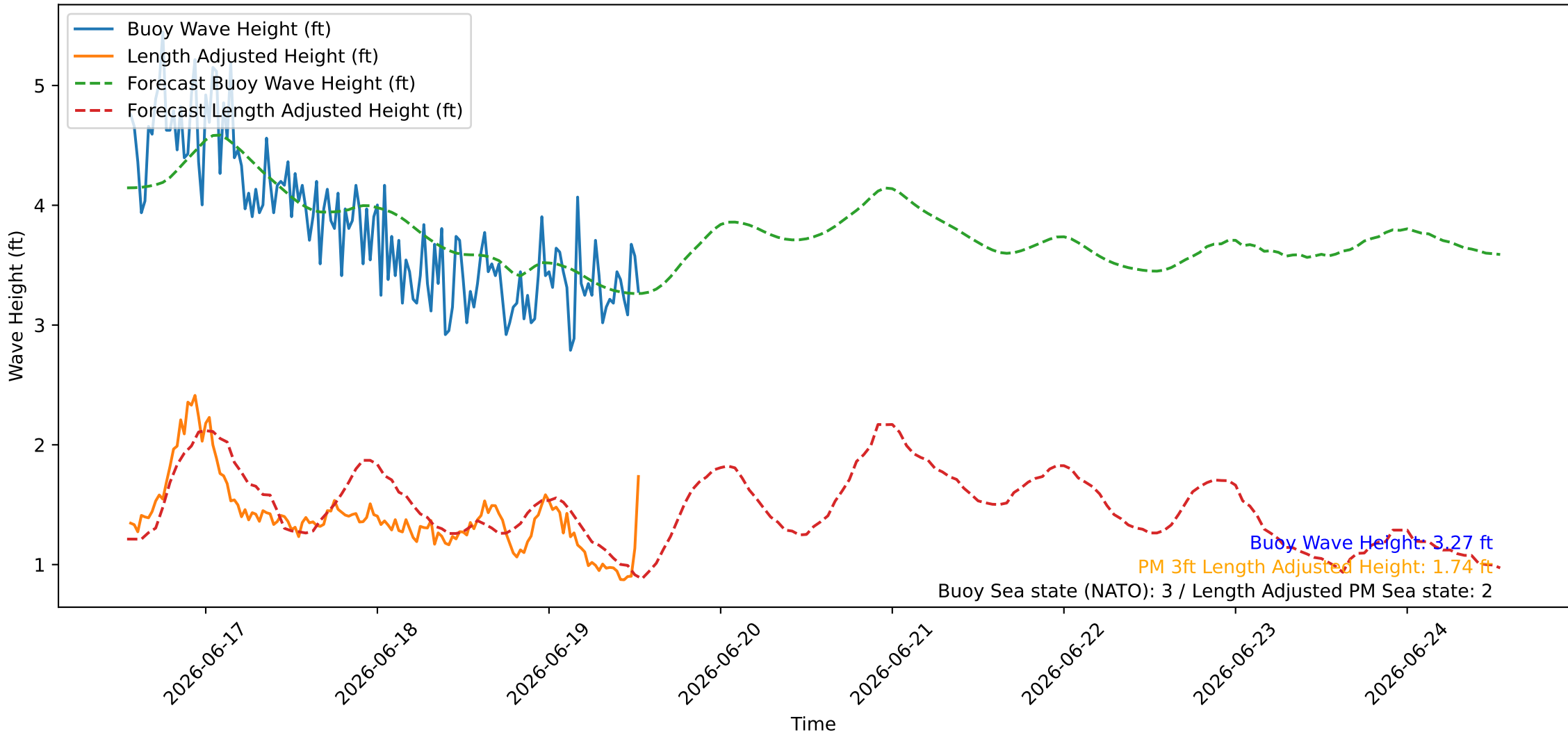
Wave Heights over Time for Oceanside Harbor at 2026-06-19 13:20:26
