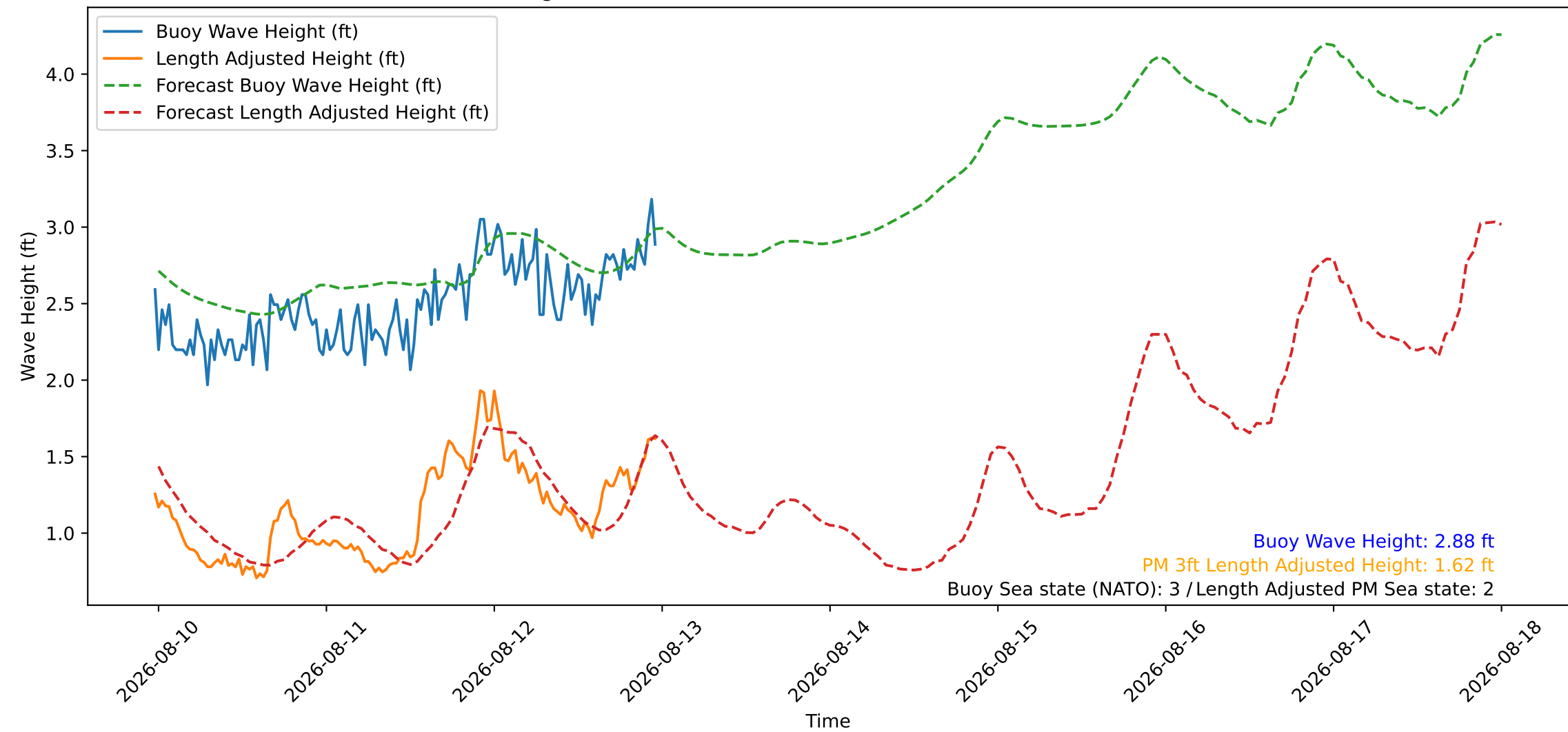
Wave Heights over Time for Oceanside Harbor at 2026-08-12 23:40:26
