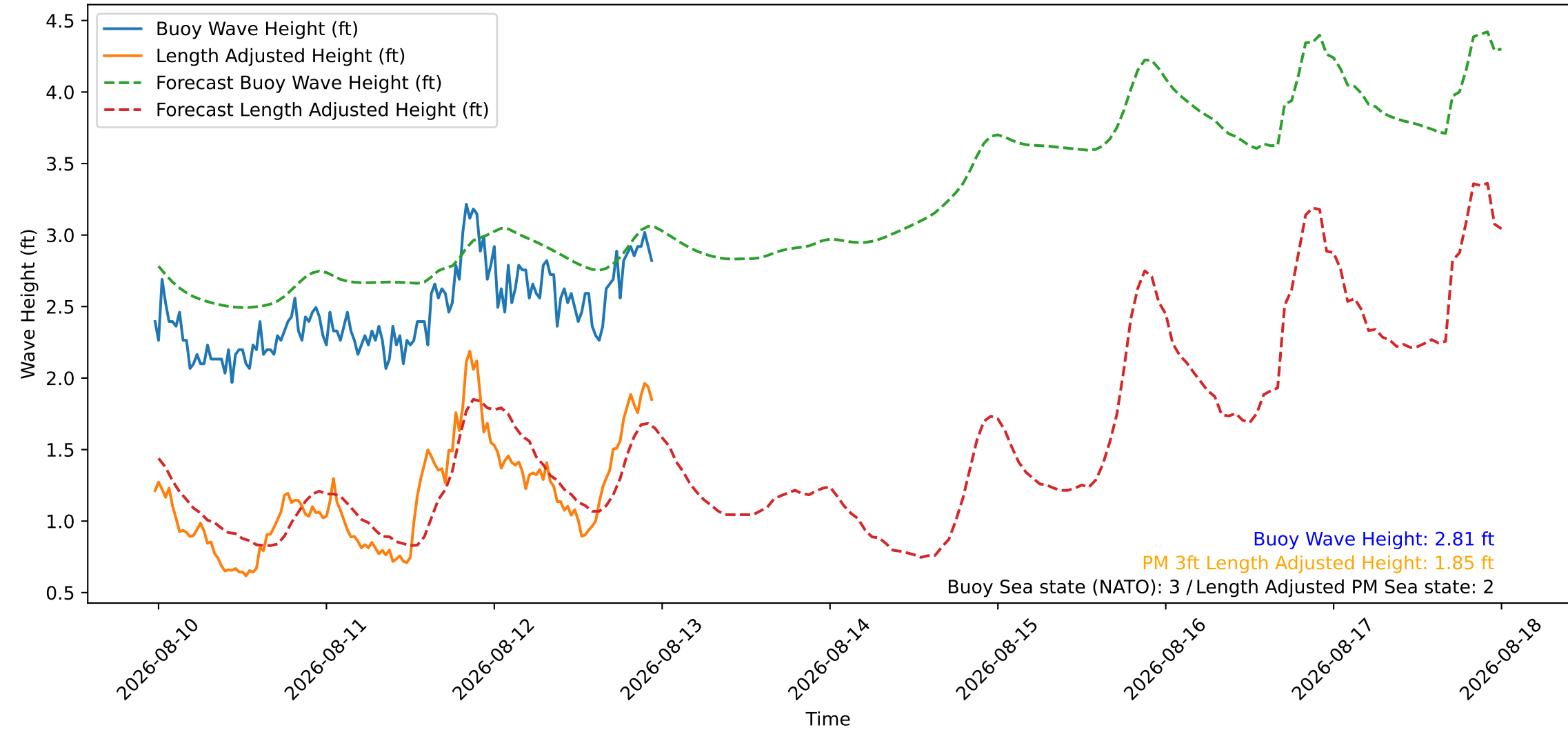
Wave Heights over Time for Green Beach at 2026-08-12 23:41:10
