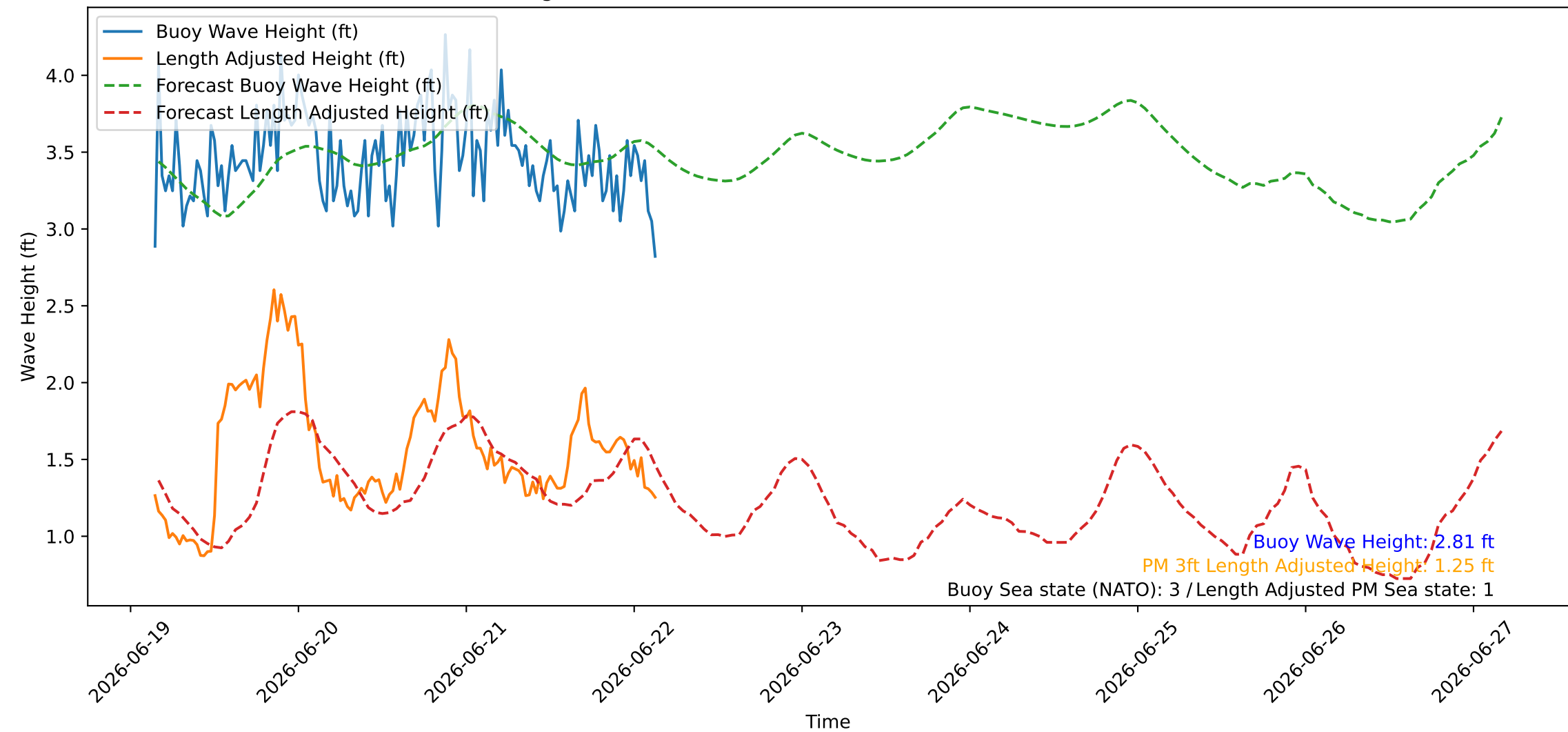
Wave Heights over Time for Oceanside Harbor at 2026-06-22 03:40:25
