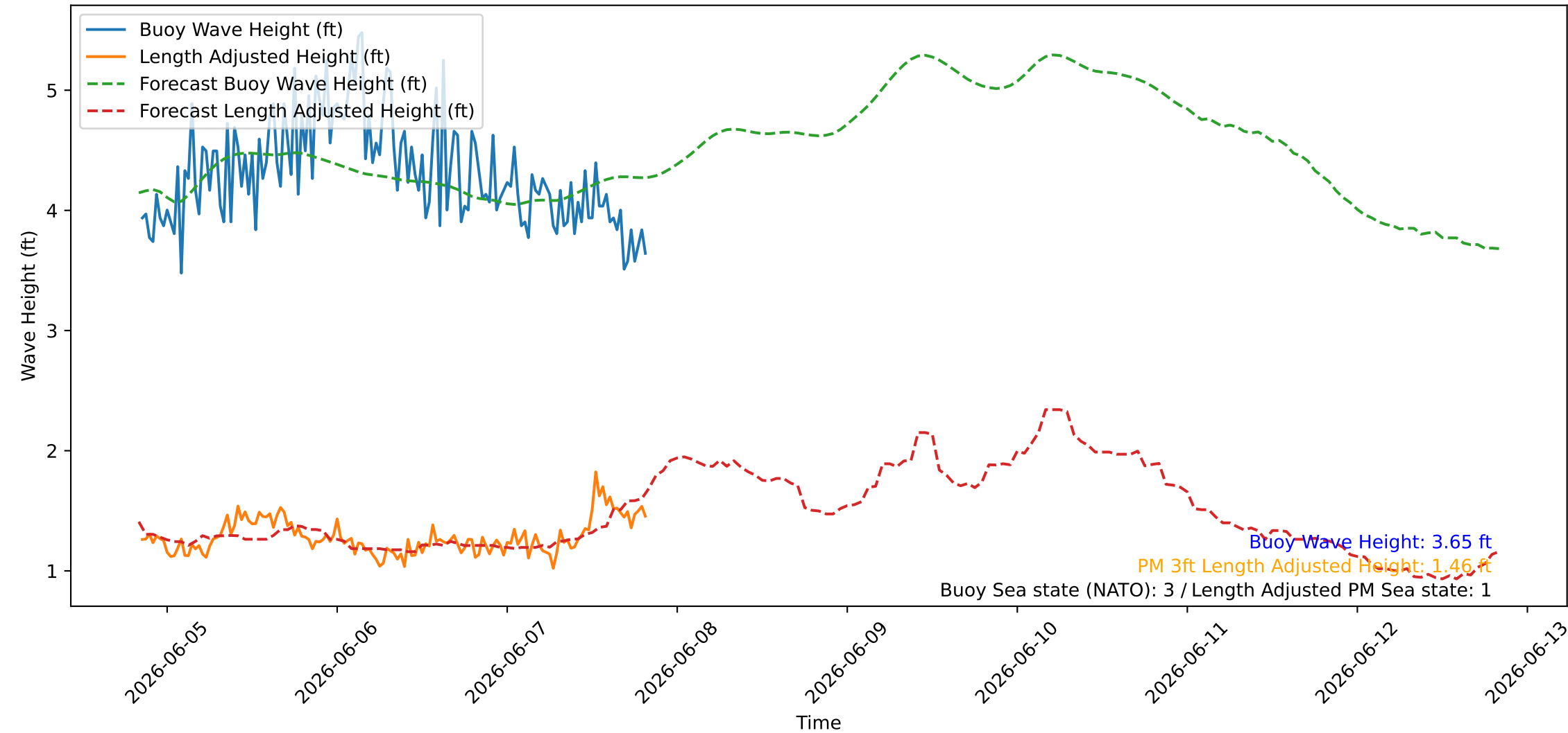
Wave Heights over Time for Oceanside Harbor at 2026-06-07 20:20:26
