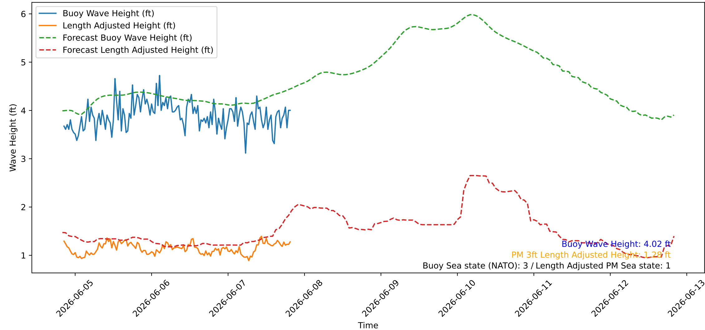
Wave Heights over Time for Green Beach at 2026-06-07 20:21:09
