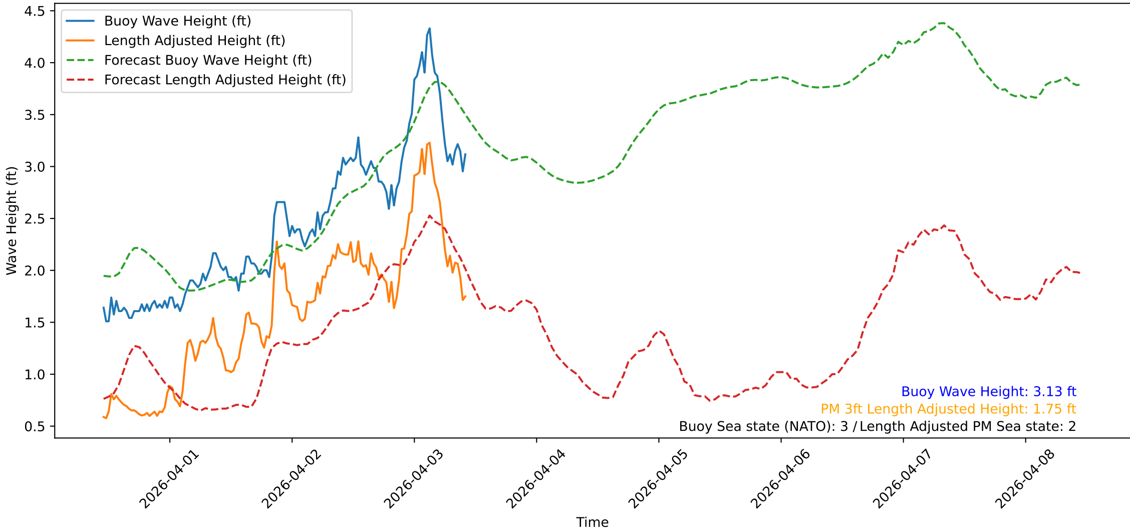
Wave Heights over Time for Green Beach at 2026-04-03 11:01:10
