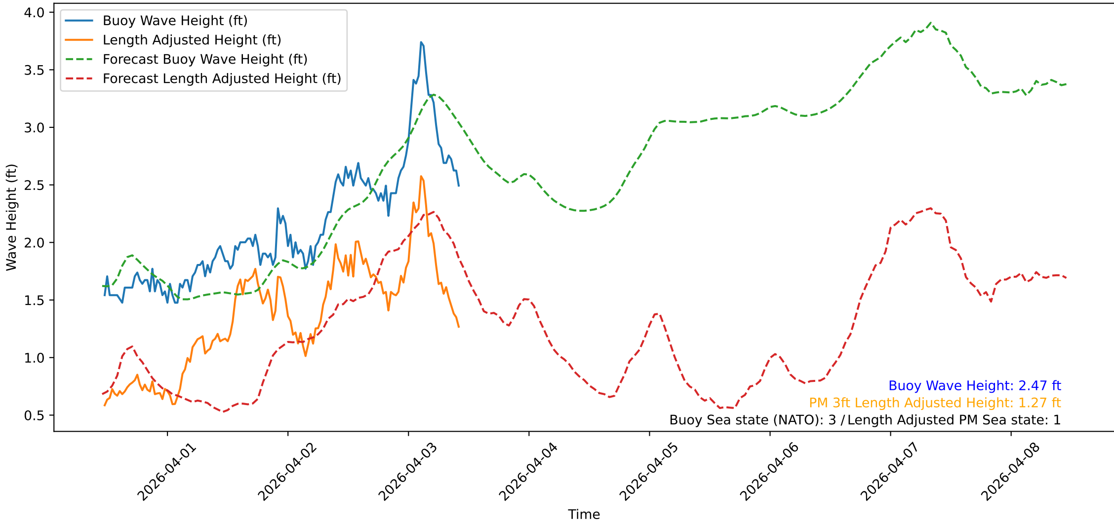
Wave Heights over Time for Red Beach at 2026-04-03 11:00:48
