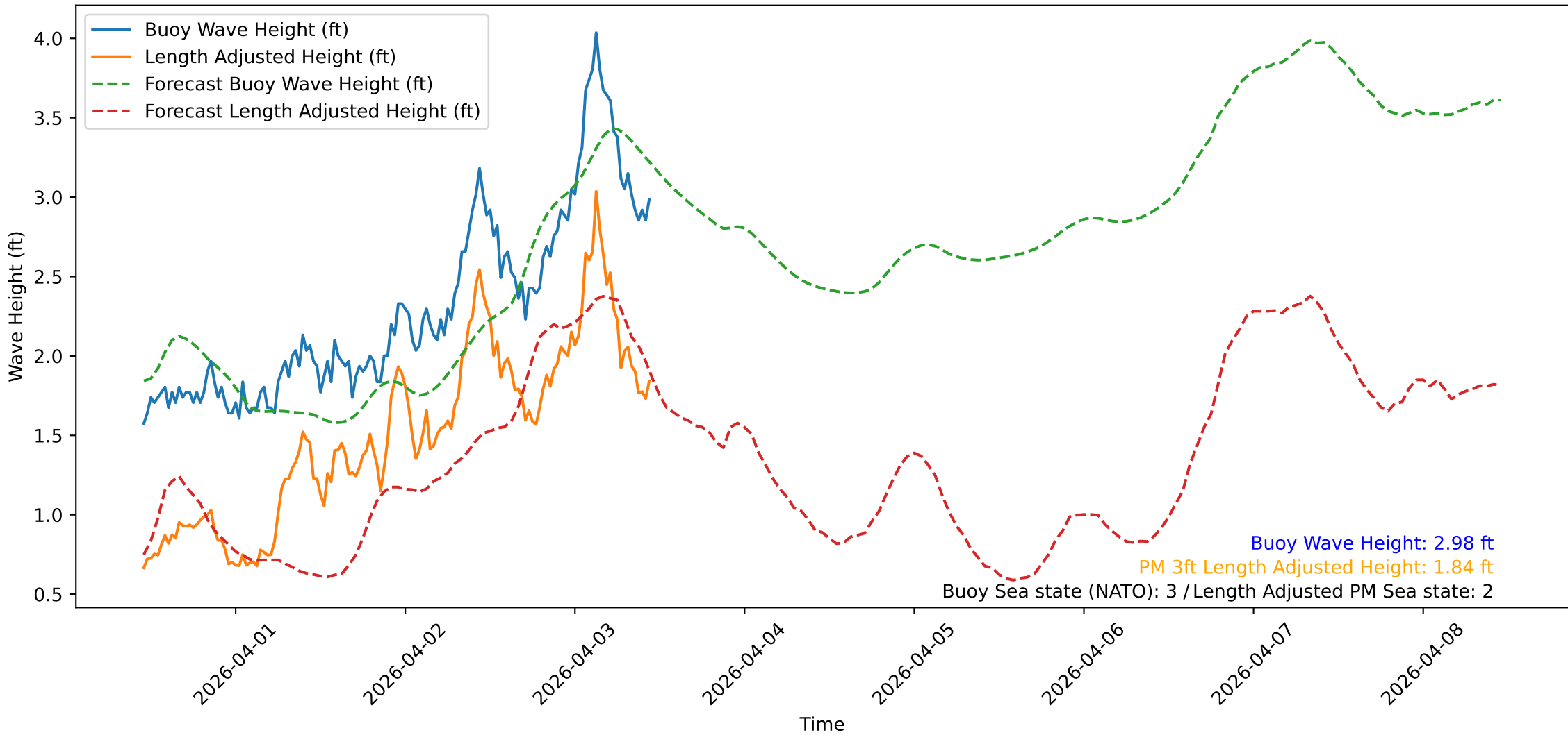
Wave Heights over Time for Oceanside Harbor at 2026-04-03 11:00:31
