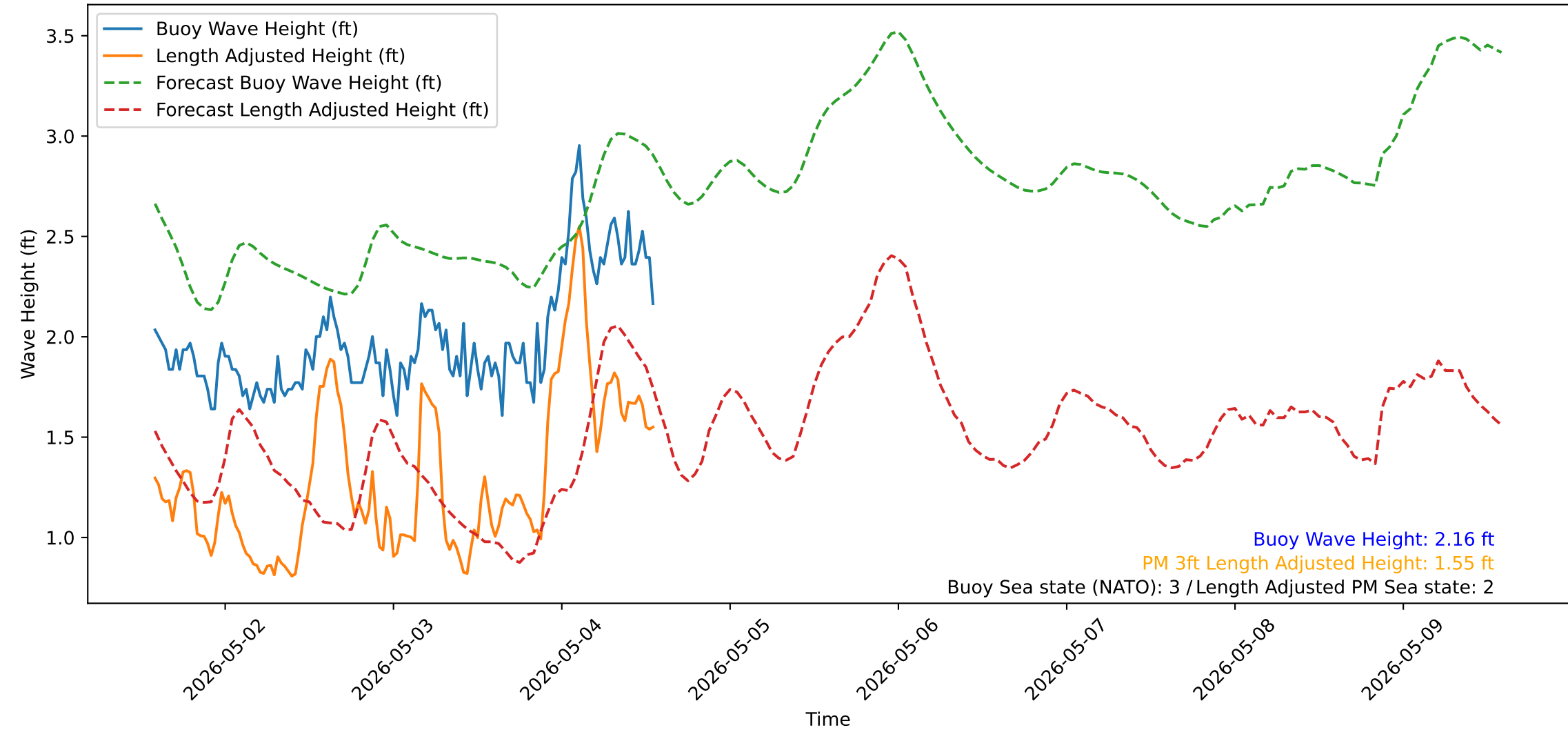
Wave Heights over Time for Red Beach at 2026-05-04 13:50:52
