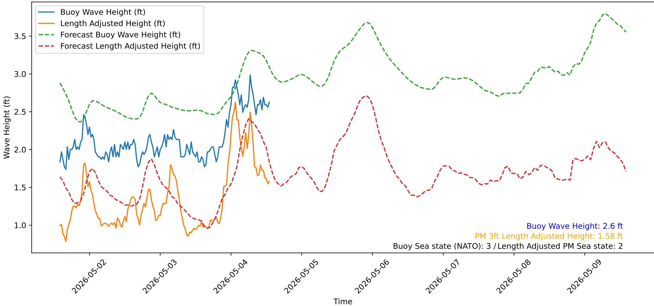
Wave Heights over Time for Green Beach at 2026-05-04 13:51:14
