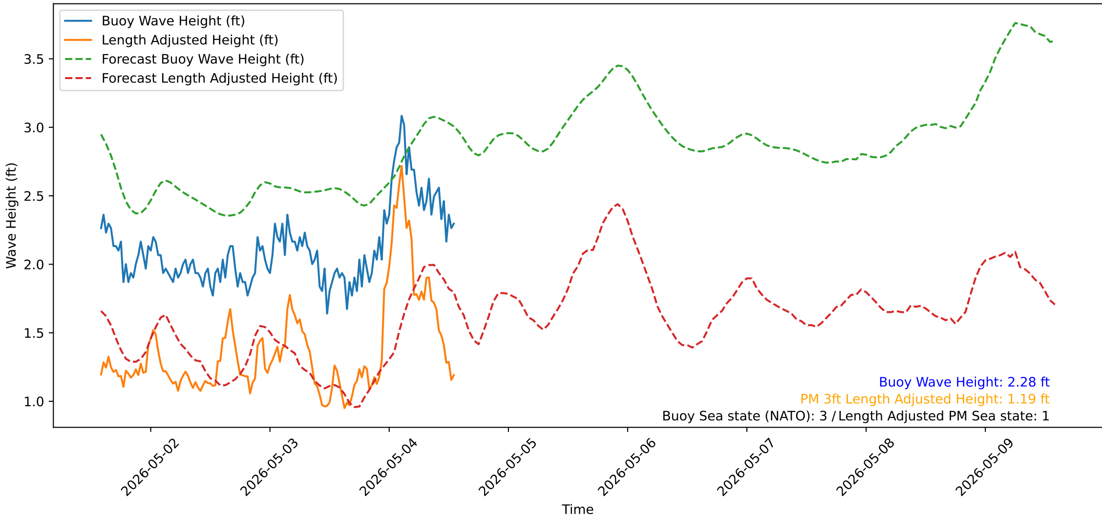
Wave Heights over Time for Oceanside Harbor at 2026-05-04 13:50:31
