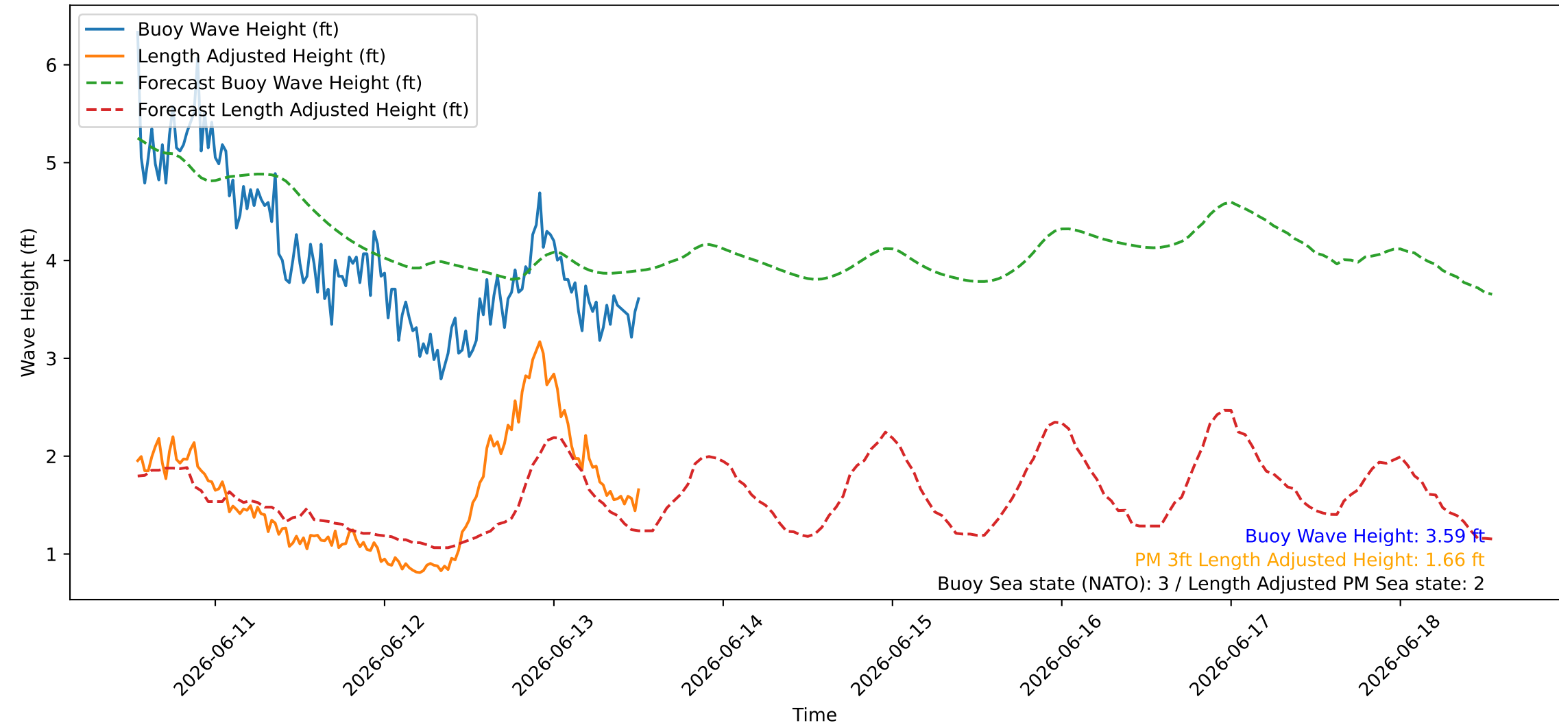
Wave Heights over Time for Oceanside Harbor at 2026-06-13 13:00:26
