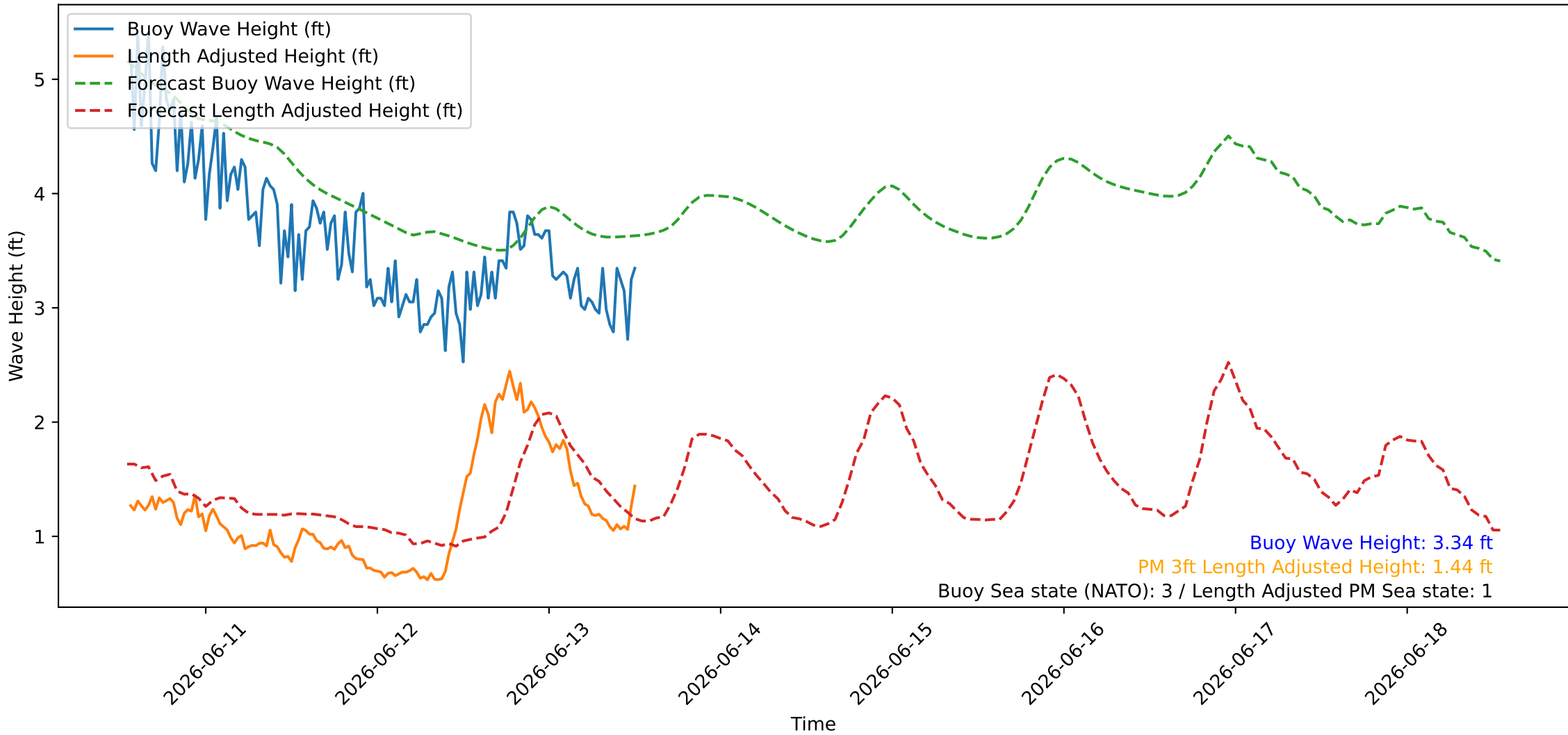
Wave Heights over Time for Red Beach at 2026-06-13 13:00:46
