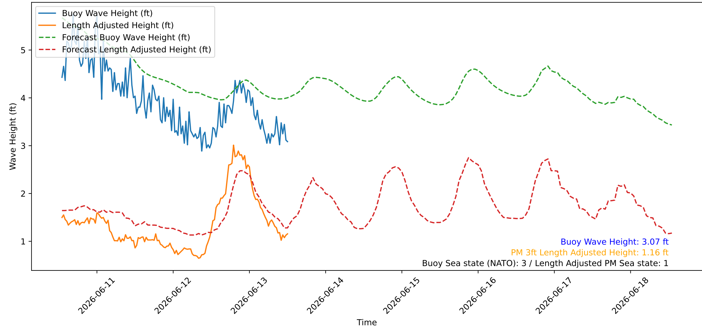
Wave Heights over Time for Green Beach at 2026-06-13 13:01:09
