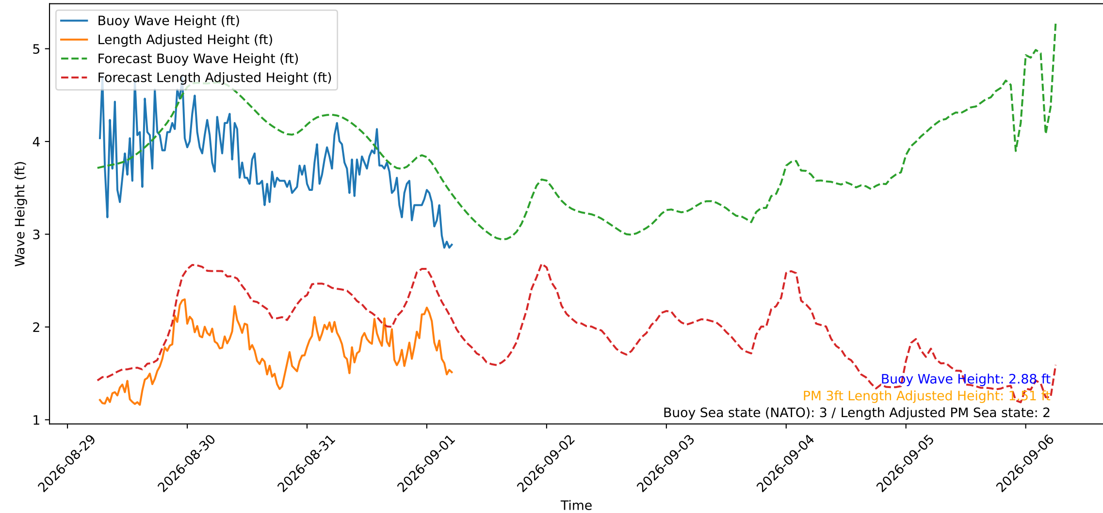
Wave Heights over Time for Red Beach at 2026-09-01 06:00:50
